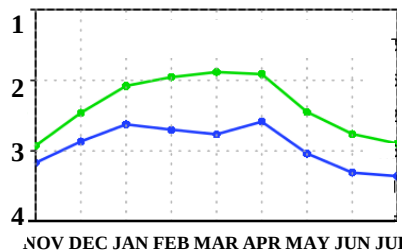
Precipitation, Trop. Pac
