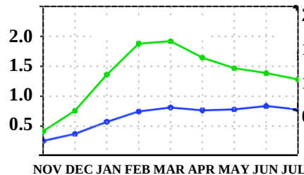
Precipitation, Trop. Pac
