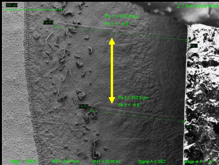
SEM image of Tin Whiskers shorting a bond pad to packaging. (example)
