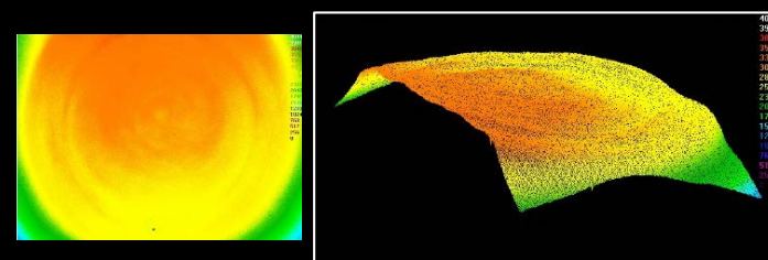
LED Beam Profile
