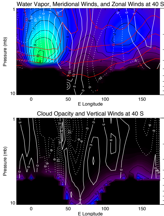
Figure 2: Top: Eastern hemisphere water vapor (color shading), meridional winds (white contours), and zonal winds (red contours) at 40^\circ S. Bottom: cloud opacity (color shading), and vertical winds (white contours) at 40^\circ S.
