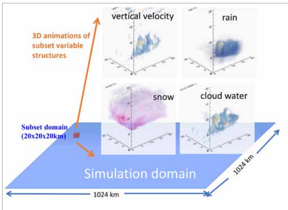
► Examples of dynamical subsetting of the convective core and associated rain, snow, and cloud water mixing ratio over a 3D box of 20 x 20 x 20 km (there are a total of two billion grid points in the whole 3D domain).
