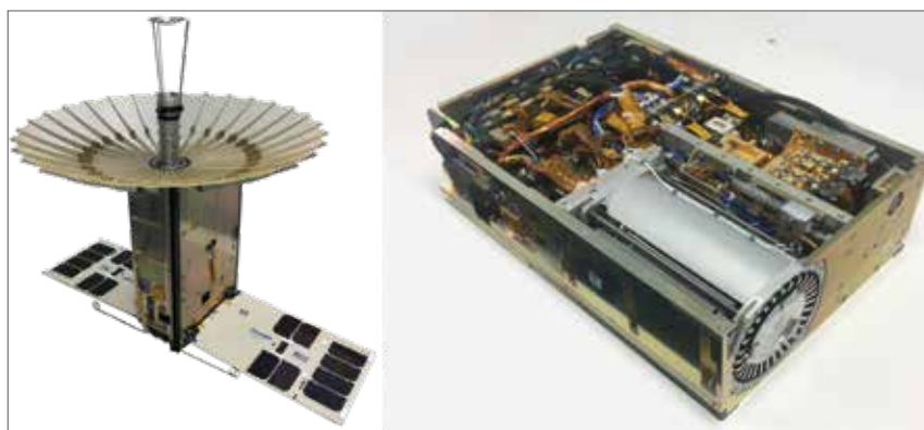
► RainCube CubeSat flight hardware (deployed on left, stowed on right). Tyvak, Inc was responsible for the bus delivery and flight integration and performed mission operations. NASA JPL developed the radar instrument and was responsible for system engineering and project management. (Credit: NASA JPL)
