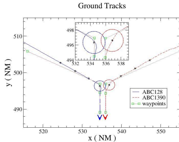
Figure 8. Ground tracks for two aircraft making visual approaches to the finals from opposite sides of the runways.
