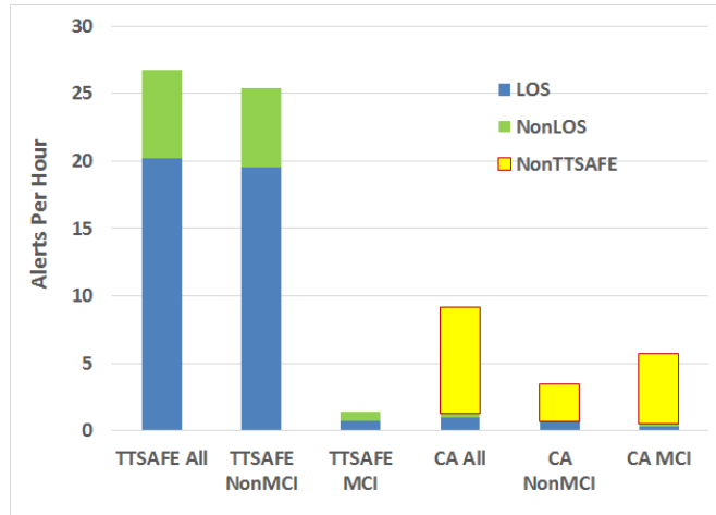
Figure 6. T-TSAFE and STARS CA alerts in terms of LOS, non-LOS, and non-TTSAFE alerts with common conflict pairs shown on the CA bars.
