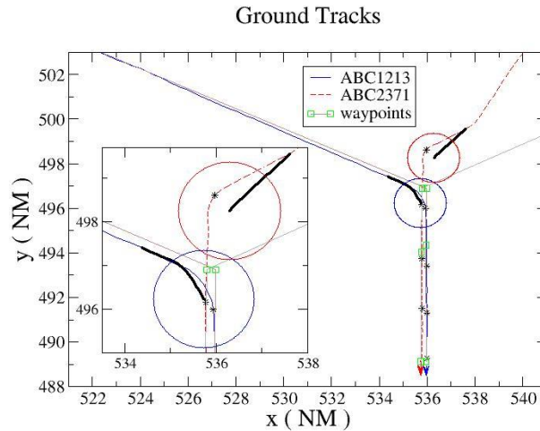
Figure 17. Ground tracks for an arrival pair making visual final approaches to two parallel runways less than 2500 ft apart from opposite sides with track crossing.
