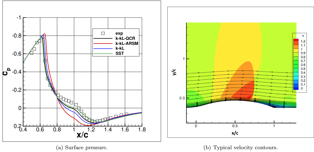
Figure 17. Axisymmetric Transonic Bump: Comparison of two-equation turbulence model results.
