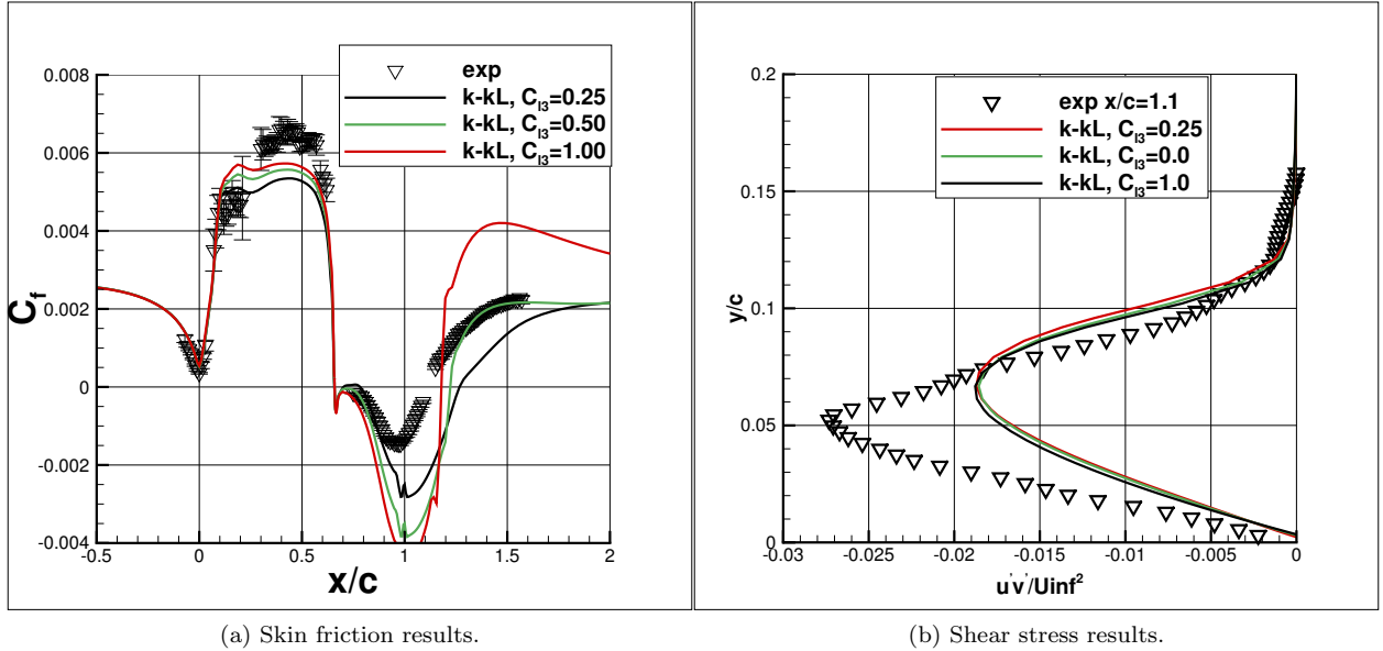
Figure 12. Wall-Mounted Hump: calibration of k-kL turbulence model.
