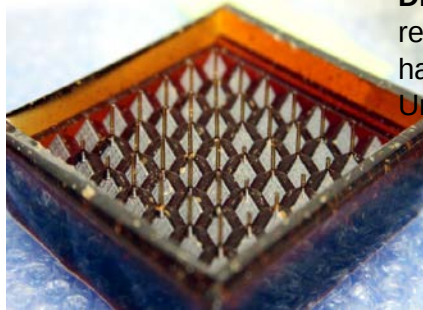
Figure 2 Tortuosity substrates produced with waveguide sheets
