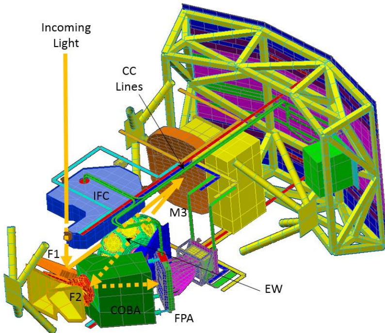
Figure 1. WFI MCR Design: Major internal components of the WFI include fold mirror 1 (F1), tertiary mirror (M3), element wheel (EW), actuated fold mirror 2 (F2), and the Focal Plane Array (FPA). The Cold Optics Baffle Assembly provides a cold scene for the detectors. A secondary Integrating Field Channel provides simultaneous spectroscopic measurements
