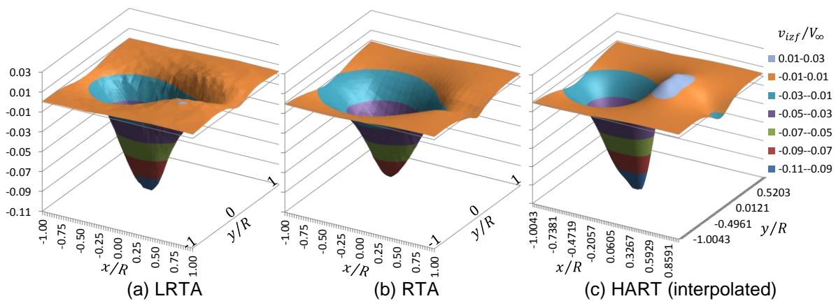
Fig. 4: Fuselage-induced velocity distribution, \alpha = -20^\circ , z/R = 0.1 .
