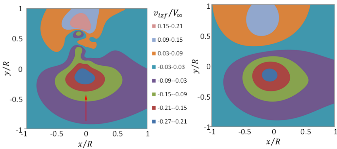
(c) \beta = 90^\circ : CFD data (left), model (right)
