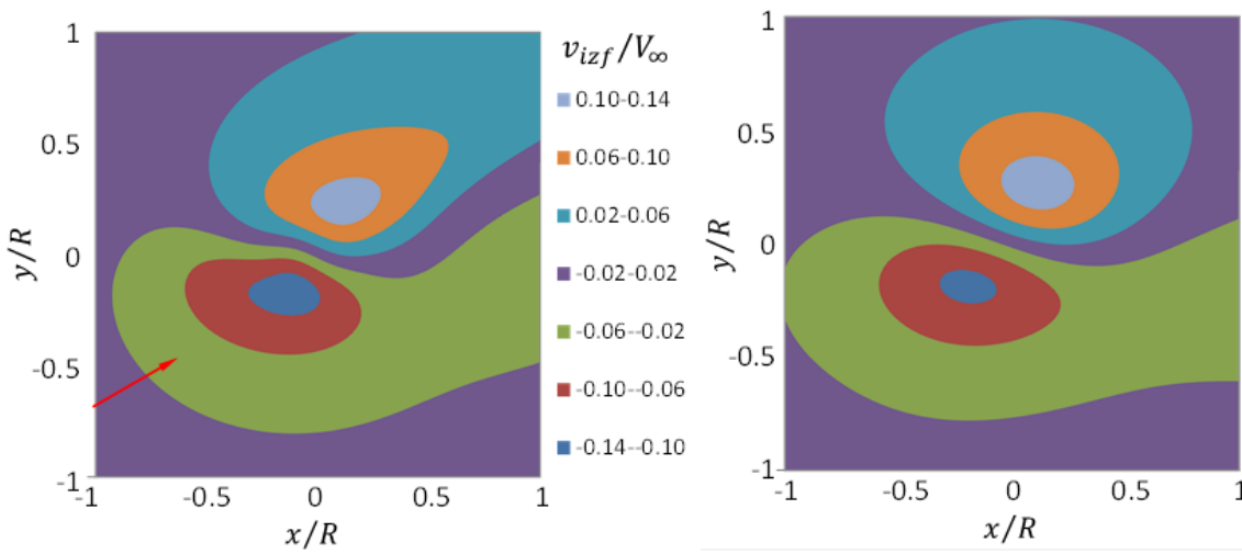
(b) \beta = 30^\circ : CFD data (left), model (right)
