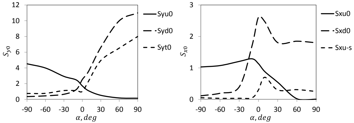
Fig. 10: Dependence of shape factors on \alpha ; \beta = 0^\circ .
