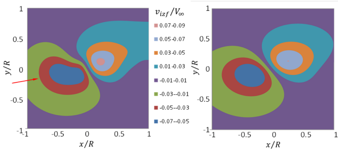
(a) \beta = 10^\circ : CFD data (left), model (right)
