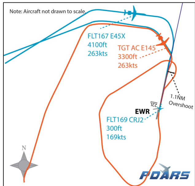
Figure 9 Go-Around with ERC Overshoot Scenario.
