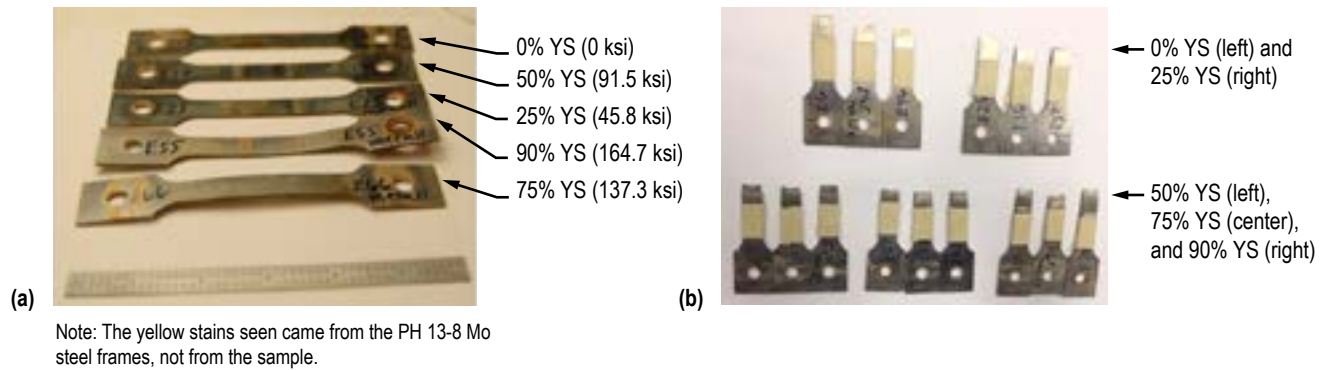
Figure 15. Samples exposed to 3.5% NaCl alternate immersion for 365 days and subjected to post-test evaluations: (a) Used for metallographic analysis and (b) tensile tested.
