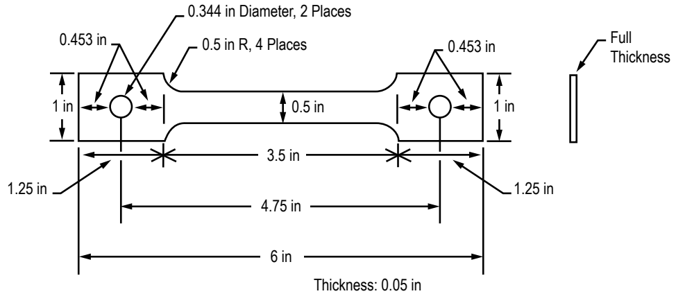
Figure 1. Drawing of stress corrosion specimen.
