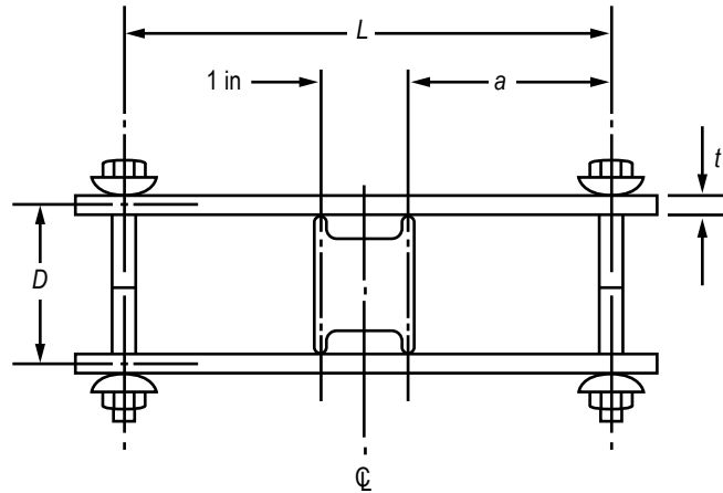
Figure 4. Double-beam assembly.
