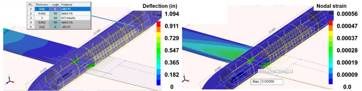
Figure 10. Tempest FEM analysis with M-SHELLS composite panel fuselage floor.
