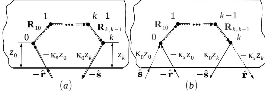
Figure 7: Scattering by the particles chain \{\mathbf{R}_{0:k}\} illuminated by (a) the same plane electromagnetic wave propagating in the direction -\hat{\mathbf{r}} , and (b) two plane electromagnetic wave propagating in the directions -\hat{\mathbf{r}} and \hat{\mathbf{s}} .
