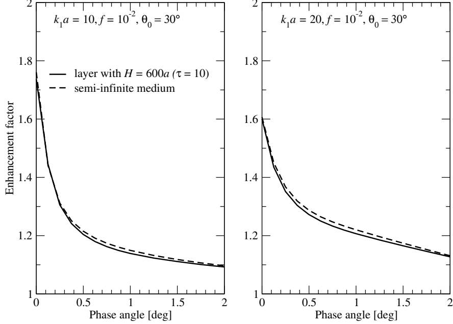
Figure 4: Enhancement factor versus the phase angle for a discrete random layer and a semi-infinite discrete random medium. For the volume concentration f = 10^{-2} , the relative error in \kappa is \varepsilon_\kappa = 1.2 \times 10^{-2} . The computational parameters are indicated in the plots.
