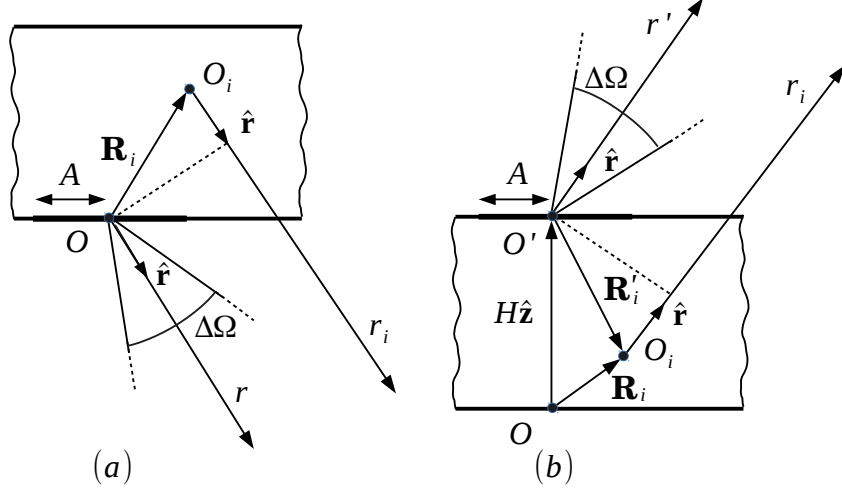
Figure 1: Geometries for defining (a) the reflection and (b) the transmission matrices.
