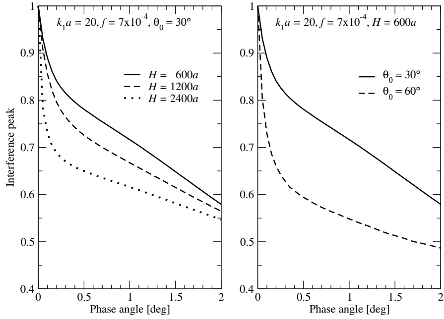
Figure 3: Left: interference peak versus the phase angle for three value of the layer thickness: H = 600a ( \tau \approx 0.7 ), 1200a ( \tau \approx 1.4 ), and 2400a ( \tau \approx 2.8 ). Right: interference peak versus the phase angle for two values of the incidence angle: \theta_0 = 30^\circ and 60^\circ . The parameters of the calculations are indicated in the plots.
