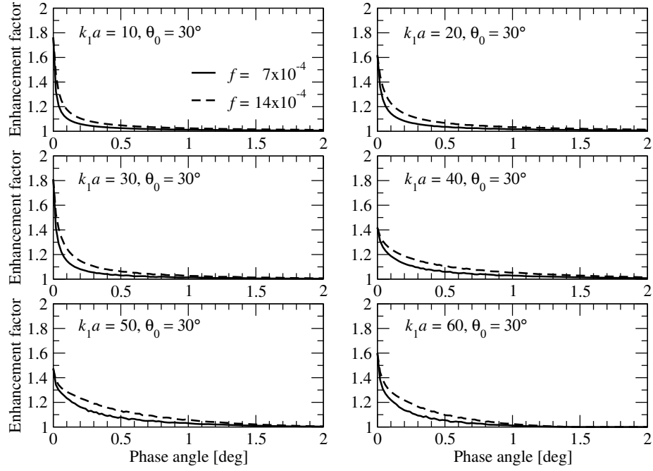
Figure 5: Enhancement factor versus the phase angle for two values of the volume concentration: f = 7 \times 10^{-4} and 14 \times 10^{-4} . The number of discrete ordinates per hemisphere N_\mu (see Appendix 4) is 16 for k_1a = 10 , 24 for k_1a = 20 , 32 for k_1a = 30 , 36 for k_1a = 40 , 42 for k_1a = 50 , and 48 for k_1a = 60 . The computational parameters are indicated in the plots.
