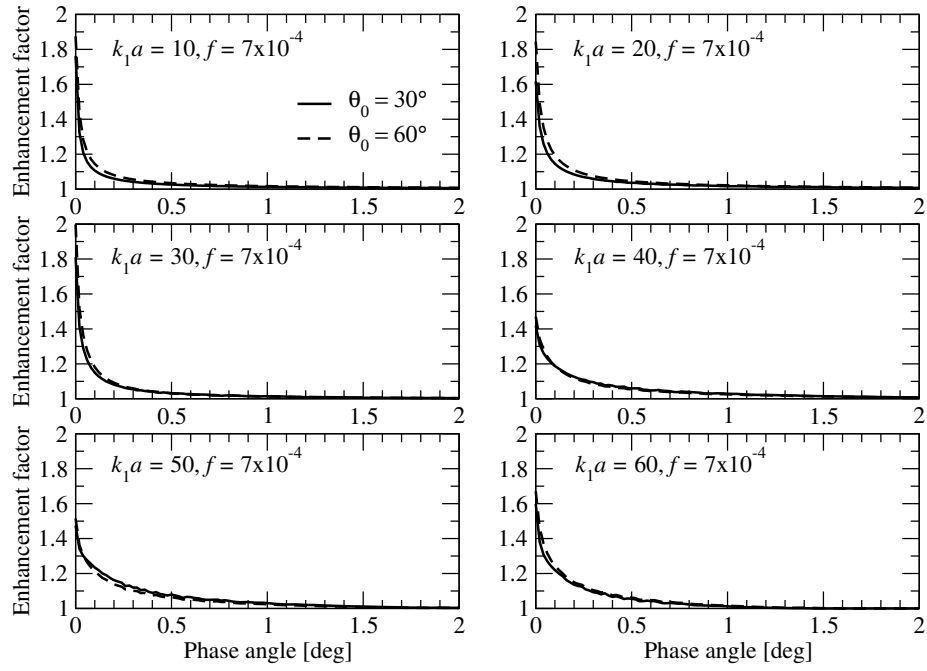
Figure 6: Enhancement factor versus the phase angle for two values of the incidence angle: \theta_0 = 30^\circ and 60^\circ . The computational parameters are indicated in the plots.
