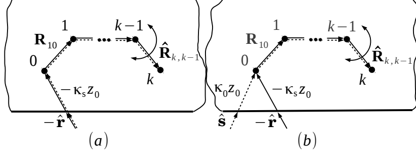
Figure 8: Scattering geometries for constructing the probability density functions (a) p_L(\Theta, \Phi) and (b) p_C(\Theta, \Phi) .
