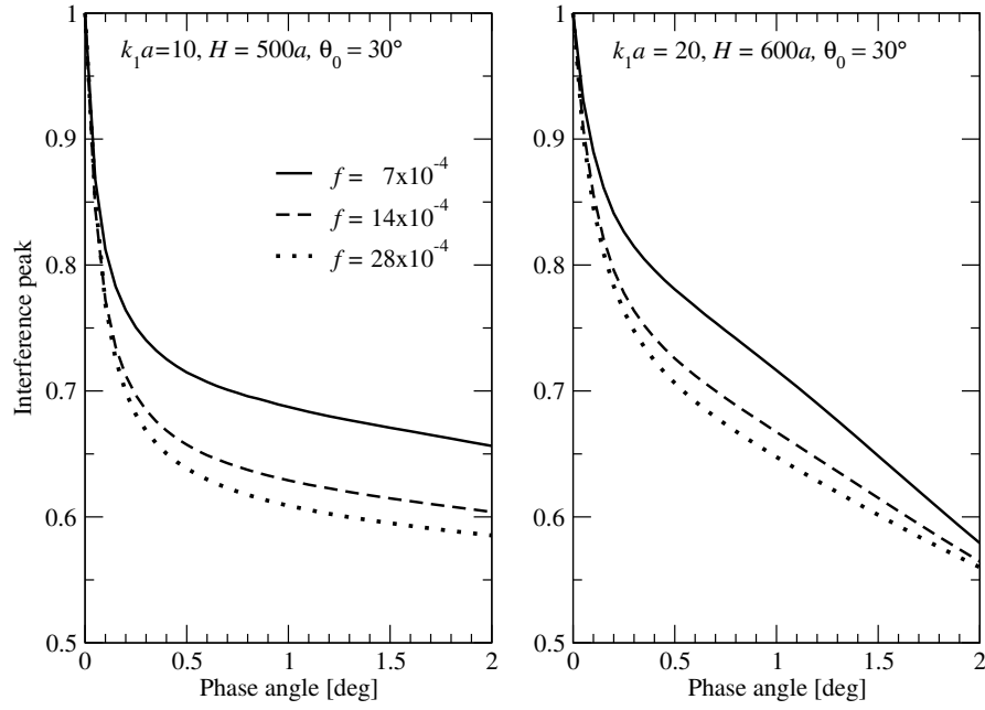
Figure 2: Interference peak versus the phase angle for three values of the volume concentration: f = 7 \times 10^{-4} , 14 \times 10^{-4} , and 28 \times 10^{-4} . For these values of the volume concentration, the relative errors in \kappa are \varepsilon_\kappa = 9 \times 10^{-4} , 1.8 \times 10^{-3} , and 3.6 \times 10^{-3} , respectively. The parameters of the calculations are indicated in the plots.
