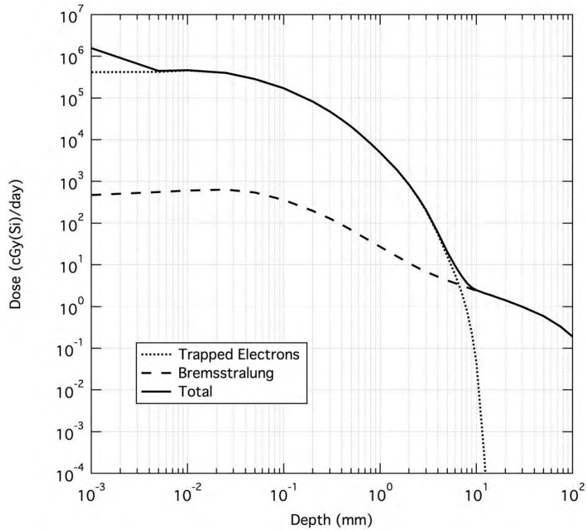
Figure 3.3.1.3-2. Daily Trapped Belts TID Inside Shielding
