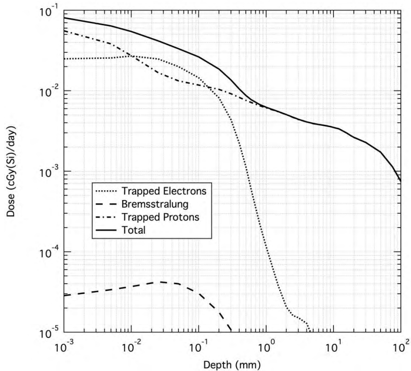
Figure 3.3.1.2.3-3. Daily Trapped Belts TID Inside Shielding
