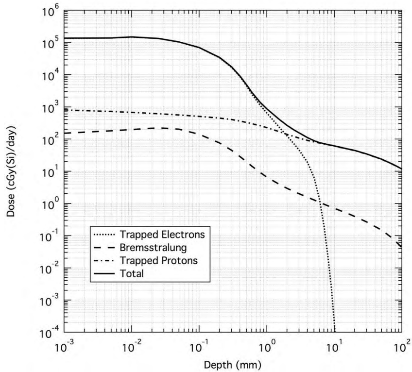
Figure 3.3.1.2.1-3. Daily Trapped Belts TID Inside Shielding
