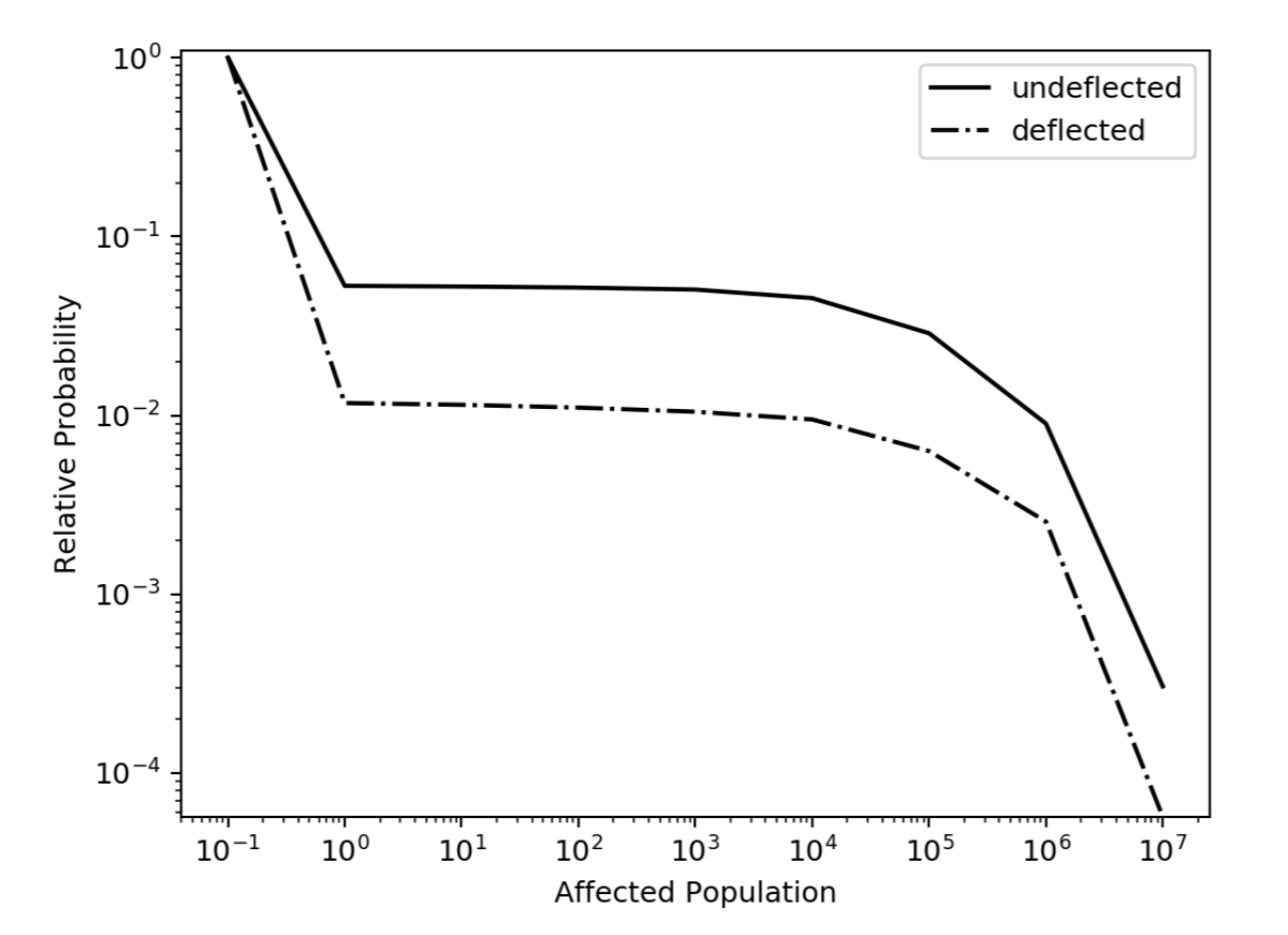
Figure 6: Damage exceedance plot for deflected and undeflected scenario. Shows probability of incurring the inquired damage level or less. The deflected case reduces the damage probability consistently.
