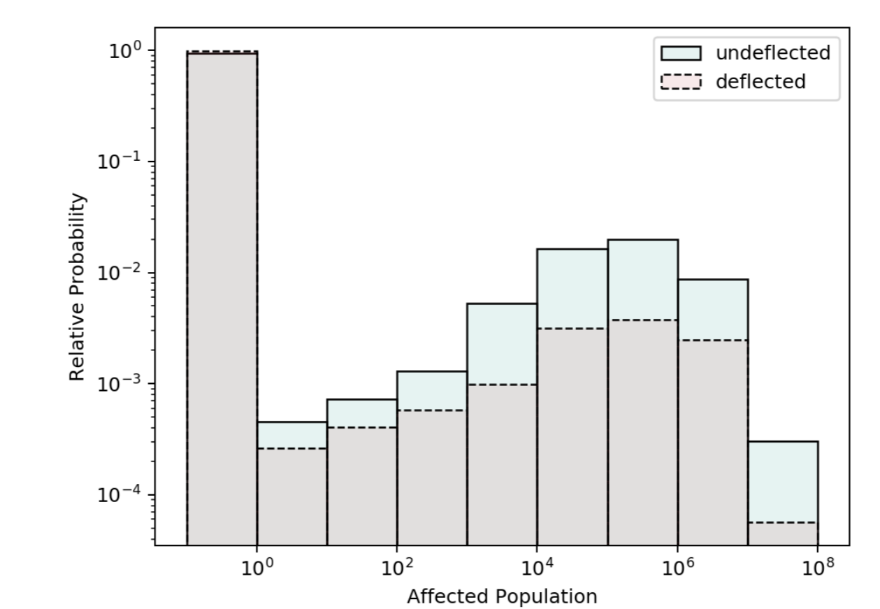
Figure 5: Affected population histogram for the undeflected and deflected impact scenario. Values <1 equate to zero casualties and largely represent samples that miss the Earth entirely. The deflection mission reduces the affected population in each bin and increases the asteroid's Earth miss probability.
