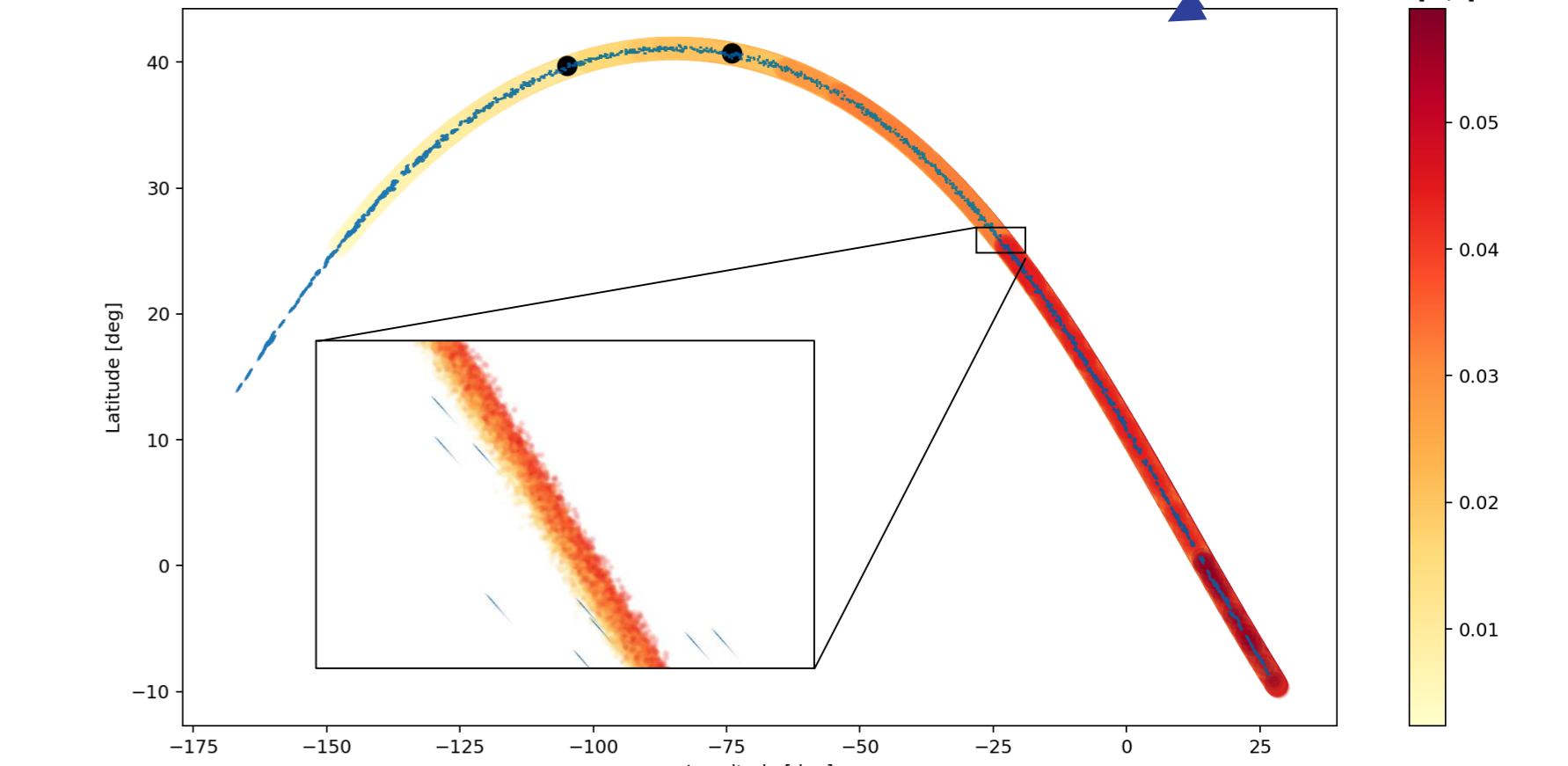
Figure 4: Impact corridor plot. The undeflected corridor is shown in blue points. The yellow/red shaded regions show impact points (see inset) of deflected orbits. The deflected impact points are colored with the applied deflection DV. A larger deflection DV moves the corridor eastwards.
