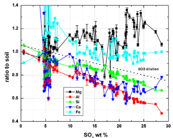
Figure 3: Major element content vs S
