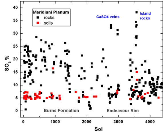
Figure 2: S vs sol number (traverse)
