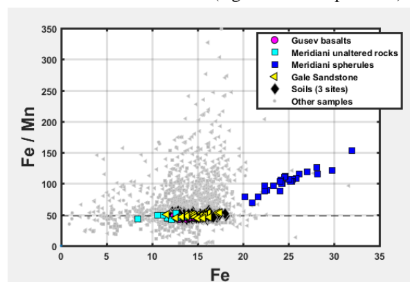
Fig. 2. Molar Fe/Mn ratio versus Fe. Samples along the dashed line maintain an unaltered Fe/Mn ratio.
