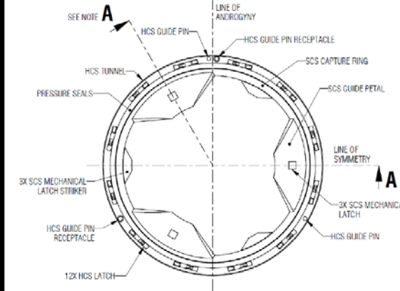
FIGURE 3.1.1.1-1 ANDROGYNOUS DOCKING INTERFACE – AXIAL VIEW
