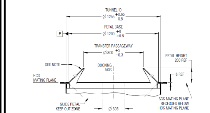
FIGURE 3.1.1.1-2 SECTION A-A (CROSS-SECTION THROUGH MID-PLANE OF TWO PETALS)
