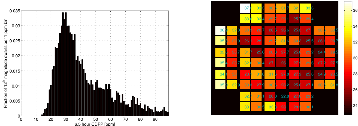
Figure 8: Combined differential photometric precision at 6.5 hours from Quarter-3 for all dwarf stars with 11.5 < \text{Kepler Mag} \leq 12.5 : (a) histogram of the distribution, left panel, and (b) the 25 th percentile of the distribution on each detector channel. The 12 th magnitude CDPP requirement is 20 ppm at 6.5 hours. Dwarf stars were selected using a surface gravity cutoff since sub-giants and giants are significantly more variable and thus their noise would be dominated by stellar variability. Approximately 10% of the 12 th magnitude dwarfs are noisier than 100 ppm. The 25 th percentile was used as an empirically determined proxy for the mode of the distribution.
