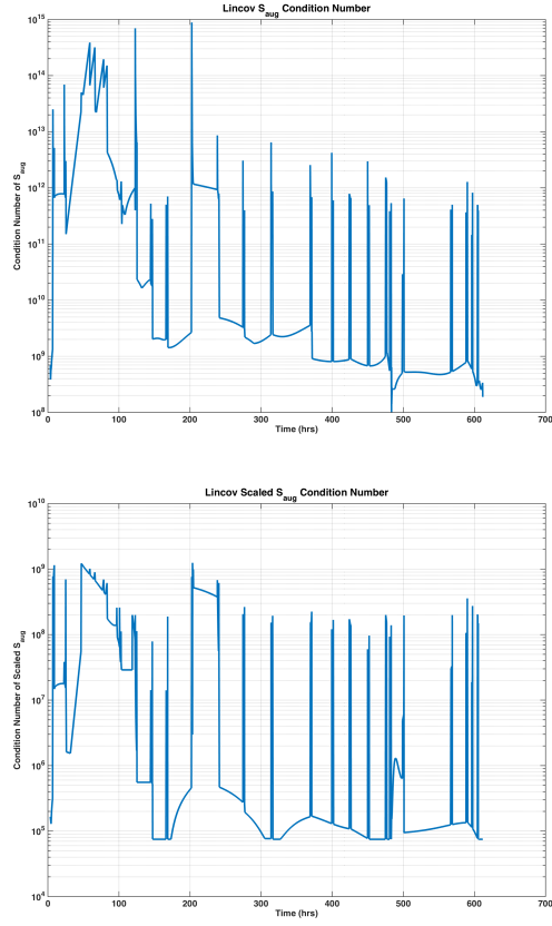
Figure 3. Condition Number for Unscaled and Scaled S_{aug}
