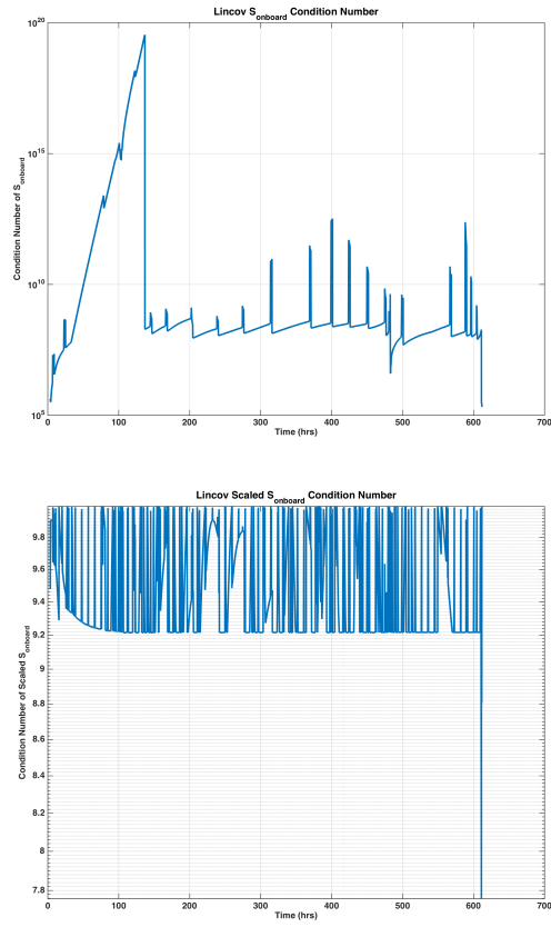
Figure 4. Condition Number for Unscaled and Scaled S_{onboard}
