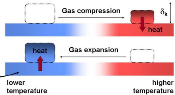
Illustration of the hydrodynamic energy transfer up the temperature gradient (heat pump, refrigerator)
