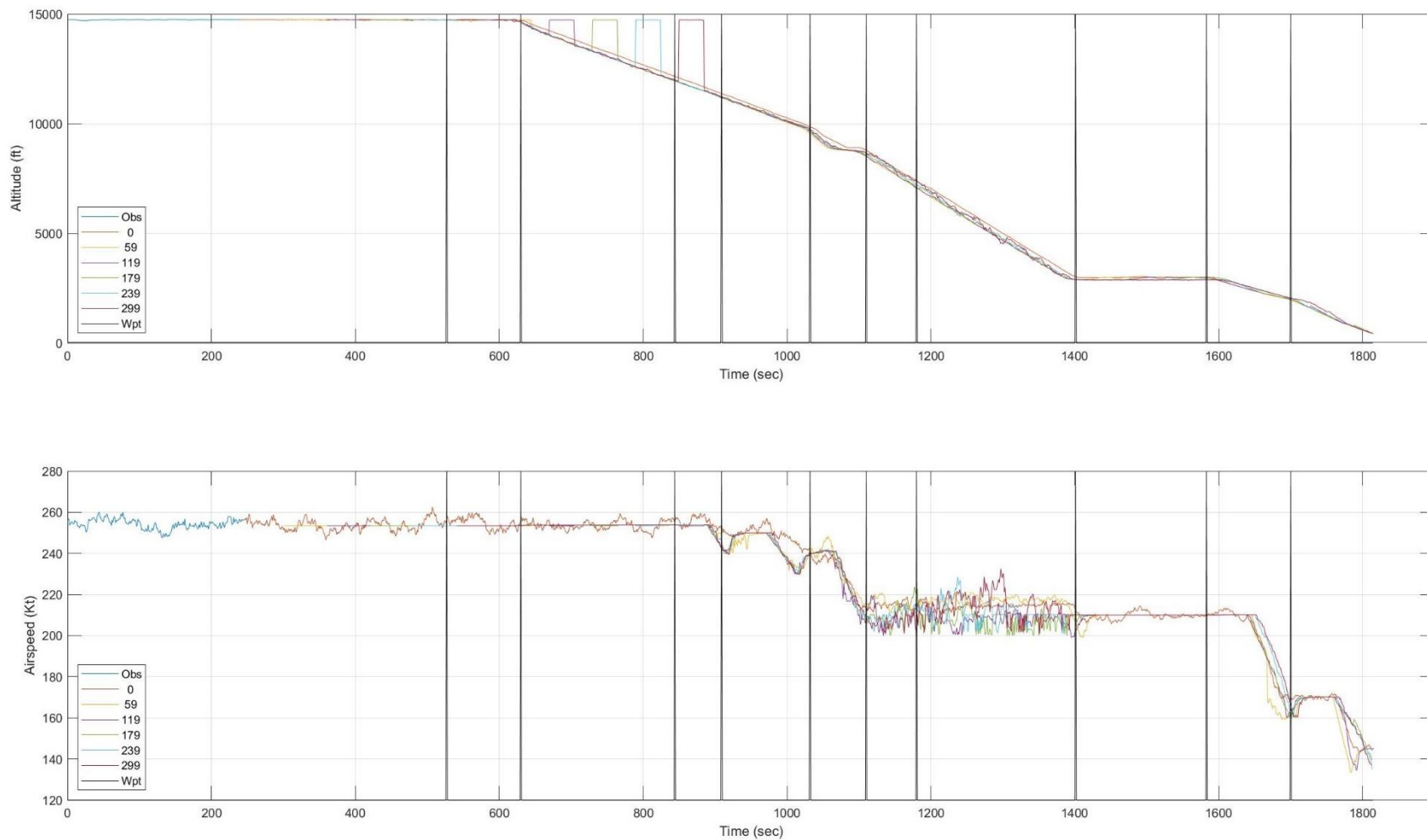
Figure E. 10: Test Flight 11: Observed and Predicted Altitude and Airspeed as a Function of Time t
