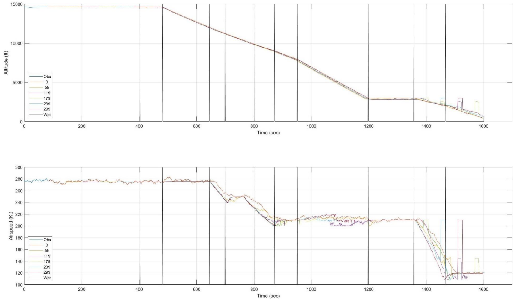
Figure E. 2: Test Flight 3: Observed and Predicted Altitude and Airspeed as a Function of Time t
