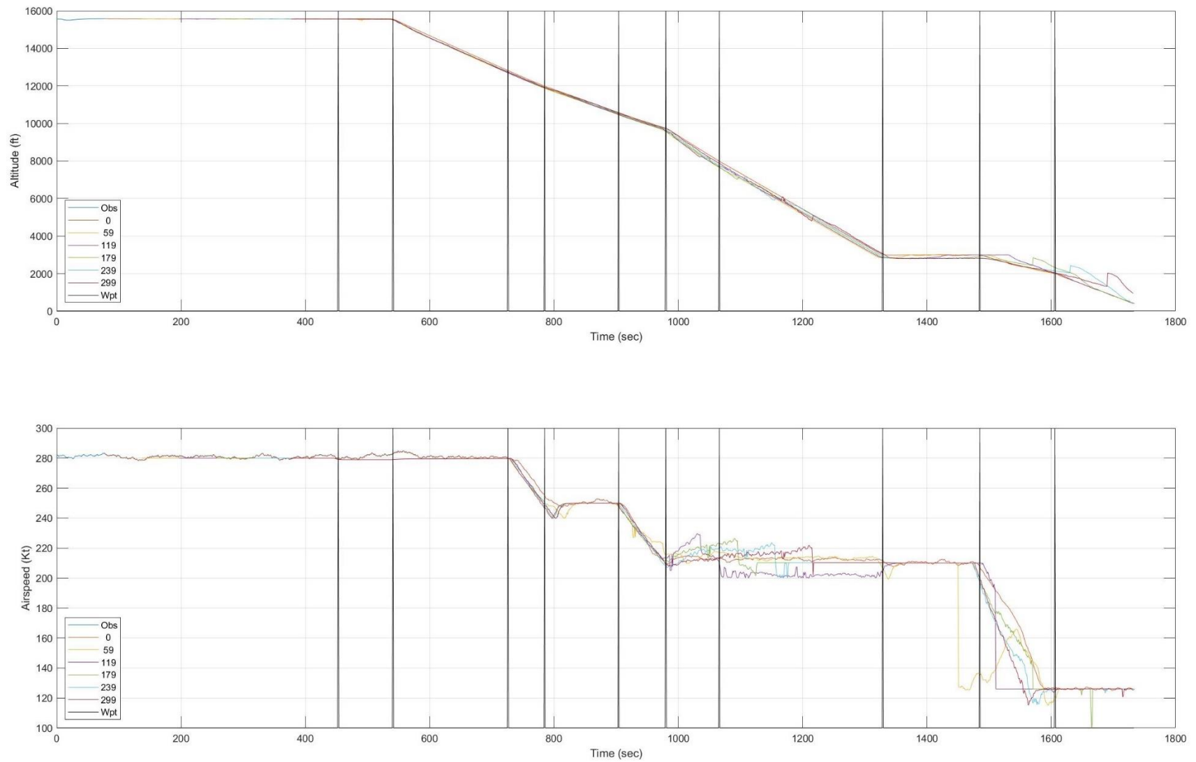
Figure E. 46: Test Flight 95: Observed and Predicted Altitude and Airspeed as a Function of Time t
