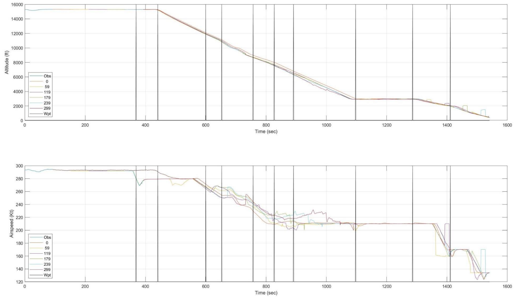
Figure E. 14: Test Flight 16: Observed and Predicted Altitude and Airspeed as a Function of Time t
