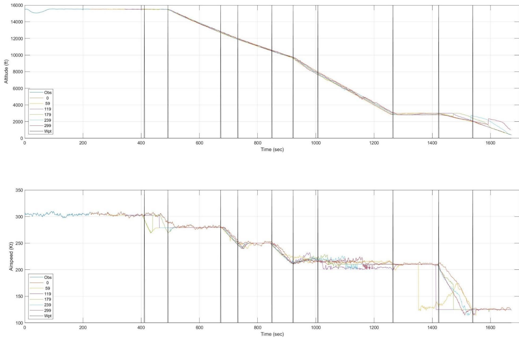
Figure E. 34: Test Flight 79: Observed and Predicted Altitude and Airspeed as a Function of Time t
