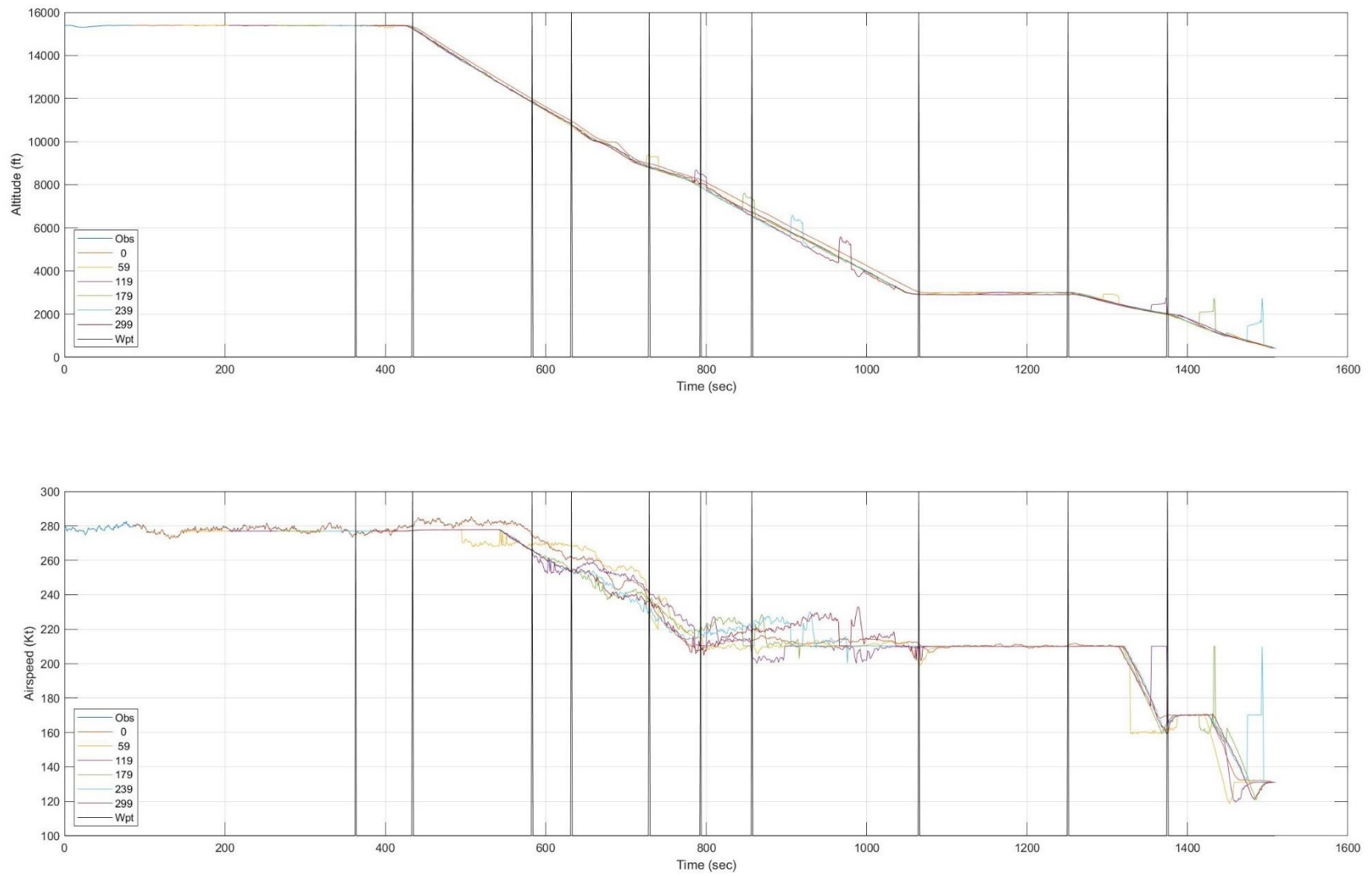
Figure E. 26: Test Flight 36: Observed and Predicted Altitude and Airspeed as a Function of Time t
