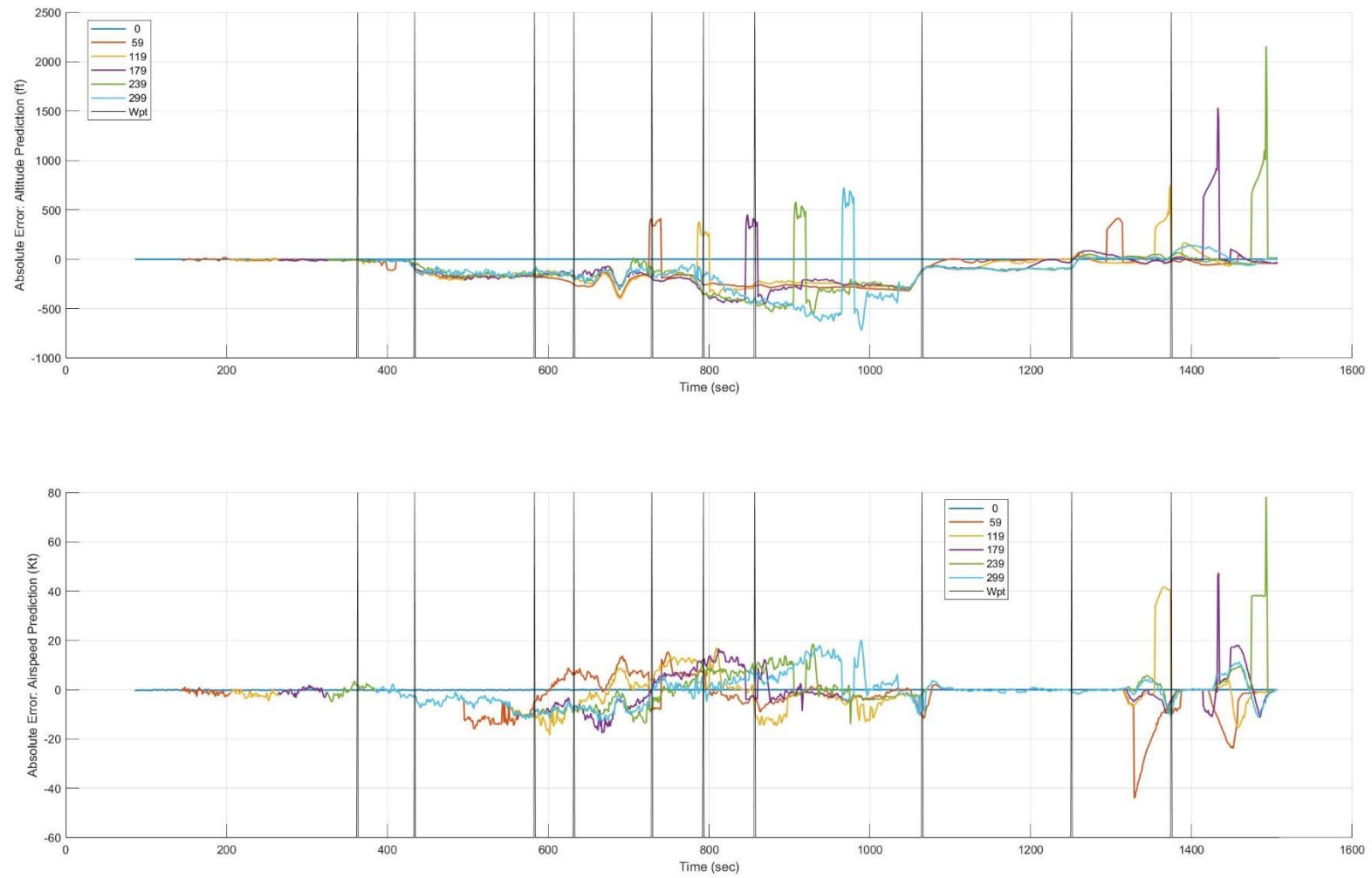
Figure 53: Test Flight 36: Absolute Error of Predicted Altitude and Airspeed as a Function of Time t
