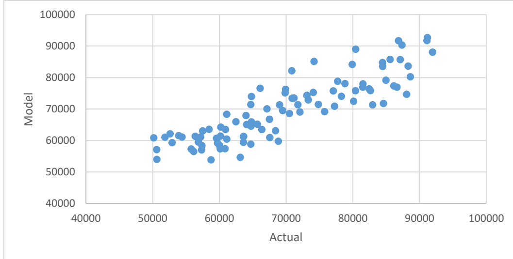
Figure 40: Scatter Plot of Actual and Modeled Cumulative RMS Absolute Error of Energy Prediction ( \rho = 0.87 )
