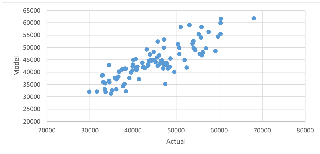
Figure 38: Scatter Plot of Actual and Modeled Cumulative RMS Absolute Error of Altitude Prediction ( \rho = 0.85 )
