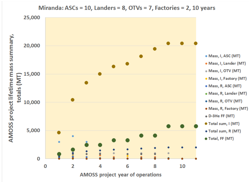
Figure B1. AMOSS on-orbit mass requirements for 10 years of operations, Miranda, 10 ASCs.
