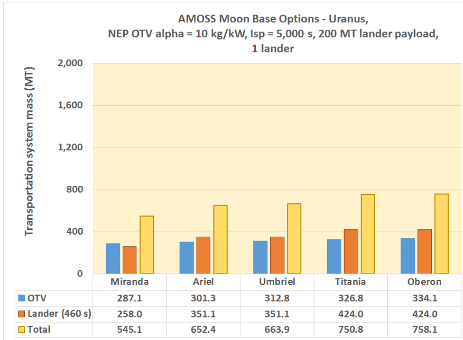
Figure 2. Uranus - Transportation System Mass – NEP alpha = 10 kg/kW, Isp = 5,000 s, Lander Isp = 460 s (one lander included in each case).
