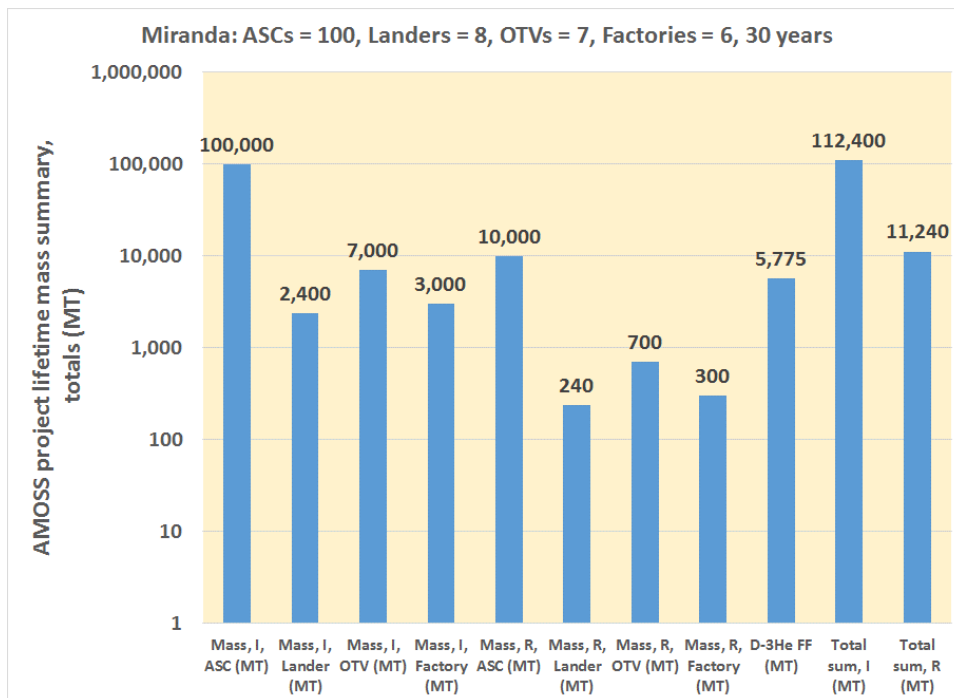
Figure A6. AMOSS on-orbit mass requirements for 30 years of operations, total vehicle masses, Miranda, 100 ASCs.
