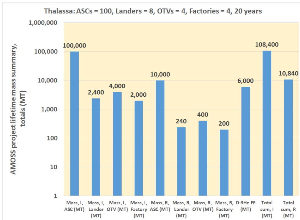
Figure C4. AMOSS on-orbit mass requirements for 20 years of operations, total vehicle masses, Thalassa, 100 ASCs.
