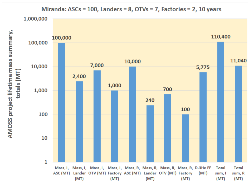
Figure 6. AMOSS on-orbit mass requirements for 10 years of operations, total vehicle masses, nominal case.
