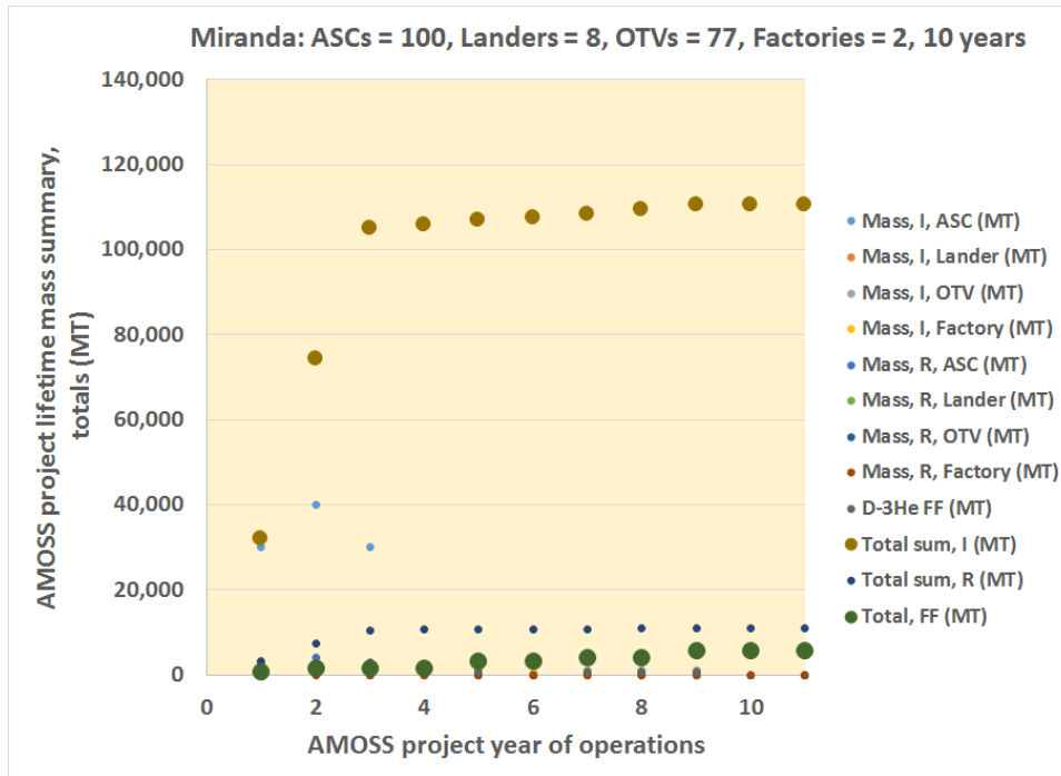
Figure 5. AMOSS on-orbit mass requirements for 10 years of operations, nominal case.
