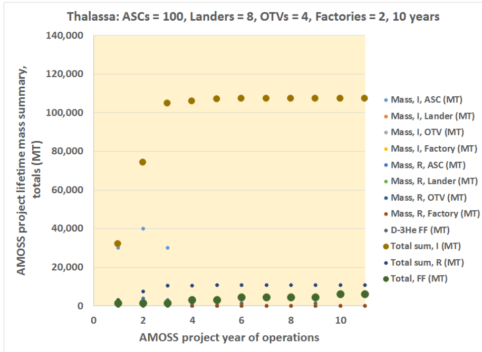
Figure C1. AMOSS on-orbit mass requirements for 10 years of operations, Thalassa, 100 ASCs.
