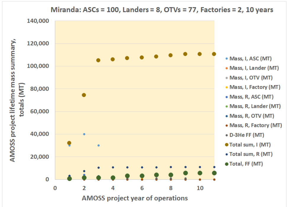
Figure A1. AMOSS on-orbit mass requirements for 10 years of operations, Miranda, 100 ASCs.
