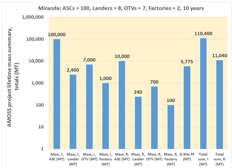
Figure A2. AMOSS on-orbit mass requirements for 10 years of operations, total vehicle masses, Miranda, 100 ASCs.
