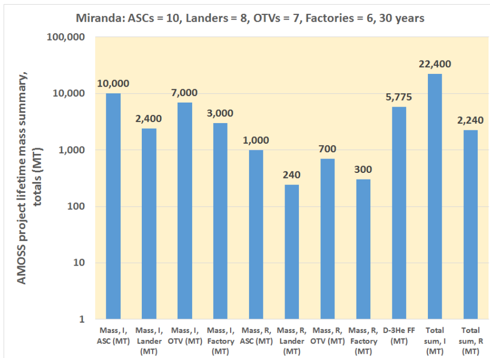
Figure B6. AMOSS on-orbit mass requirements for 30 years of operations, total vehicle masses, Miranda, 10 ASCs
