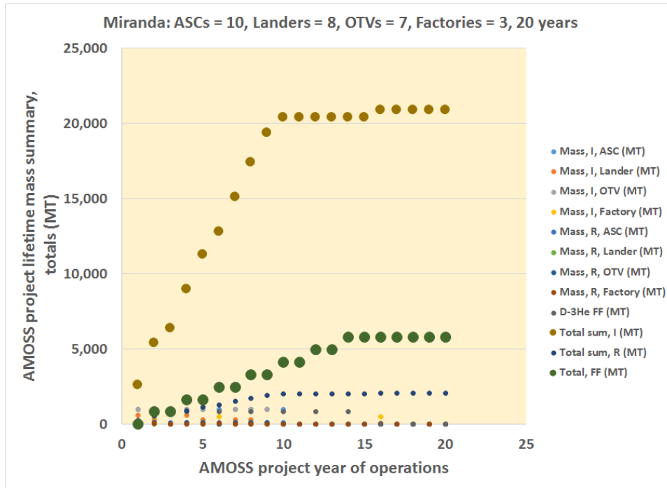
Figure B3. AMOSS on-orbit mass requirements for 20 years of operations, Miranda, 10 ASCs.
