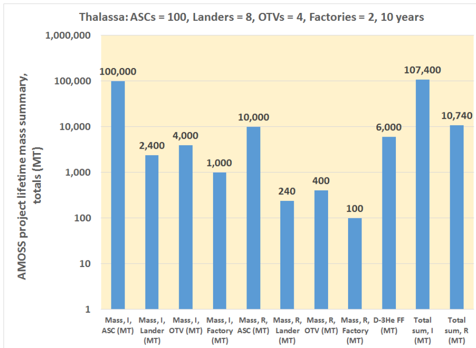
Figure C2. AMOSS on-orbit mass requirements for 10 years of operations, total vehicle masses, Thalassa, 100 ASCs.
