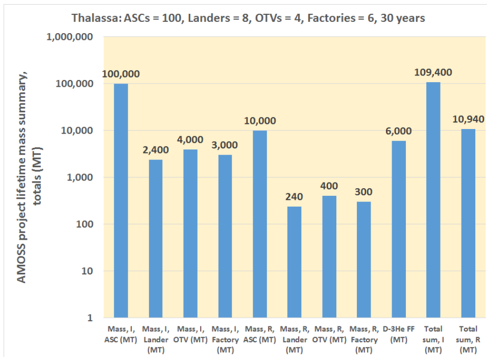
Figure C6. AMOSS on-orbit mass requirements for 30 years of operations, total vehicle masses, Thalassa, 100 ASCs.
