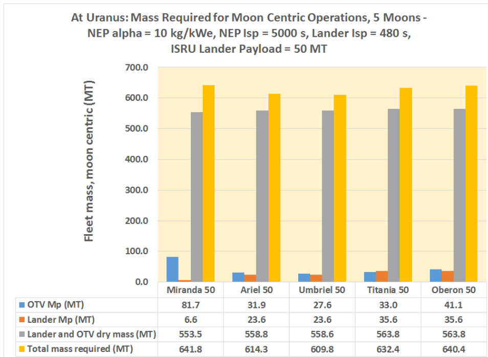
Figure VIII. Mass required for centric moon operations: Uranus
