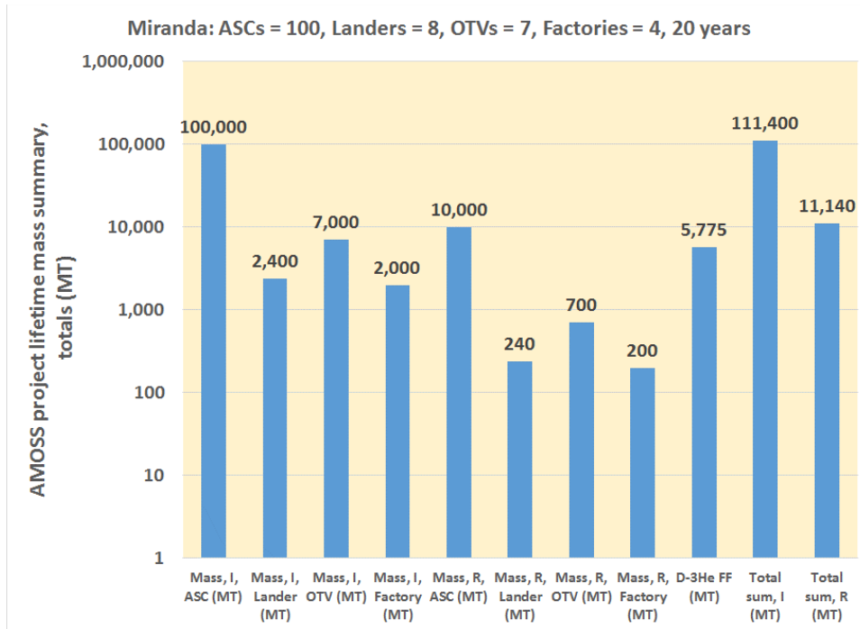
Figure A4. AMOSS on-orbit mass requirements for 20 years of operations, total vehicle masses, Miranda, 100 ASCs.
