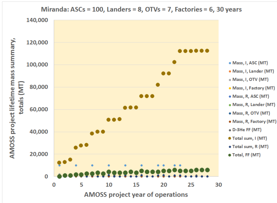
Figure A5. AMOSS on-orbit mass requirements for 30 years of operations, Miranda, 100 ASCs.
