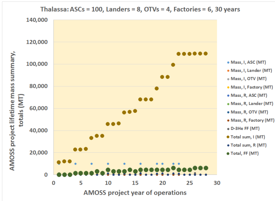
Figure C5. AMOSS on-orbit mass requirements for 30 years of operations, Thalassa, 100 ASCs.
