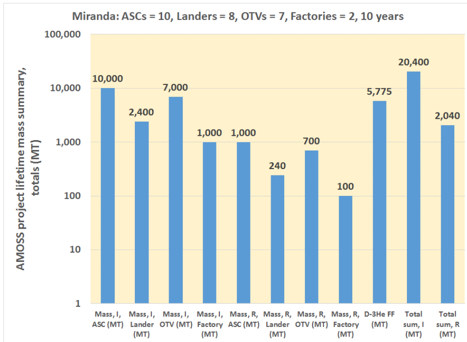
Figure B2. AMOSS on-orbit mass requirements for 10 years of operations, total vehicle masses, Miranda, 10 ASCs.
