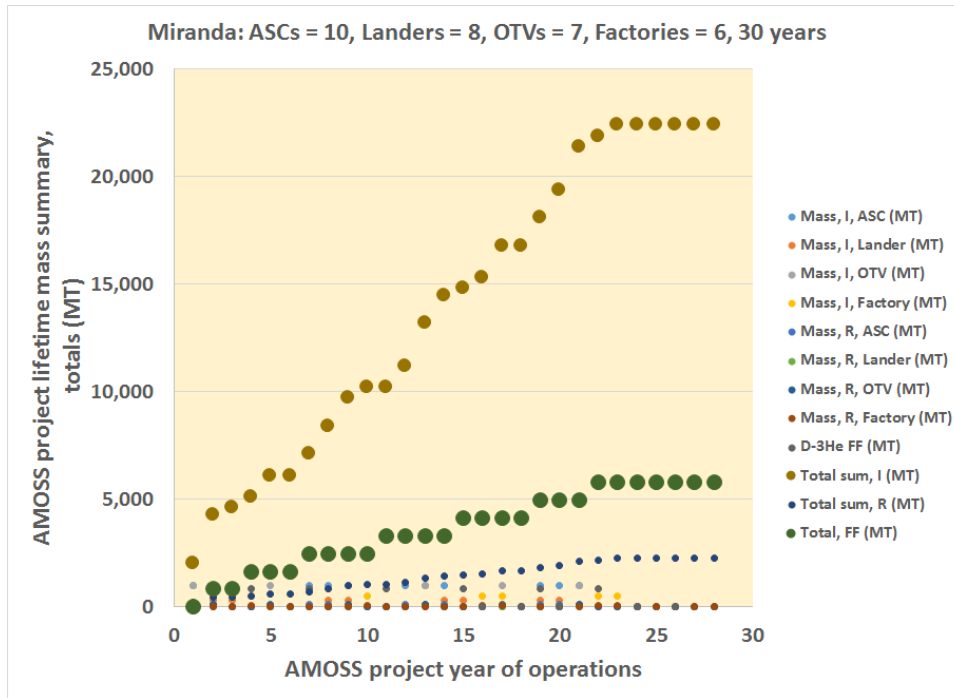
Figure B5. AMOSS on-orbit mass requirements for 30 years of operations, Miranda, 10 ASCs
