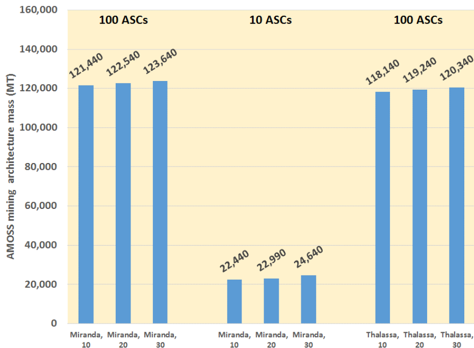
Figure 7. AMOSS mining architecture masses: Miranda with 100 and 10 ASCs and Thalassa with 100 ASCs.
