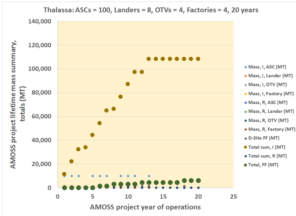
Figure C3. AMOSS on-orbit mass requirements for 20 years of operations, Thalassa, 100 ASCs..
