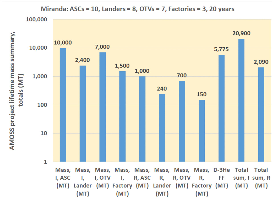
Figure B4. AMOSS on-orbit mass requirements for 20 years of operations, total vehicle masses, Miranda, 10 ASCs
