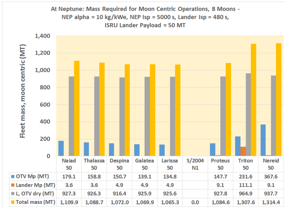
Figure 8. Mass required for centric moon operations: Neptune
