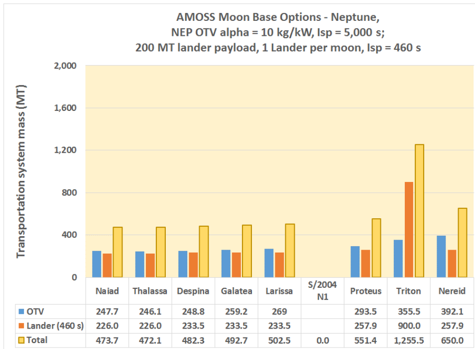
Figure 3. Neptune - Transportation System Mass – NEP alpha = 10 kg/kW, Isp = 5,000 s, Lander Isp = 460 s
