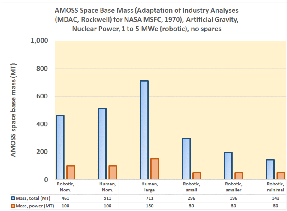
Figure 1. Space base mass estimates (Ref. 1)
