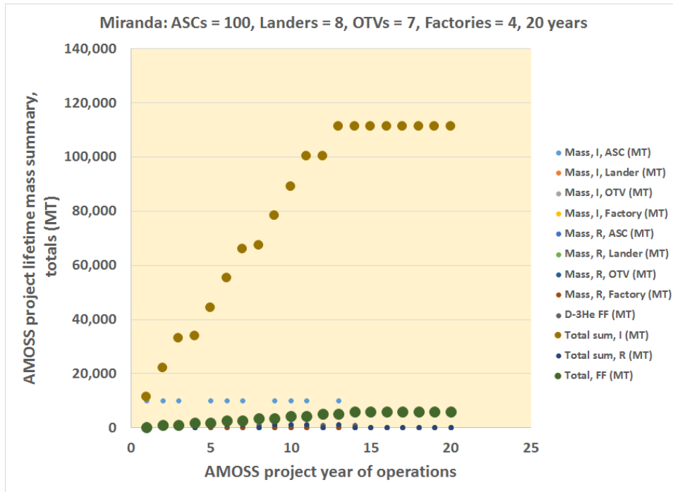
Figure A3. AMOSS on-orbit mass requirements for 20 years of operations, Miranda, 100 ASCs.
