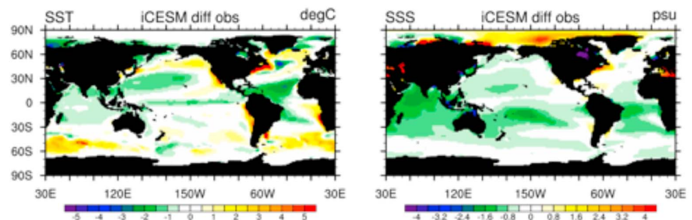
Figure 7. Model annual mean (a) sea surface temperature (SST) and (b) sea surface salinity (SSS), minus the WOA13v2 observational climatology (Boyer et al., 2013). The model results are averaged over years 1955–2005. Biases are in ^\circ\text{C} and PSU, respectively.
