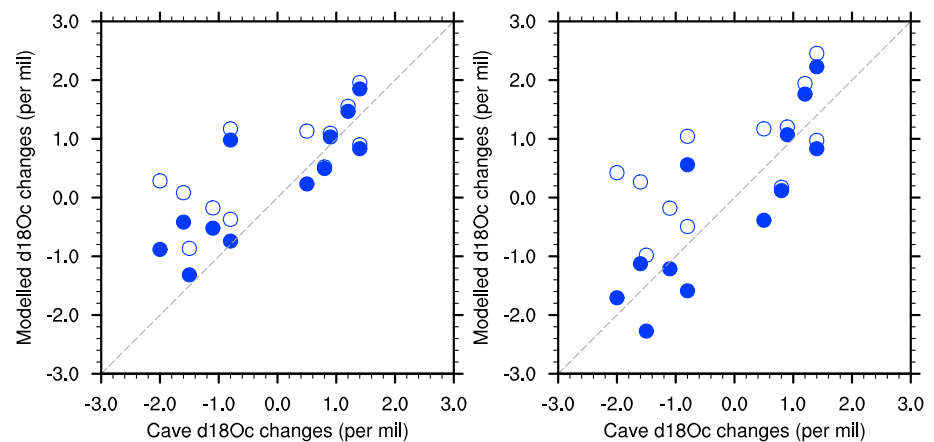
Figure 12. A model-data comparison of response in speleothem \delta^{18}\text{O} during Heinrich events (unit: ‰). The response in the model is the difference between a water hosing experiment and a preindustrial control simulation. Either (left) 0.25-Sv or (right) 0.5-Sv freshwater with a \delta^{18}\text{O} signature of -30\text{‰} was applied for 300 years in the water hosing experiments. Open circles are results if only the indirect climate effects are considered (no influence from meltwater \delta^{18}\text{O} ); filled circles include both effects. Modeled \delta^{18}\text{O}_c is calculated from model \delta^{18}\text{O}_p and temperature using Kim and O'Neil (1997). Reproduced from Zhu et al. (2017a), Figure S3. Please refer to Zhu et al. (2017a) for details of the simulations and model-data comparison.
