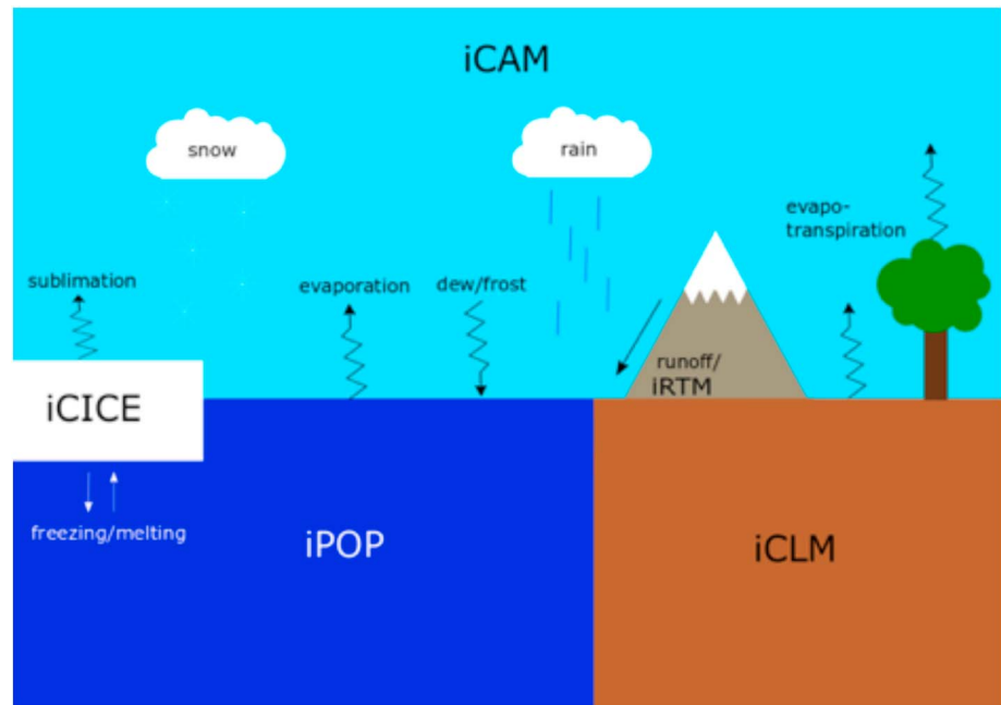
Figure 1. A schematic of iCESM1 showing the five major model components (iCAM, iCLM, iRTM, iPOP, and iCICE) and all of the major intercomponent fluxes that impact water isotopes. It should be noted that although some of these fluxes are only shown once, they occur for multiple components (e.g., dew/frost can occur between iCAM and iCLM, iPOP, and iCICE).
