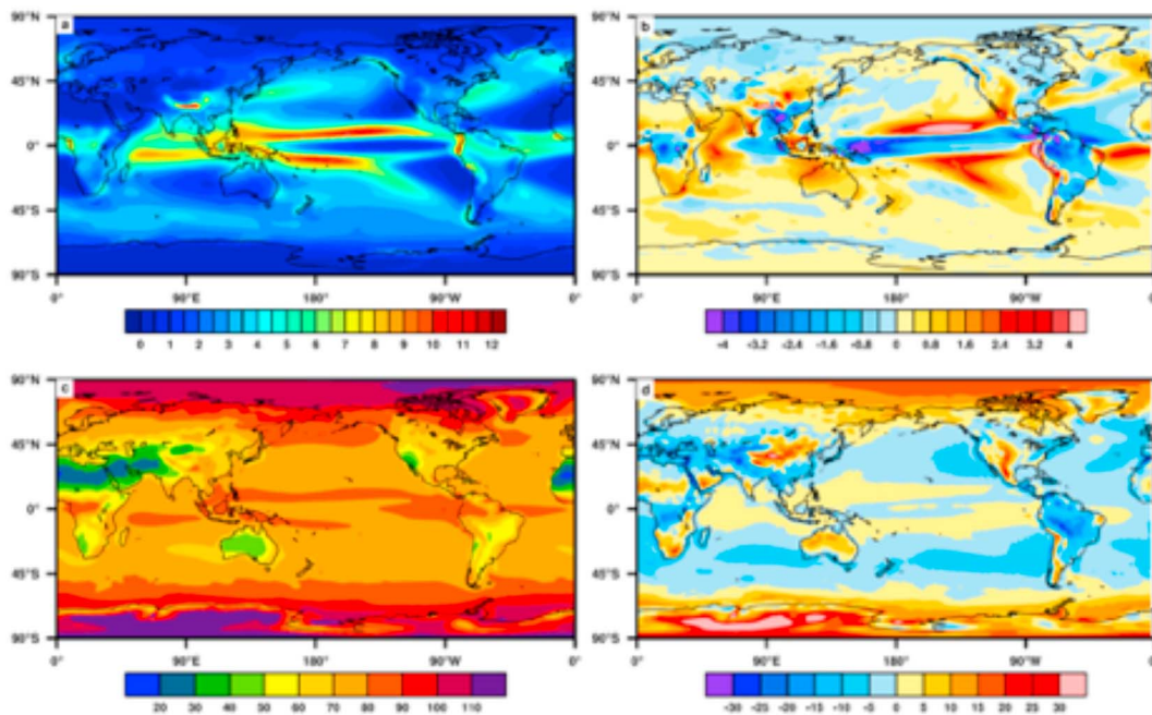
Figure 2. (a) Annual average precipitation in mm/day and (c) surface relative humidity in percent as simulated by iCESM1. Also shown are the differences between iCESM1 and ERA-Interim for (b) precipitation and (d) surface relative humidity. The iCESM1 values were averaged over model years 1950–2005.
