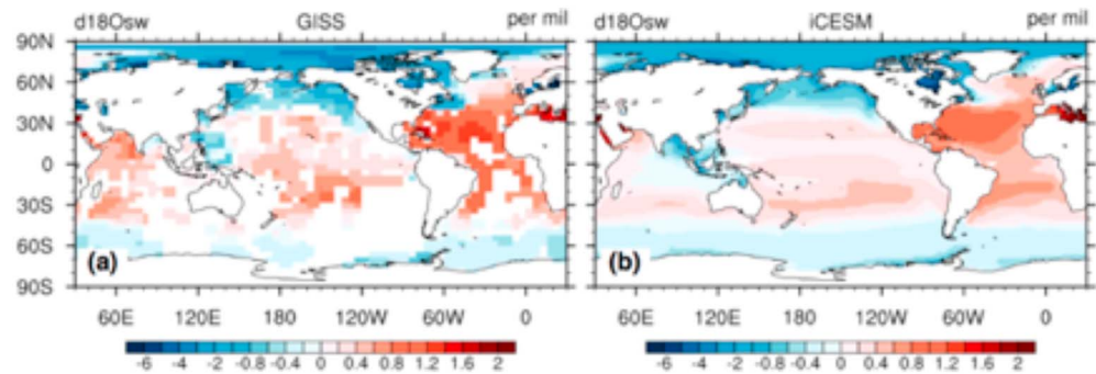
Figure 8. Model-data comparison of annual mean \delta^{18}\text{O} composition of surface seawater (unit: ‰). (a) The GISS data set and (b) iCESM simulation (1955–2005).
