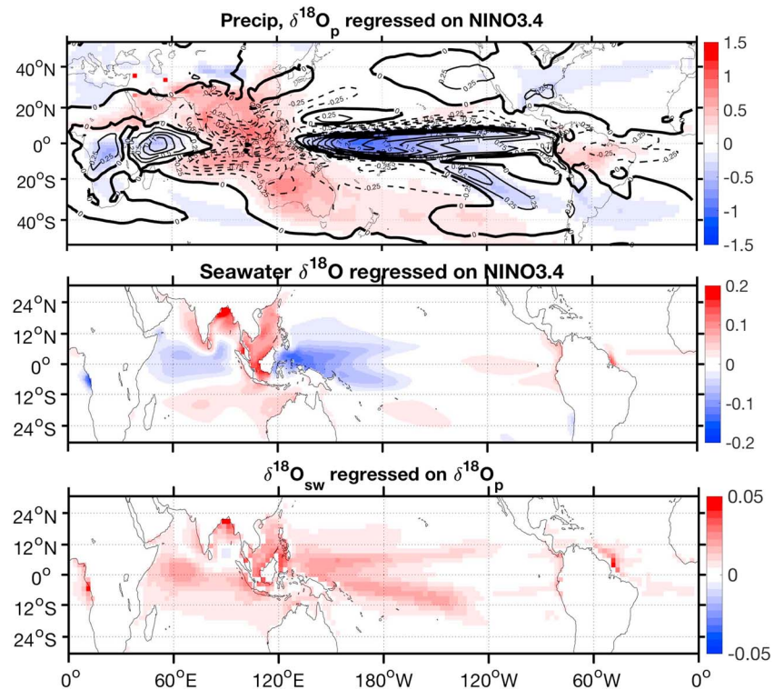
Figure 11. (a) Anomalies in precipitation (contours) and \delta^{18}\text{O} of precipitation (colors) regressed on Niño3.4 SSTA in iCESM. Time period is the entire length of an iLME full-forcing experiment (850–2005), and anomalies are all computed relative to a 20-year moving window. (b) Same as in (a), for seawater \delta^{18}\text{O} anomalies. (c) Regression of grid point seawater \delta^{18}\text{O} on precipitation \delta^{18}\text{O} anomalies. Time period and anomaly computation is the same as in (a).
