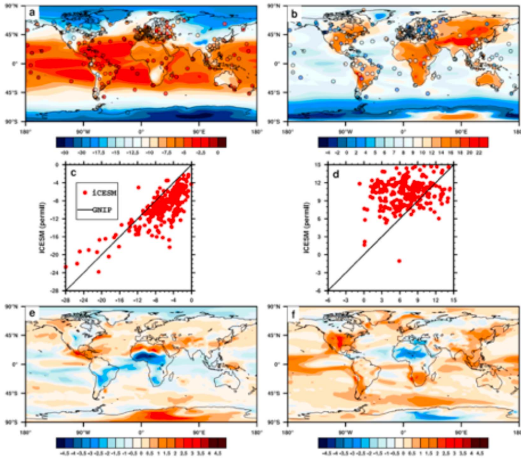
Figure 4. (a) Annual average precipitation \delta^{18}\text{O} and (b) d-excess from iCESM1.2 (contours) and GNIP (circles). Also shown are the (c) average \delta^{18}\text{O} and (d) d-excess values from the model grid cells closest to each GNIP station, compared against those GNIP values. The black line shows the values for a “perfect” match with GNIP. The differences between iCESM1.2 and iCAM5/iCLM4 with prescribed SSTs are also shown for (e) precipitation \delta^{18}\text{O} and (f) d-excess. The iCESM1.2 values were averaged over model years 1950–2005. The iCAM5 and GNIP values were the same used in Nusbaumer et al. (2017).
