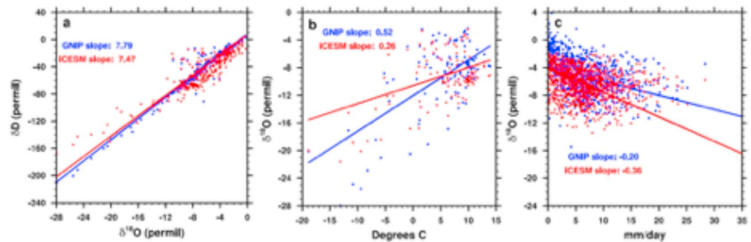
Figure 6. Scatterplots of (a) time-averaged precipitation-weighted \delta^{18}\text{O} and \delta\text{D} , (b) surface air temperature and \delta^{18}\text{O} of precipitation in the extra tropics, and (c) precipitation rate and \delta^{18}\text{O} of precipitation in the tropics for GNIP (blue) and iCESM (red) at the grid cell nearest to the GNIP station. The solid lines represent the linear regression between the respective quantities, with the slopes of those regression lines shown in the legends for both GNIP and iCESM. The temperature plot (b) only uses stations poleward of 45^\circ\text{N/S} , whereas the precipitation plot (c) only uses stations between 15^\circ\text{N/S} and 90^\circ\text{E} to 255^\circ\text{E} . The precipitation plot also uses monthly values, while all other plots use the long-term averages for each station.
