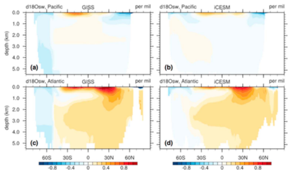
Figure 9. Model-data comparison of zonal mean seawater \delta^{18}\text{O} (unit: ‰). Pacific zonal mean in (a) the GISS data set and (b) the iCESM simulation averaged between year 1955 and 2005. (c and d) Same as in (a) and (b) but for the Atlantic zonal mean.
