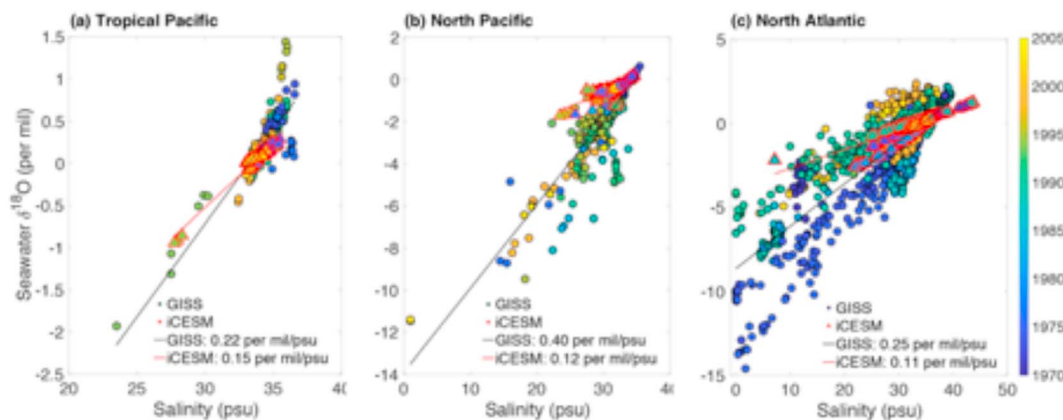
Figure 10. Relationship between salinity and seawater \delta^{18}\text{O} , in both iCESM and the GISS database. Color shading indicates the model year of the simulation. Circles indicate GISS data and triangles iCESM output. Note that iCESM output has been subsampled to match the latitudes/longitudes/times corresponding to GISS data points; best fit regressions for GISS and iCESM are plotted as black and red lines, respectively. (a) Tropical Pacific ( 25^{\circ}\text{S} – 25^{\circ}\text{N} , 90^{\circ}\text{E} – 90^{\circ}\text{W} ), (b) North Pacific ( 30 – 70^{\circ}\text{N} , 90^{\circ}\text{E} – 90^{\circ}\text{W} ), and (c) North Atlantic ( 0 – 70^{\circ}\text{N} , 100^{\circ}\text{W} – 60^{\circ}\text{E} ).
