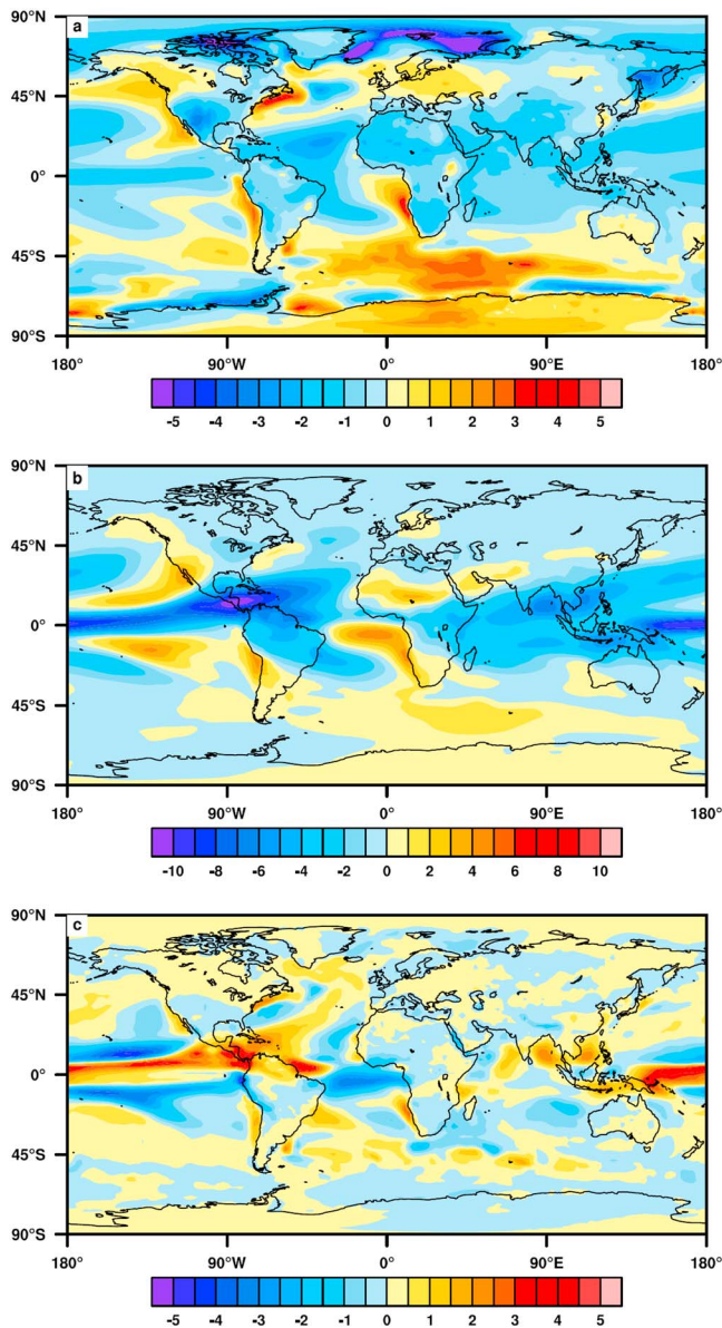
Figure 5. Climatological differences in (a) surface temperature, defined here as the temperature at the lowest atmospheric model layer; (b) precipitable water; and (c) evaporation minus precipitation, between iCESM1 and iCAM5/iCLM4 with prescribed SSTs and sea ice.
