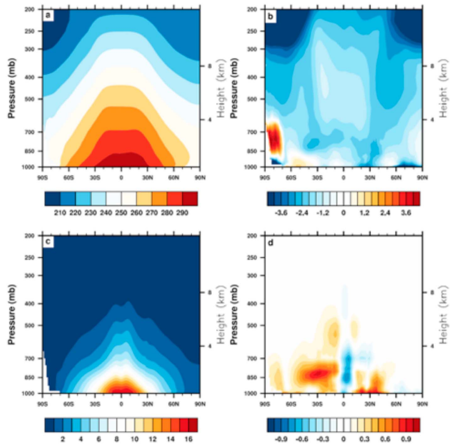
Figure 3. (a) Zonal and annual average air temperature in kelvin and (c) specific humidity in g/kg as simulated by iCESM1.2. Also shown are the differences between iCESM and ERA-Interim for (b) air temperature and (d) specific humidity. The iCESM values were averaged over model years 1950–2005.
