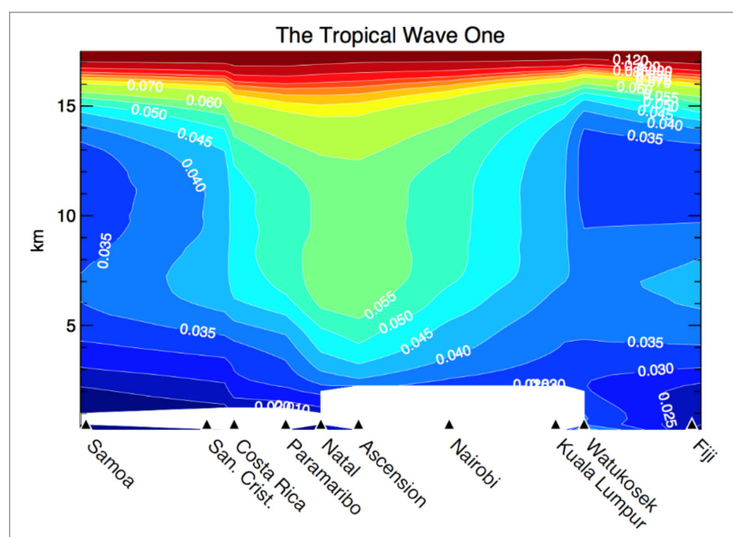
Figure 2.3.2: Longitudinal cross section of contours of tropospheric ozone mixing ratios (units of ppm), computed from 0.25 km averages of 1998-2016 reprocessed data, for the 10 tropical stations, labeled by station on the x-axis.
