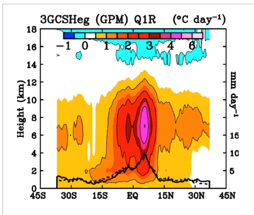
Figure 2.1.7: Zonal cross section (latitude vs height) of mean cloud heating (latent heating + cloud eddy effects) retrieved from the latest version of the Goddard Convective-Stratiform Heating (CSH) algorithm for the 3 month period, April-June 2014. Overlaid are zonal mean surface rainfall (solid black line) and zonal mean equivalent surface rainfall.
