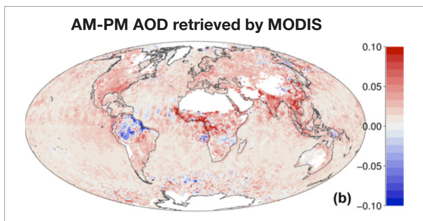
Figure 2.2.7: 0.015 or 13% offset nearly everywhere. Why?
