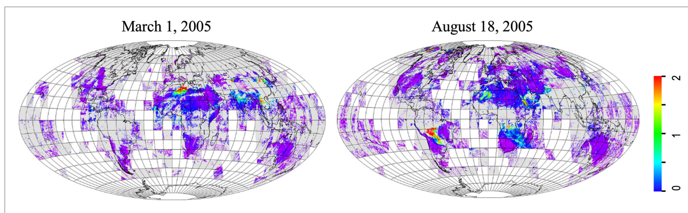
Figure 2.2.11: Aerosol Optical Depth
