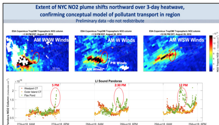
Figure 4.7b: Combined TROPOMI (top panels) and Pandora (bottom panels) view of Long Island Sound nitrogen dioxide pollution plume evolution during the LISTOS campaign. Plots: Lukas Valin, EPA.
