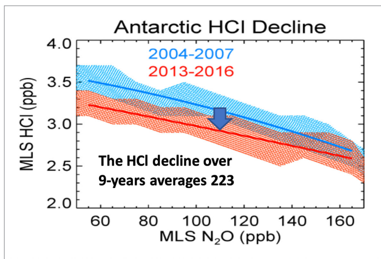
Figure 2.3.1: Decreases in HCl for constant \text{N}_2\text{O} values identify changes in stratospheric chlorine loading that are independent of atmospheric dynamical variability.
