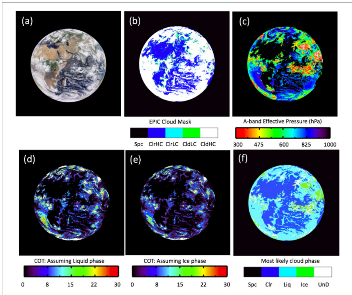
Figure 3.1.2.1c: Sample EPIC L2 cloud products for the observations at 08 UTC on Aug. 18, 2016: (a) EPIC RGB image; (b) EPIC cloud mask. Spc: space pixels, ClrHC: high confidence clear, ClrLC: low confidence clear, CldLC: low confidence cloudy, and CldHC: high confidence cloudy; (c) oxygen A-band cloud effective pressure; (d) cloud optical thickness assuming liquid phase; (e) cloud optical thickness assuming ice phase; (f) most likely cloud phase. Other L2 cloud products not shown include oxygen B-band cloud effective pressure, and A- and B-band cloud effective height.
