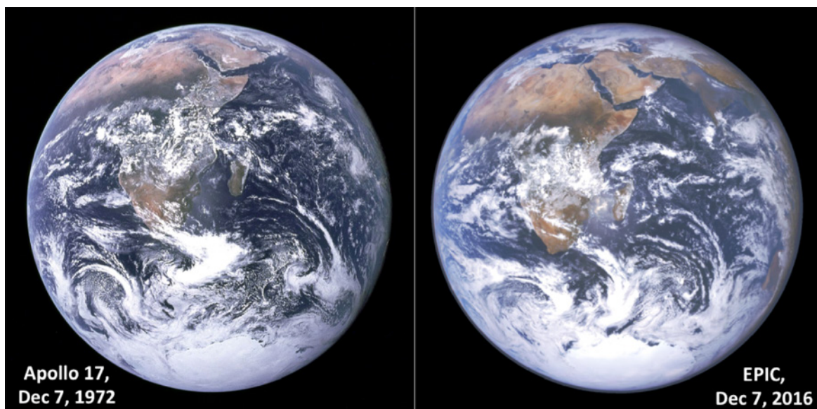
Figure 3.1.2.1a: Apollo 17 (“blue marble”) and DSCOVR EPIC images acquired on December 7, 1972 and 2016, 44 years apart.
