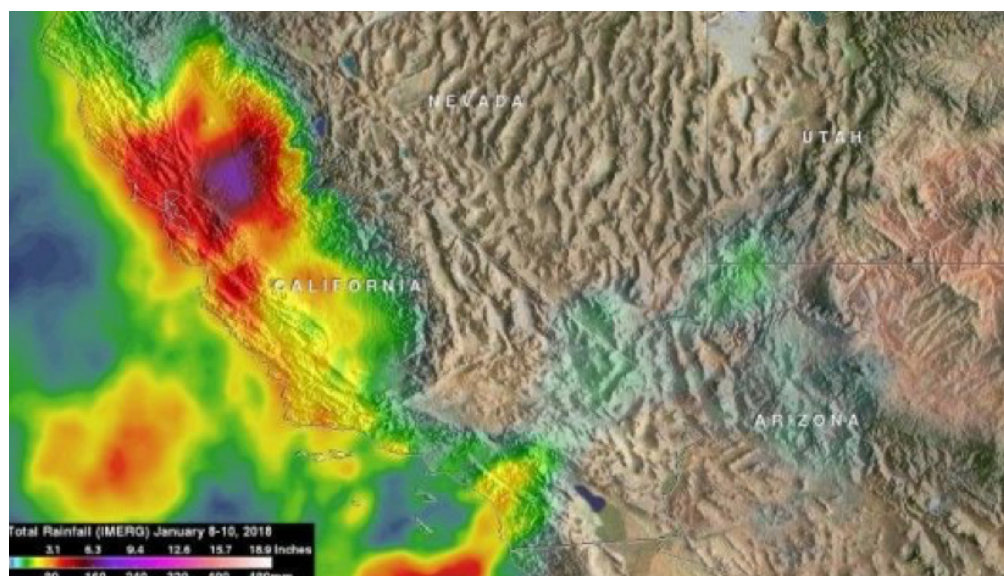
NASA's IMERG analysis of Jan. 8 through 10, 2018 revealed that the heaviest rainfall occurred over the Sacramento Valley where over 8 inches (203 mm) were indicated. A rainfall total of 5 inches (127 mm) was reported in Ventura County. Credit: NASA/JAXA/Hal Pierce
