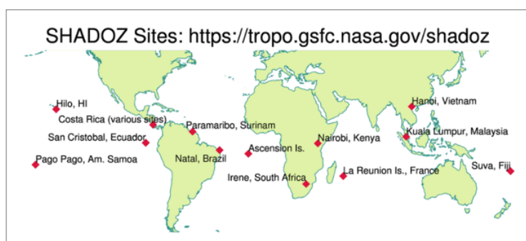
Figure 4.8a: Map of operating SHADOZ stations in 2018.
