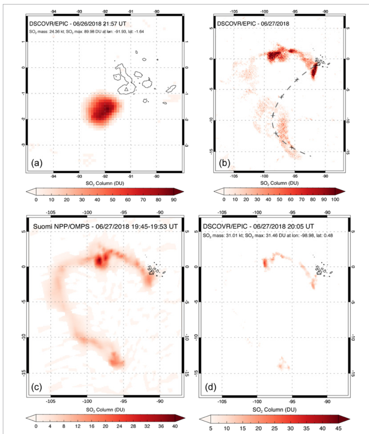
Figure 3.1.2.1c: (a) EPIC detection of strong SO 2 emissions from Sierra Negra (Galápagos Islands; triangle) at 21:57 UT on June 26, 2018; (b) Cumulative SO 2 column amounts measured in the Sierra Negra volcanic plume by EPIC in 8 exposures on June 27, 2018 (14:38-22:16 UT). Dashed line shows a 36-hour HYSPLIT model trajectory for an eruption to 11 km altitude beginning at 19:00 UT on June 26, with crosses every 6 hours. (c) SNPP/OMPS map of SO 2 emissions from Sierra Negra at 19:50 UT on June 27; (d) EPIC SO 2 map at 20:05 UT on June 27.
