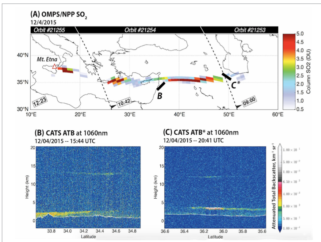
Figure 2.1.1: CATS observed the Mt. Etna plume on December 4, 2015 at altitude of 12-14 km (B & C), higher than estimated using trajectory analysis (8-12 km.) CATS near-real time data provided an unprecedented opportunity to monitor and predict volcanic plume transport. J. Yorks (612), E. Hughes, (614, UMD); et al.
