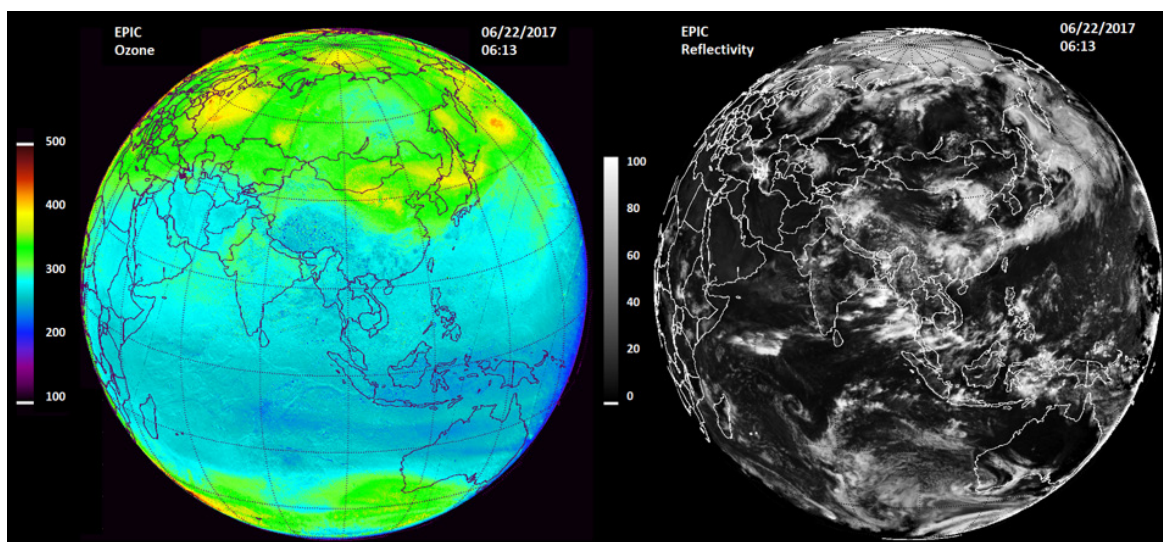
Figure 3.1.2.1b: Ozone (left in DU: 100 to 500 DU) and reflectivity (Lambert equivalent reflectivity, LER, right in percent: 0 to 100) for June 22, 2017 at 06:13 GMT. These are the basic input data needed to compute UV radiation reaching the ground.
