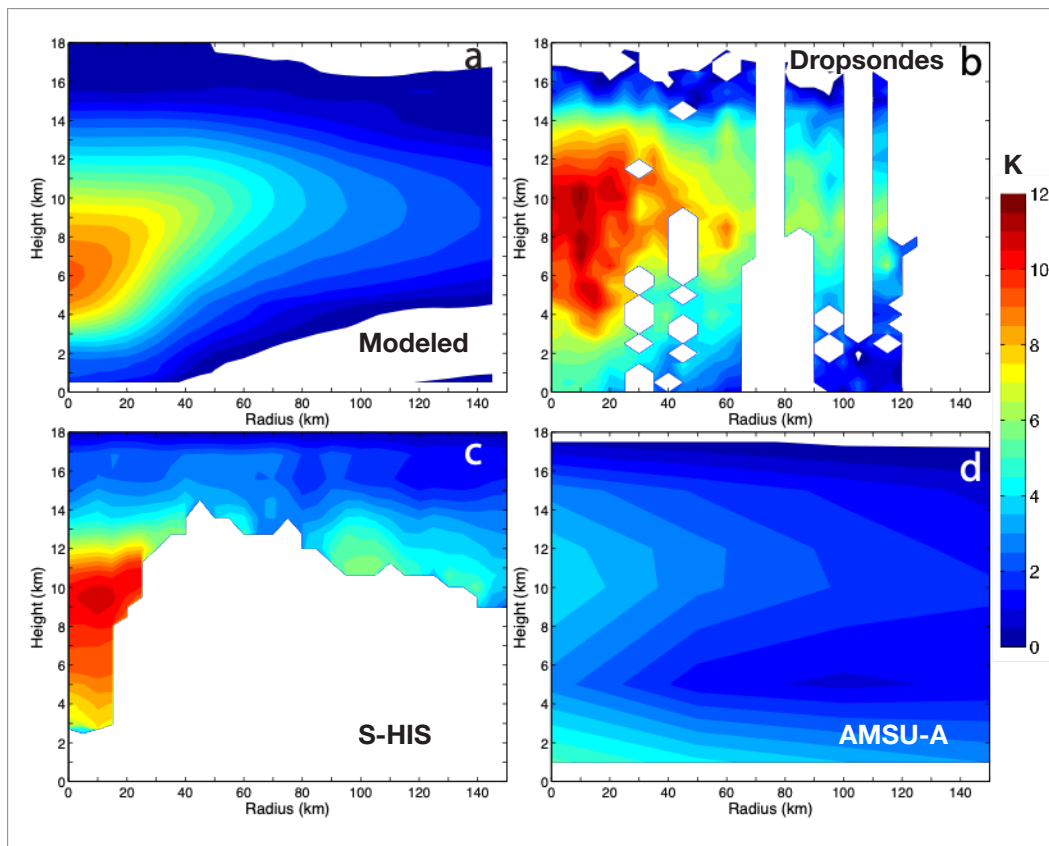
Figure 2.1.3: A comparison between Hurricane Edouard’s (2014) modeled and observed inner-core temperature structure highlights the need for direct measurements of the magnitude and vertical structure of the warm core of tropical cyclones.
