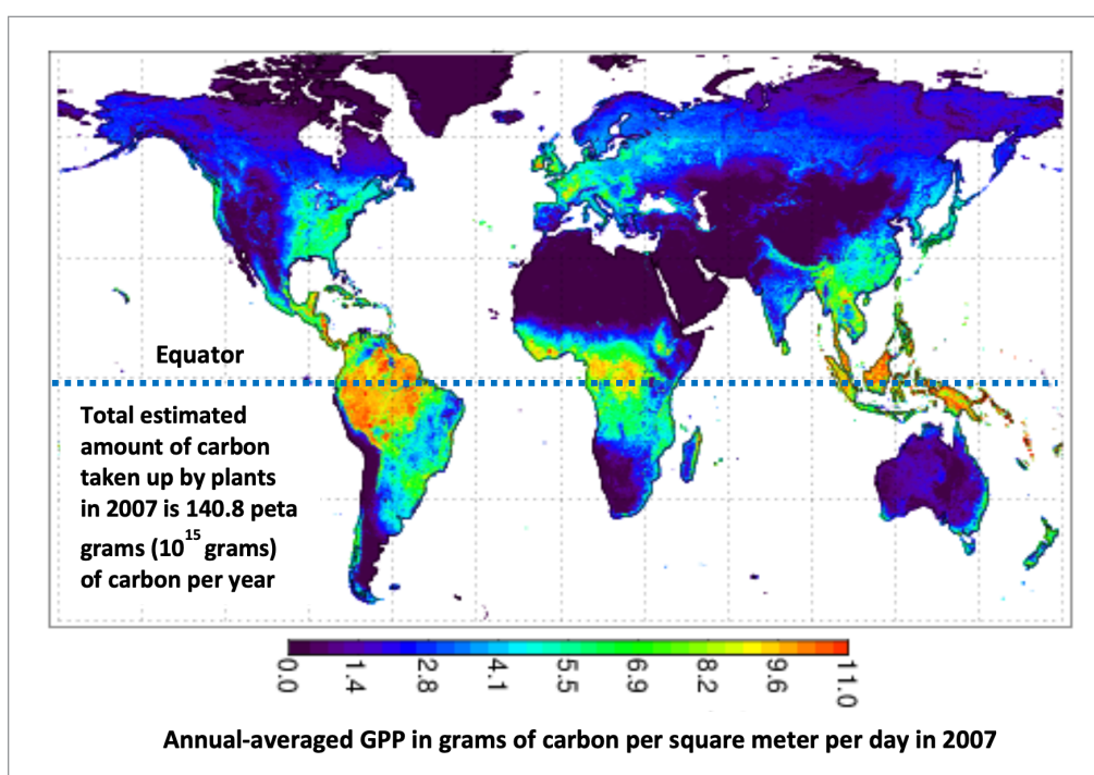
Figure 2.3.7: Map of averaged GPP estimated with remote sensing data for the year 2007.
