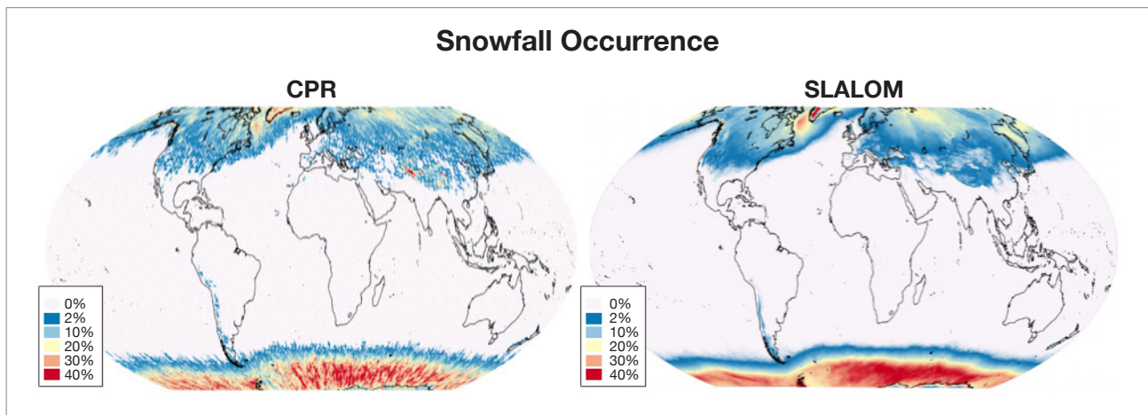
Figure 2.1.11: Caption: Snowfall percentage of occurrence as given by CPR and SLALOM, May 2014 to 2016.
