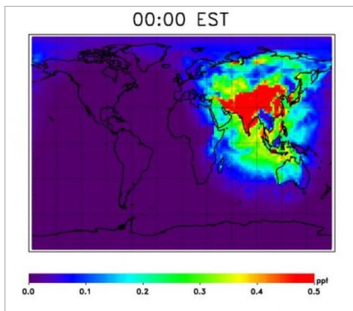
Model output of OH primary production over a 24-hour period in July tracks with sunlight across the globe. Higher levels of OH over populated land are likely from OH recycling in the presence of NO and NO 2 , which are common pollutants from cars and industry. Credit: NASA / Julie Nicely
