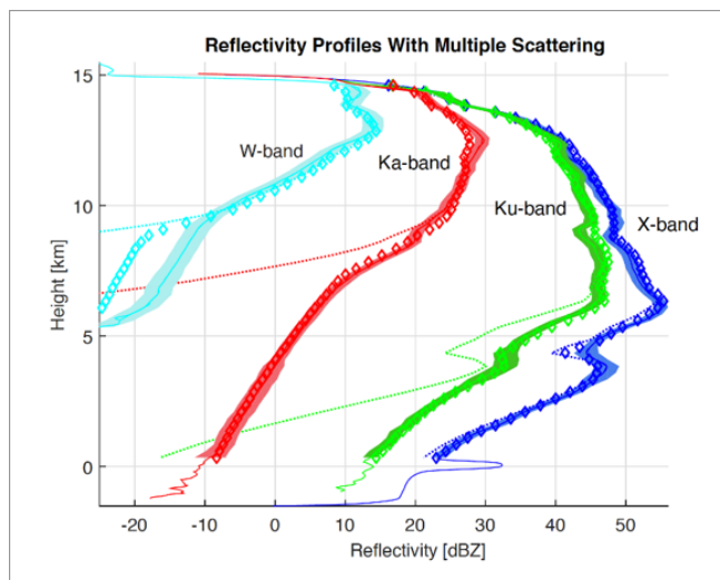
Figure 2.1.2: Four-frequency measurements from GSFC CRS (W), HIWRAP, and EXRAD radars on the NASA ER-2 for North Carolina hailstorms.
