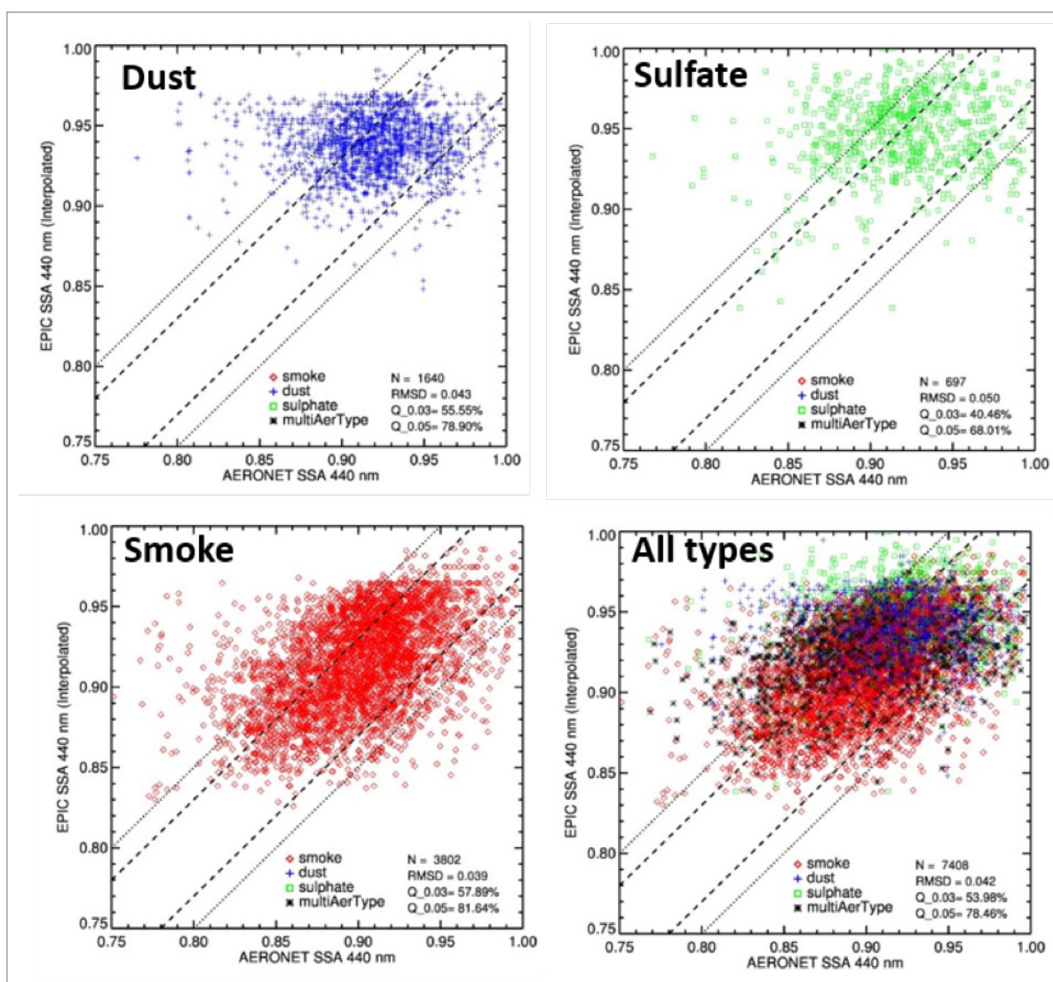
Figure 3.1.2.1d: Results of the evaluation of EPIC retrieved single scattering (SSA) albedo for different aerosol types using AERONET observations at 380 sites. EPIC retrieved SSA has been converted to 440 nm for comparison to AERONET measured values. Dashed (dotted) lines indicate agreement within 0.03 (0.05). AERONET SSA retrieval uncertainty is 0.03. Statistics indicate number of matchups (N), root mean square error difference (rmsd), and percent of points agreement within 0.03 and 0.05 (Q_0.03 and Q_0.05). Overall, 54% of compared pairs agree within 0.03, whereas 78% agree within 0.05.
