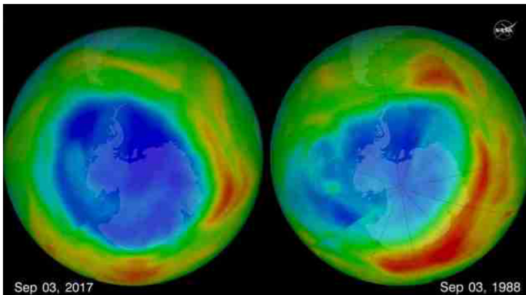
The hole in Earth’s protective ozone layer that forms over Antarctica each September was the smallest seen since 1988, according to NASA and NOAA. Credit: NASA’s Goddard Space Flight Center/Kathryn Mersmann
