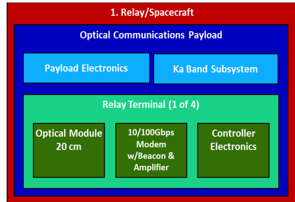
Figure 4: Optical Communications Payload
