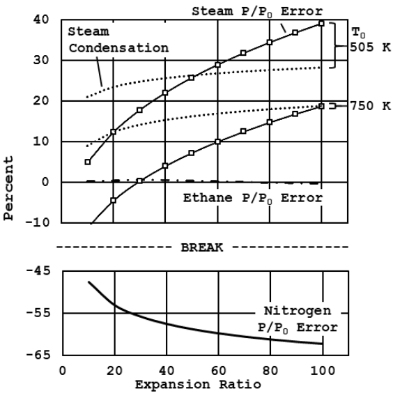
Figure 5 - Comparison of Simulant Gas Errors vs. LO 2 /LH 2 Hot-Fire, P 0 = 5 MPa, O/F=6.1
