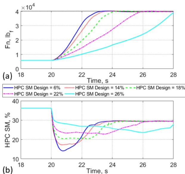
Fig. 10 Thrust and HPC SM response for a burst and chop simulation
