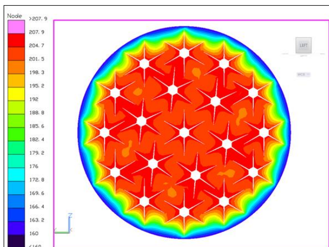
Figure 4. Simulated temperature cross-section of a heating 4BCO 2 sorbent bed at the end of a half-cycle. 18
