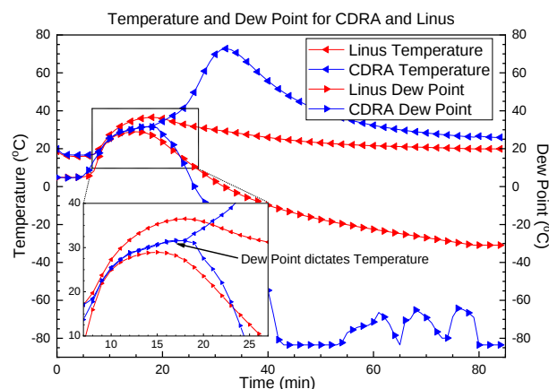
Figure 9. Temperature and dew point overlap indicating condensing conditions in the desorbing desiccant bed for the CDRA-like testbed whereas Linus does not exhibit this behavior.
