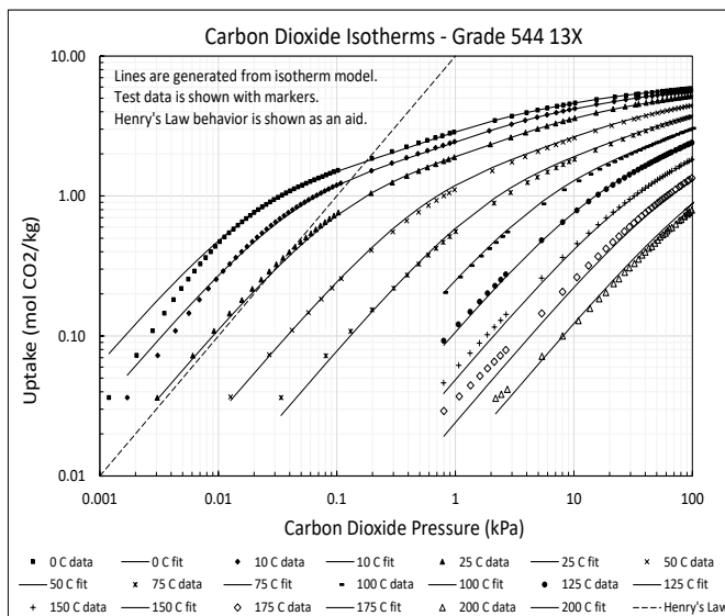
Figure 2. Pure component CO 2 isotherms at temperatures from 0°C up to 200°C. 6
