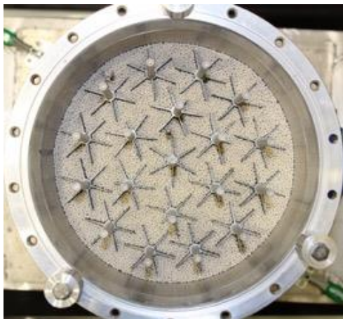
Figure 6. Partially filled sorbent bed for the prototype 4BMS ‘Linus’ system.
