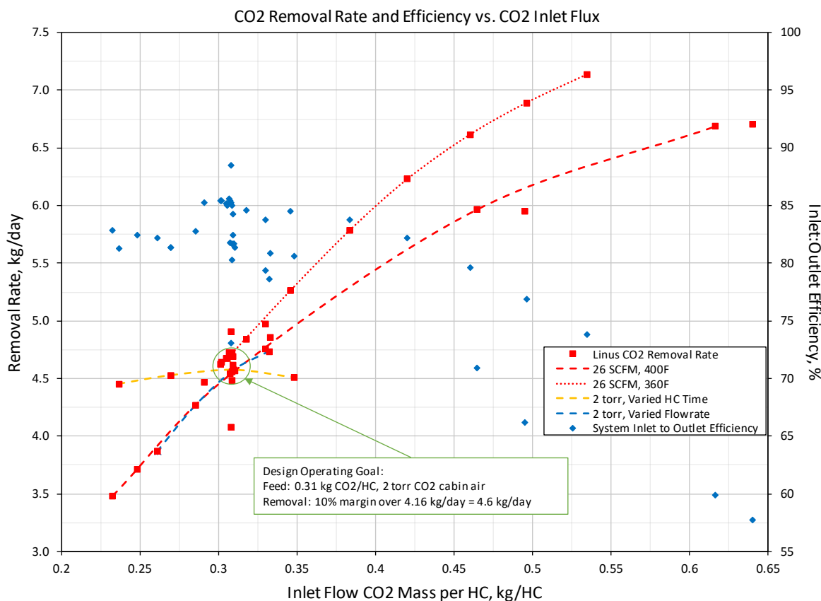
Figure 13. Performance map of Linus, the 4BCO 2 prototype. Blue and yellow dashed lines connect two selected test series where in each a single factor is varied. Red dashed lines show two similar test series where the heater setpoint was set to 360°F and 400°F.
