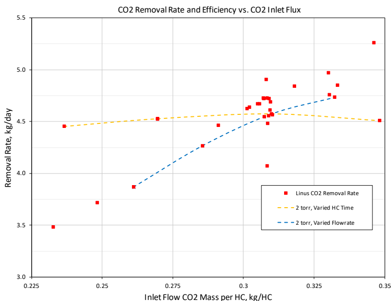
Figure 11. Performance map of Linus, the 4BCO 2 prototype. Blue and yellow dashed lines connect two selected test series where in each a single factor is varied.
