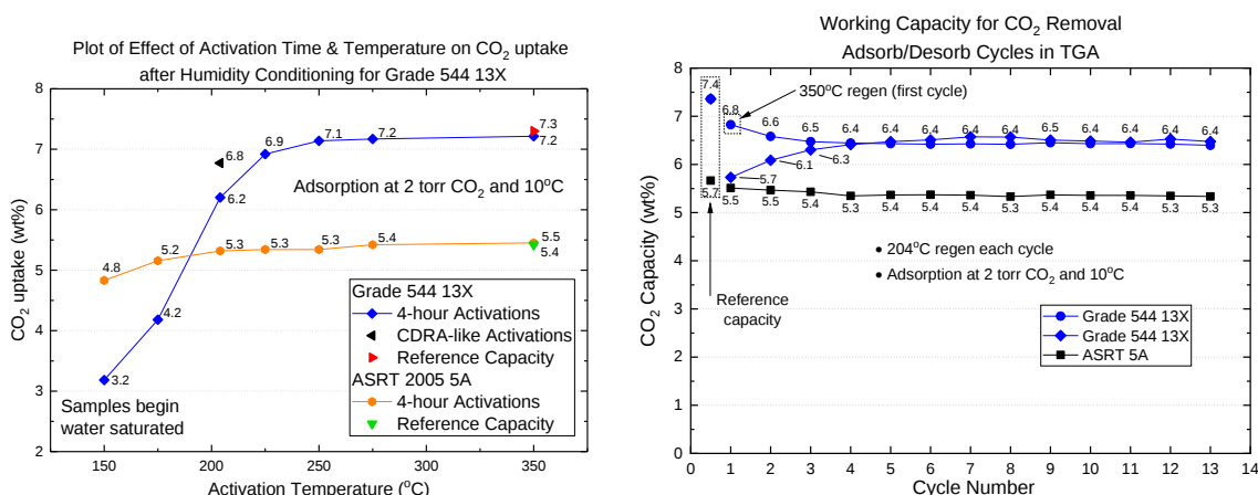
Figure 3. Effect of activation temperature on sorbent performance [left] and simulated 4BMS cyclic operation [right] for ASRT (5A) and Grade 544 (13X). Each point is the CO 2 capacity at end of a single adsorption cycle. Reduced capacity is attributed to trace water vapor in bottled gas supply to TGA. 4
