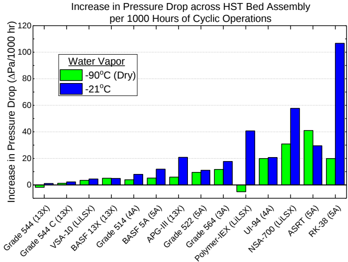
Figure 1. Rate of pressure drop increase which correlates to sorbent dust generation in sub-scale beds under dry and humid conditions subjected to thermal cycling. 5
