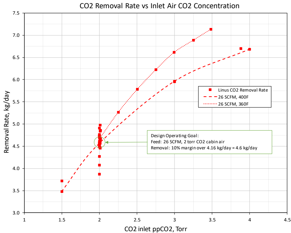
Figure 12. Performance map of Linus, the 4BCO 2 prototype. Red dashed lines show two similar test series where the heater setpoint was set to 360°F and 400°F.
