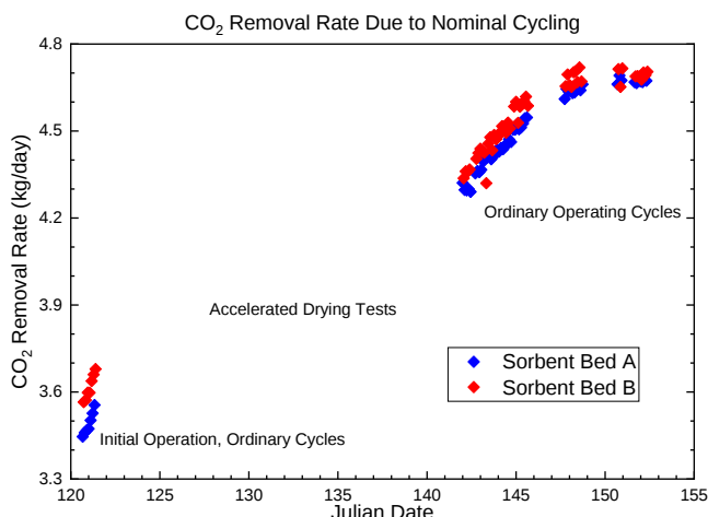
Figure 8. Recovery of CO 2 removal performance after initial assembly which had exposed dry sorbent to ambient humidity. The CO 2 removal was impaired but increased after numerous operating cycles to a steady-state.
