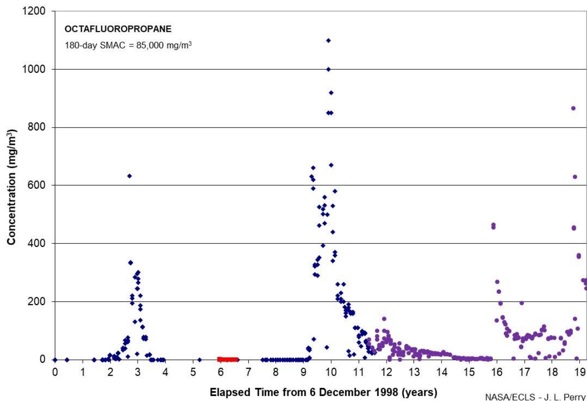
Figure 3. Octafluoropropane concentration in the ISS cabin atmosphere.
