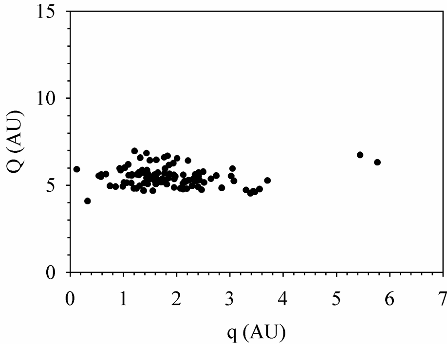
Figure 3.2 Peri/aphelion distributions of JF_m comets
