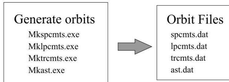
Figure 11.2 Files involved in the generation of orbits.
