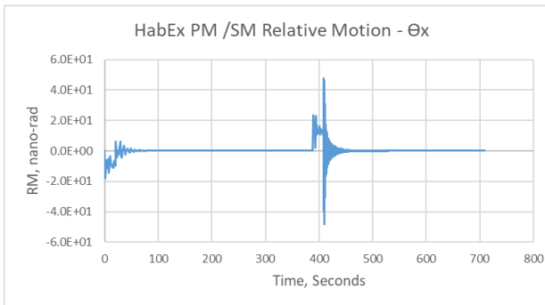
Figure 8. PM/SM X Rotation Direction Relative Motion
