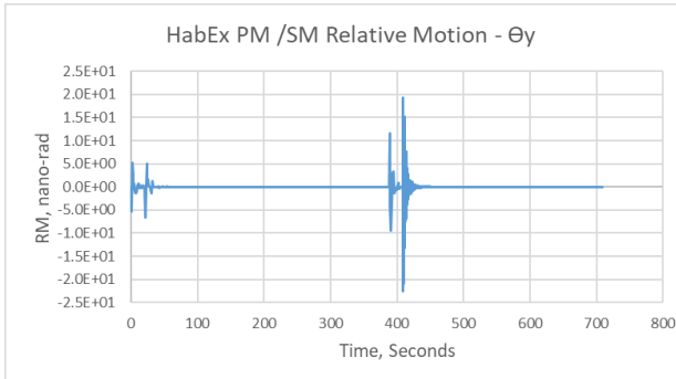
Figure 9. PM/SM Y Rotation Direction Relative Motion
