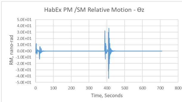
Figure 10. PM/SM Z Rotation Direction Relative Motion
