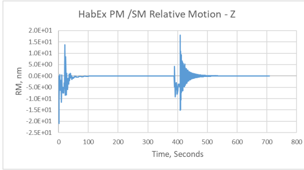
Figure 7. PM/SM Z Direction Relative Motion
