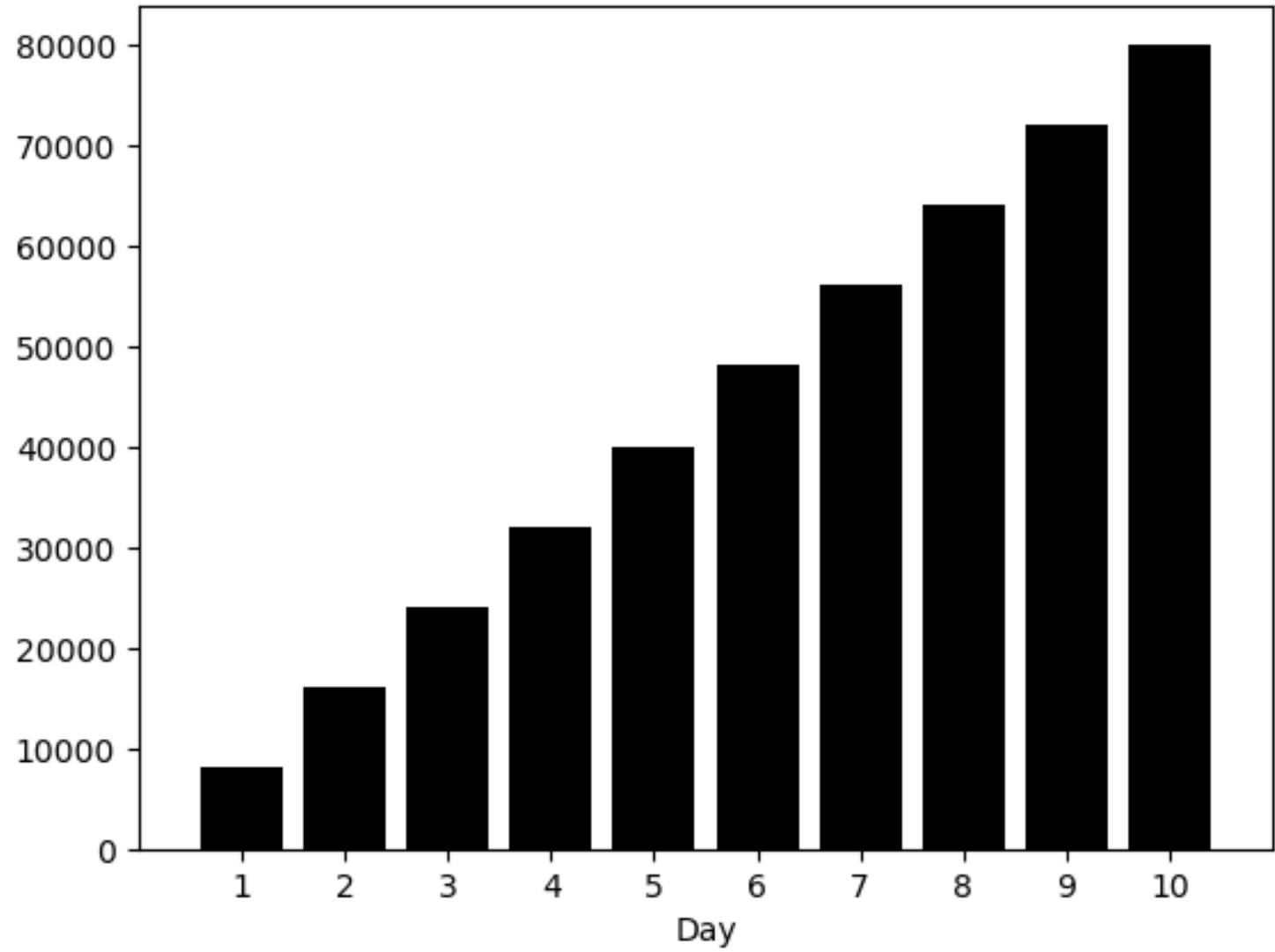
Cumulative sum of profiles within TC domain
