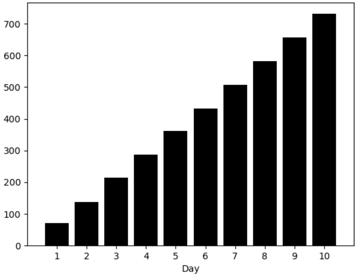
Cumulative sum of profiles at 50 km
