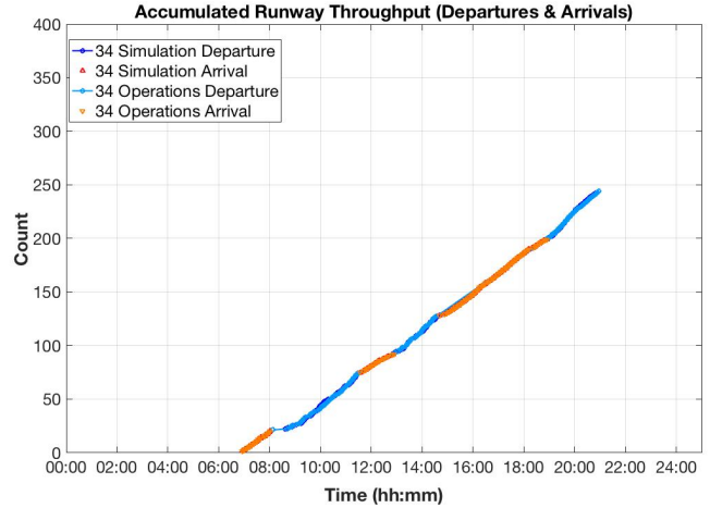
Fig. 7 Accumulated Runway Throughput on 34
