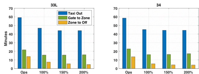
Fig. 14 Mean Taxi Out Times
