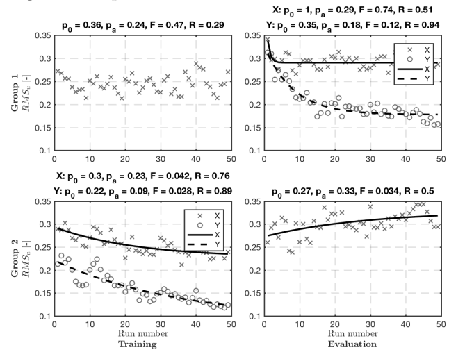
Fig. 6. Pilot control activity.
