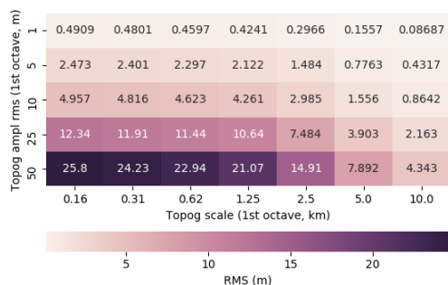
Figure 1: Crossover discrepancy RMS for dataset simulated at MLA measurement epochs in January 2013 with different terrain roughness and no range noise. Real data over the same month show an RMS of \sim 20 m.
