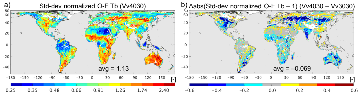
Figure 8. (a) Standard deviation of normalized O-F Tb residuals ( v ) for Vv4030 from April 2015 to March 2018. (b) Difference in the absolute departure of v from unity (Vv4030 minus Vv3030). Blue (red) shading in (b) indicates that v is closer to (farther away from) unity in Vv4030 than Vv3030, that is, blue (red) shading indicates that Vv4030 (Vv3030) is better. Regions with insufficient Tb assimilation coverage for the computation of statistics are shown in white and excluded from the global average calculation.
