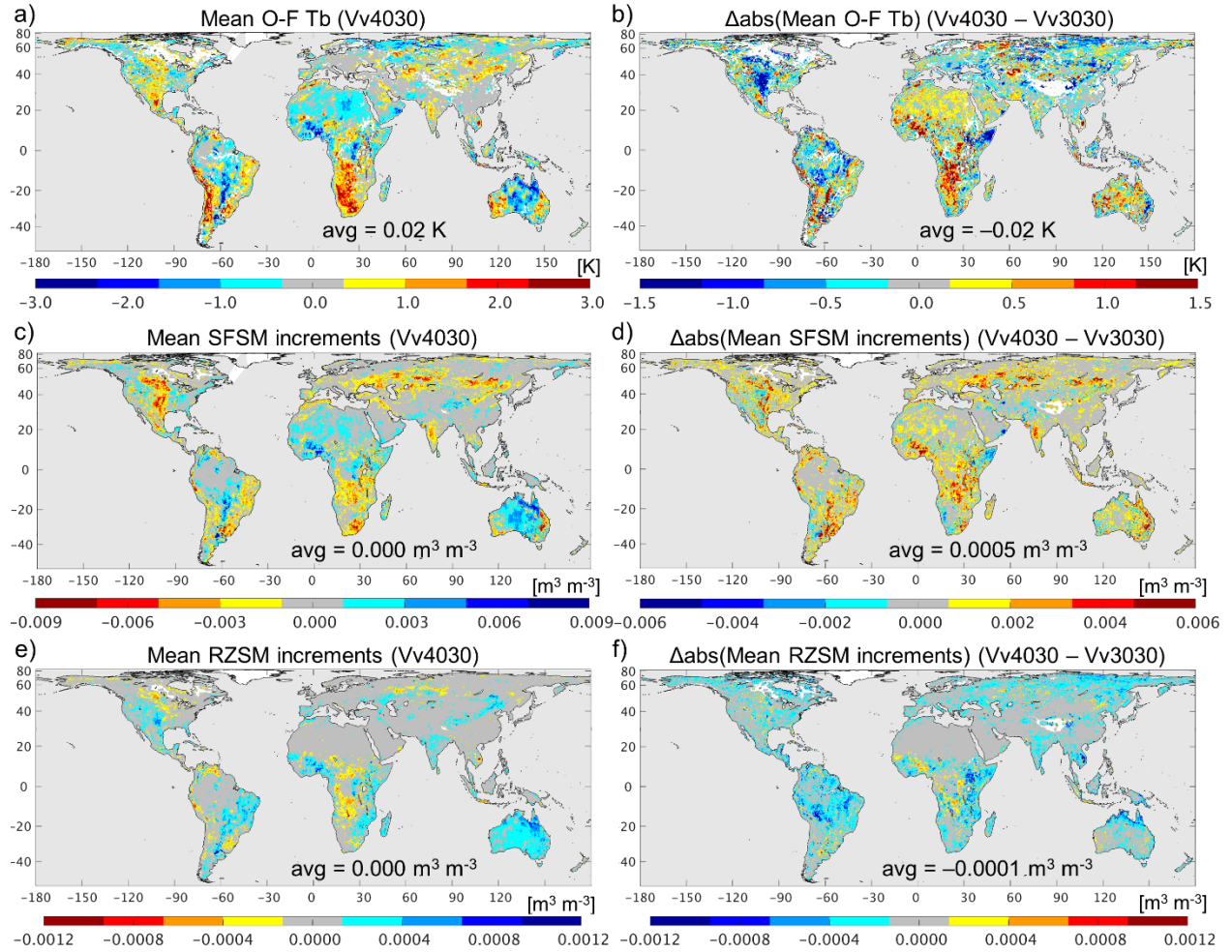
Figure 6. (a,c,e) Mean of Vv4030 assimilation diagnostics. (b,d,f) “Closeness” of Vv4030 and Vv3030 mean assimilation diagnostics to the ideal value of zero, where “closeness” is measured as the Vv4030 minus Vv3030 difference in the absolute value of the mean assimilation diagnostic. Blue (red) colors in (b,d,f) indicate that the Vv4030 (Vv3030) mean diagnostic is better. Assimilation diagnostics include (a,b) O-F Tb residuals, (c,d) surface soil moisture (SFISM) increments, and (e,f) root-zone soil moisture (RZSM) increments for April 2015 to March 2018. Regions with insufficient Tb assimilation coverage for the computation of statistics are shown in white and excluded from the global average calculation.
