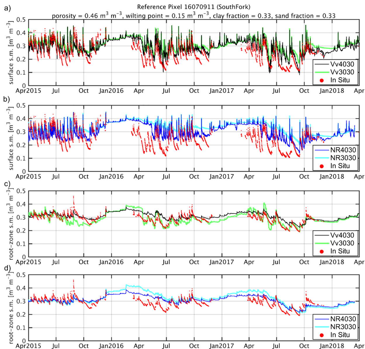
1353 1354 Figure 1. Surface soil moisture at the 9-km South Fork, Iowa, reference pixel #16070911 from 1355 (a) L4_SM estimates (Vv4030 and Vv3030) and (b) Nature Run simulations (NR4030 and 1356 NR3030). In situ measurements are shown identically in both (a) and (b) as red dots. (c,d) As in 1357 (a,b), respectively, but for root-zone soil moisture.
