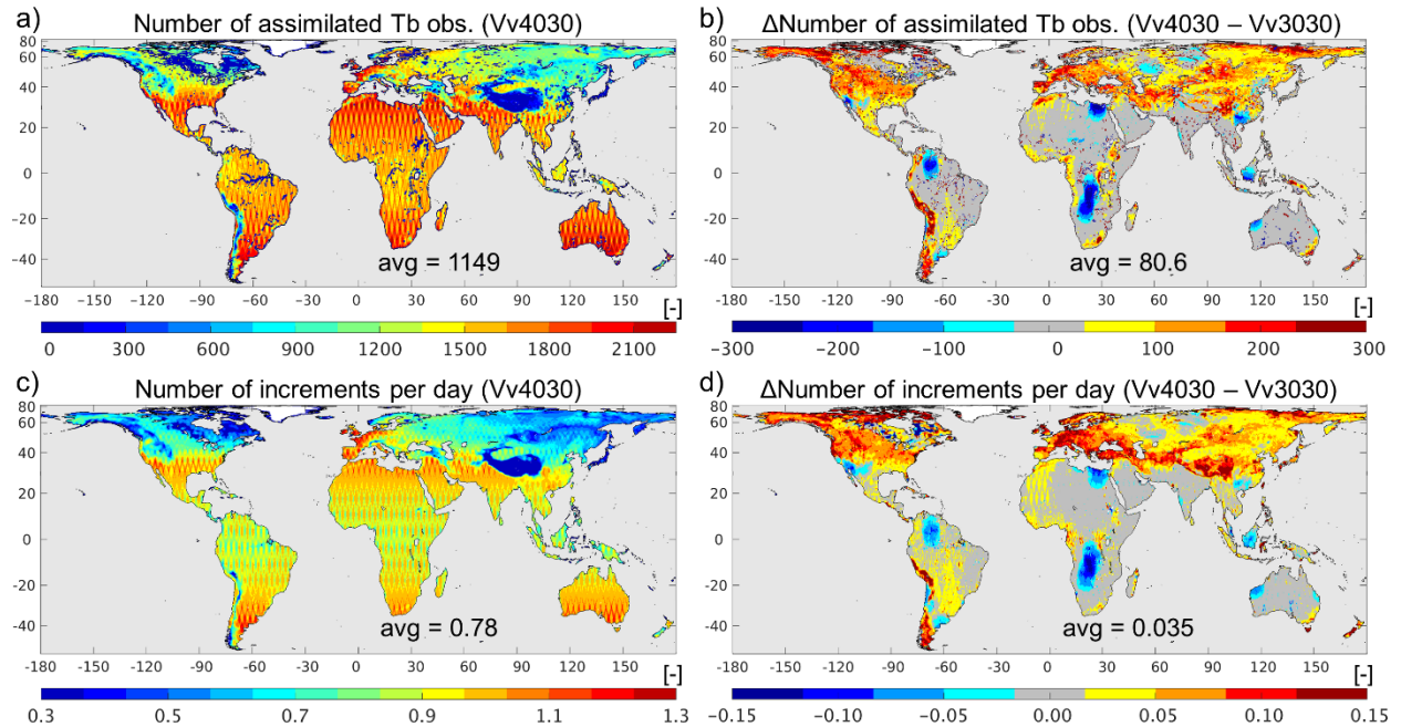
Figure 5. (a) Number of SMAP Tb observations assimilated into Vv4030 from April 2015 to March 2018. Data counts include horizontal- and vertical-polarization data from ascending and descending half-orbits. (b) Difference in number of assimilated observations (Vv4030 minus Vv3030). (c) Average number of increments per day generated in Vv4030 from April 2015 to March 2018 (applies equally to surface and root-zone soil moisture increments). (d) Difference in number of increments (Vv4030 minus Vv3030). Global averages computed over all land excluding glaciated and open water surfaces.
