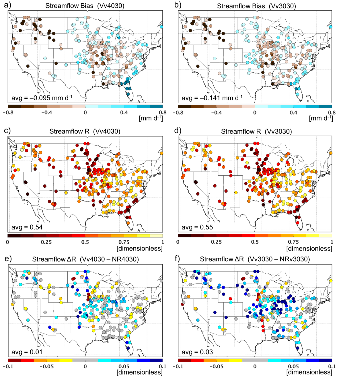
Figure 4. June – September 2015-2017 runoff skill versus USGS streamflow measurements in 239 U.S. basins for (a,c,e) Vv4030 and (b,d,f) Vv3030. (a,b) Bias and (c,d) R values of the L4_SM product. (e,f) Difference in R values between the L4_SM product and the corresponding Nature Run data. Blue (red) colors in (e,f) indicate that the L4_SM estimates are better (worse) than Nature Run estimates.
