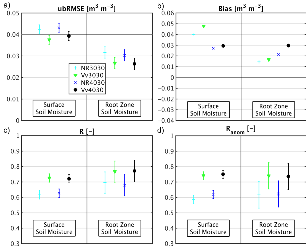
Figure 2. (a) ubRMSE ( \text{m}^3 \text{m}^{-3} ), (b) bias ( \text{m}^3 \text{m}^{-3} ), (c) R (dimensionless), and (d) anomaly R (dimensionless) for Nature Run and L4_SM estimates of surface and root-zone soil moisture versus core validation site measurements, averaged across all 9-km reference pixels. Error bars for ubRMSE, R, and anomaly R indicate 95% confidence intervals (section 3.1). The thick horizontal line in (a) represents the L4_SM accuracy requirement of \text{ubRMSE} \leq 0.04 \text{ m}^3 \text{m}^{-3} .
