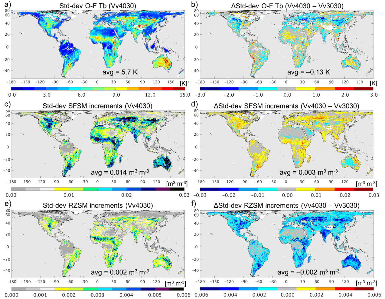
Figure 7. (a,c,e) Standard deviation of Vv4030 assimilation diagnostics and (b,d,f) difference in standard deviation of assimilation diagnostics (Vv4030 minus Vv3030). Assimilation diagnostics include (a,b) O-F Tb residuals, (c,d) surface soil moisture (SFSM) increments, and (e,f) root-zone soil moisture (RZSM) increments for April 2015 to March 2018. Regions with insufficient Tb assimilation coverage for the computation of statistics are shown in white and excluded from the global average calculation.
