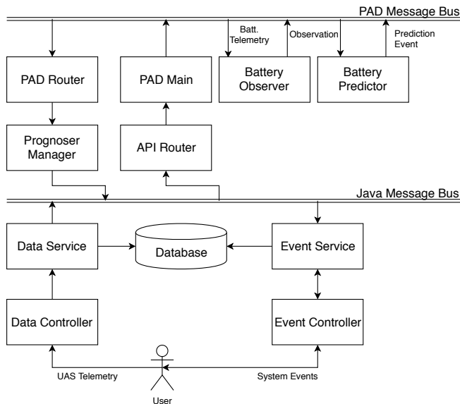
Figure 2. A simplified representation of the PaaS communication bus. A new PAD is created for each prognostic session. After initialization, the PAD's main function enters an infinite loop that reads messages from stdin until an "exit" message is received. During initialization, the PAD creates a Router object that intelligently subscribes to messages that need to be transferred to the front-end.
