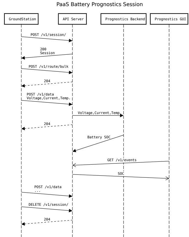
Figure 3. The sequence of requests to do battery prognostics using PaaS. The client is split into two parts: a ground station that communicates data from the vehicle, and a separate GUI to display results. The ground station first initiates the session with a POST request. The server responds with a session ID that is included in all future requests for that session. The ground station next sends the vehicle's flight plan, and then starts sending battery sensor data. This data is sent continuously throughout the flight. Upon receiving a set of battery data, PaaS computes the battery state of charge and stores it. The GUI periodically polls PaaS to request updated battery SOC. Once the flight is complete, the ground station sends a DELETE request to terminate the session.
