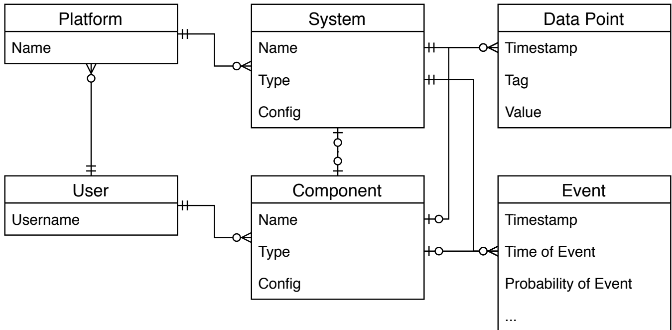
Figure 1. A simplified representation of PaaS entities. These entities represent the user’s conceptual view of the service. They map closely to the database entities used to store data used by the service. The Platform entity maps to a GSAP process, a System/Component pair map to a prognoser and Data Points and Events map to individual messages passed within the service.
