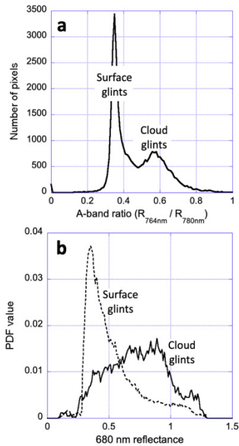
Fig. 2. Marine ice cloud glints appear ubiquitous and relatively bright: statistics of glint A-band ratios and reflectance values in a yearlong data set of EPIC images. (a) Histogram of the oxygen A-band ratio of red glints over the ocean. (b) PDF of red glint reflectance. The median 680-nm (red channel) reflectance for cloud and surface glints is 0.82 and 0.54, while the mode values are 0.89 and 0.35, respectively. Both panels consider all oceanic locations with glint angles <1.5^\circ .
