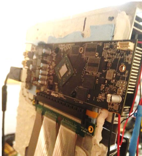
Figure 3: AMD e9173 on Cold Block aligned in beam at MGH
