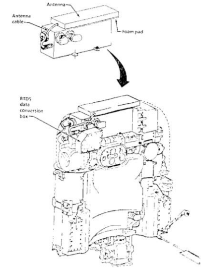
EMU Antenna
