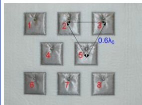
fabric array antenna
