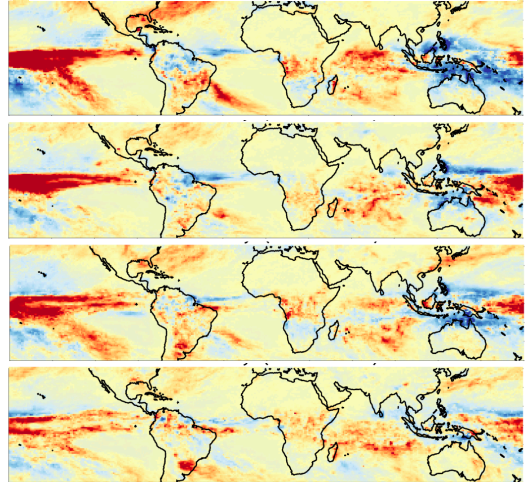
Bias-corrected Forecast Precip. Anomaly
