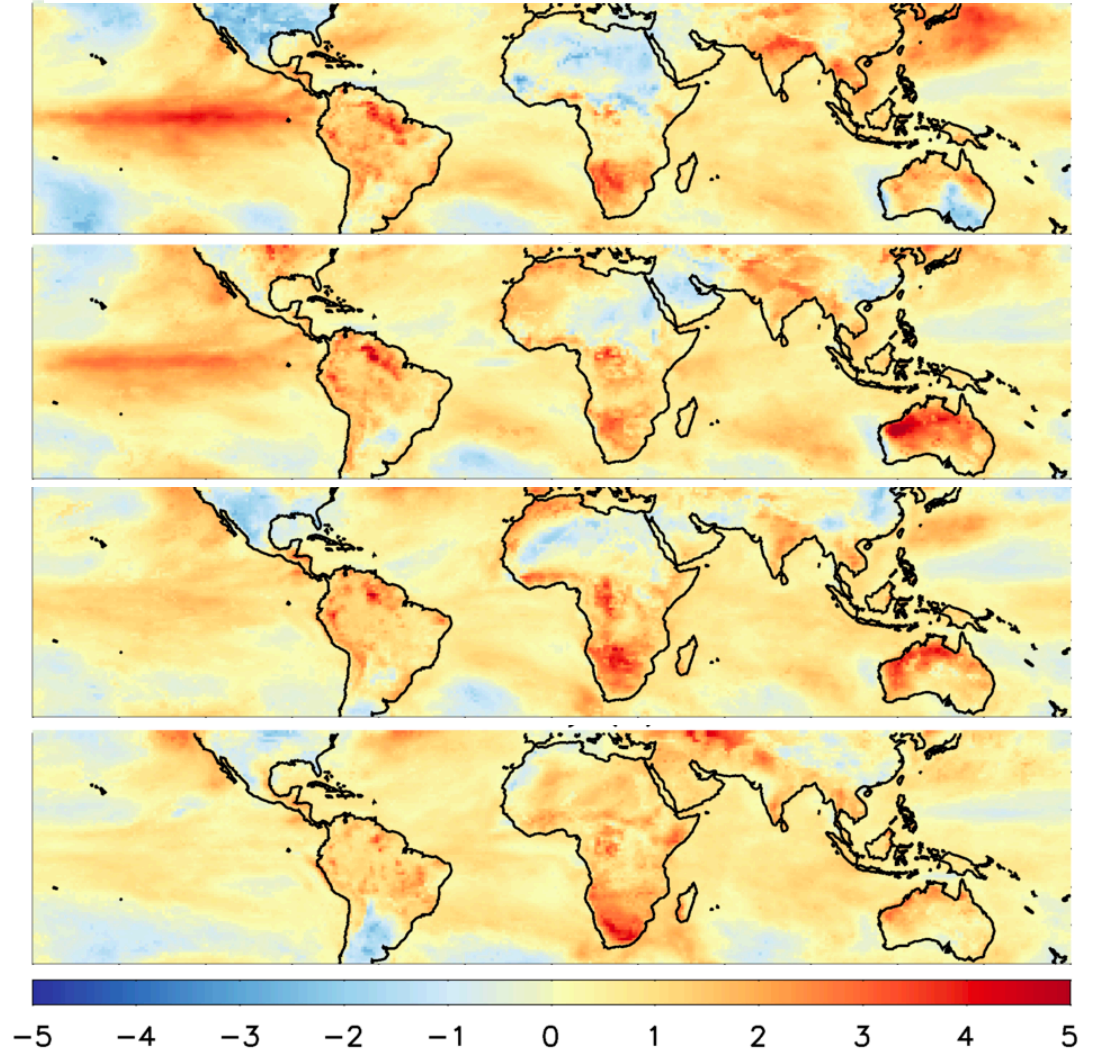
Bias-corrected Seasonal Forecast Anomaly
