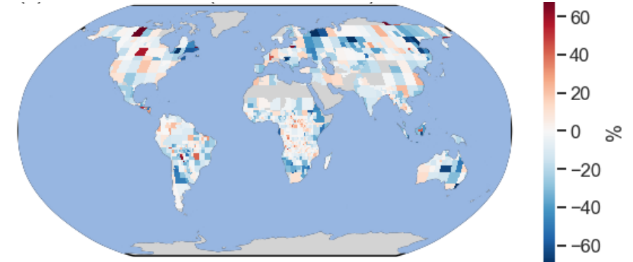
RMSE changes from Clim to OCIVPDAR model
