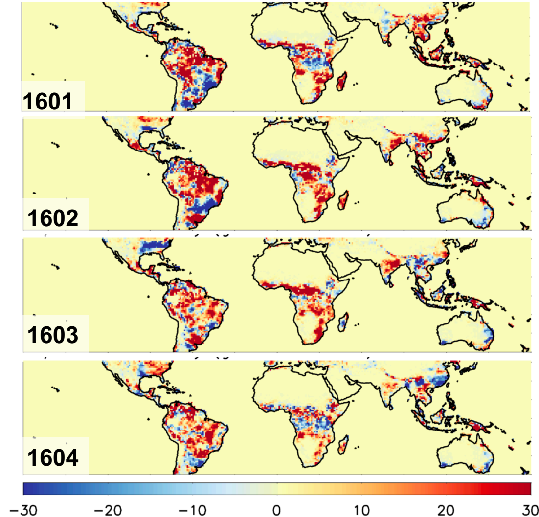
Observation-driven NEE Anomaly (g C m -2 mon -1 )
