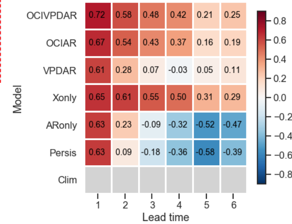
RMSE changes from Clim to OCIVPDAR model
