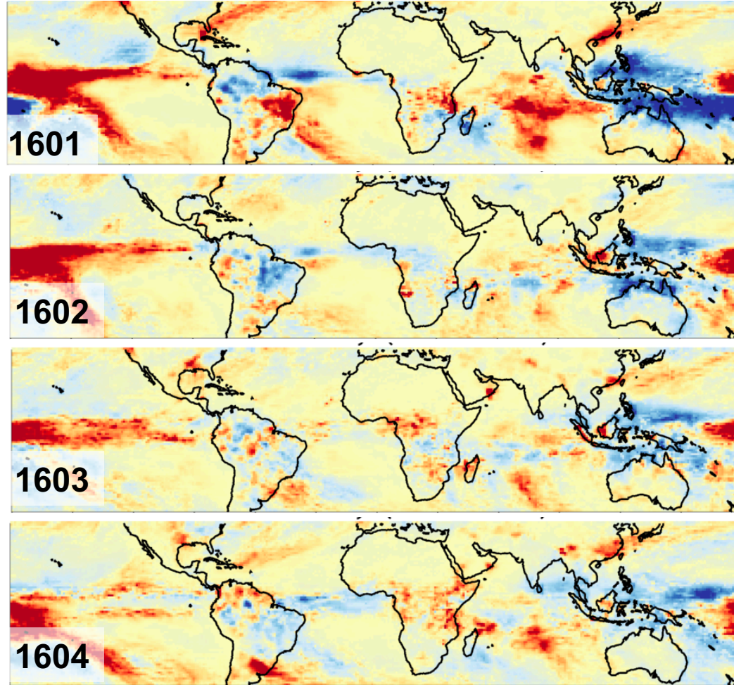
Observation-driven Precip. Anomaly (mm mon -1 )
