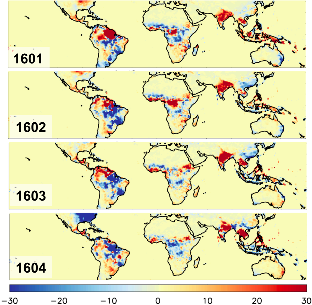
Observation-driven NEE Anomaly (g C m -2 mon -1 )
