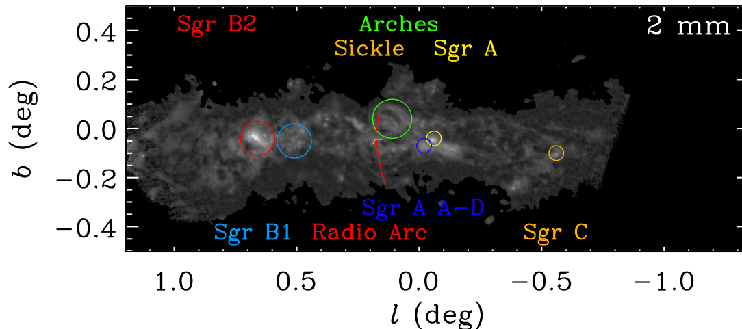
Figure 1. Features in the central molecular zone. Originally defined from longer wavelength radio observations, these features are notable 2 mm sources as well. See Figure 4 for an unadorned version of the 2 mm image.
