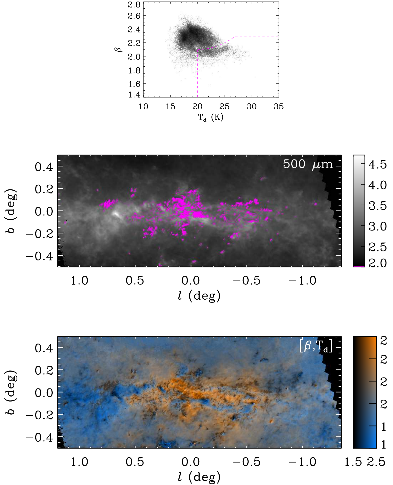
Figure 7. The top panel shows a scatter plot between T_d and \beta for all pixels shown in Figure 5. There is no tight correlation between these parameters, although there is the loose trend that regions with high temperatures are likely to have relatively low values of \beta . The magenta line separates a branch of points with high T_d and low \beta whose locations are marked in magenta on the 500 \mu\text{m} image in the second panel. The bottom panel shows the simultaneous distribution of T_d and \beta , encoding T_d with color from blue (cold) to orange (warm) and \beta with brightness from low (dark) to high (light) (cf. Fig. 5).
