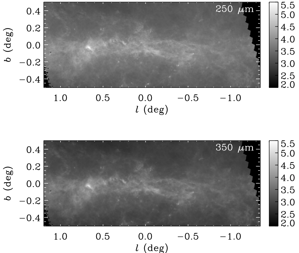
Figure 3. Herschel SPIRE 250 (top) and 350 \mu\text{m} (bottom) images from the Hi-GAL survey (Molinari et al. 2016). These are displayed on a logarithmic scale spanning [100, 3.5 \times 10^5] \text{MJy sr}^{-1} . The 250 \mu\text{m} image is convolved to the 21'' resolution of the GISMO 2 mm data. Emission is dominated by cool dust ( T_d \approx 19 K, see Figure 6).
