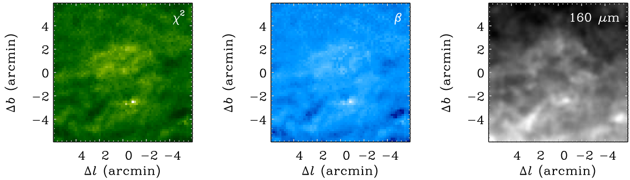
Figure 10. Magnified images of an unusual circular structure as revealed by fitting deviations ( \chi^2 ), emissivity index ( \beta ), and 160 \mu\text{m} emission (left to right). The structure is centered at (l, b) = (359.65, +0.18) . The structure seems to be largely defined by unusual dust properties (See Section 3.1).
