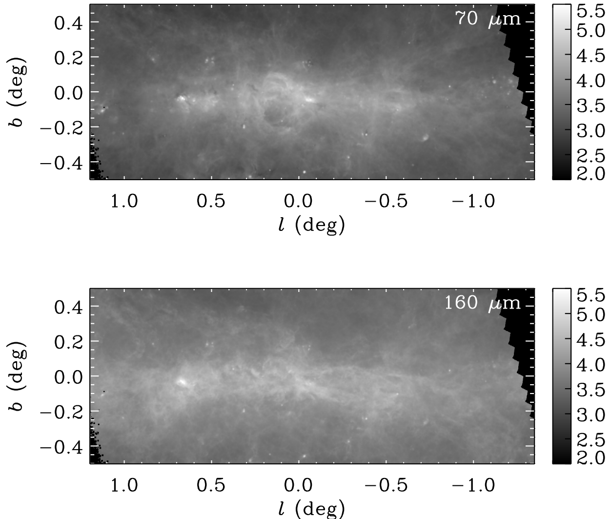
Figure 2. Herschel PACS 70 (top) and 160 \mu\text{m} (bottom) images from the Hi-GAL survey (Molinari et al. 2016). These are displayed on a logarithmic scale spanning [100, 3.5 \times 10^5] \text{MJy sr}^{-1} . These images are convolved to the 21'' resolution of the GISMO 2 mm data. Emission is dominated by cool dust ( T_d \approx 19 K, see Figure 6), but warmer dust components ( T_d up to 30 K) in compact and extended H II regions are evident at 70 \mu\text{m} .
