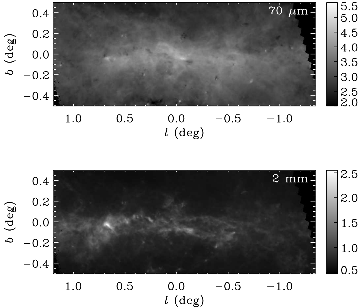
Figure 11. Images of 70\ \mu\text{m} (top) and 2\ \text{mm} (bottom) emission extrapolated from the fixed \beta = 2.25 model of the 160\text{--}500\ \mu\text{m} emission. The data are convolved to 37'' resolution. These images are visually similar to the observed intensities shown in Figures 2 and 4, and are shown on the same logarithmic display ranges.
