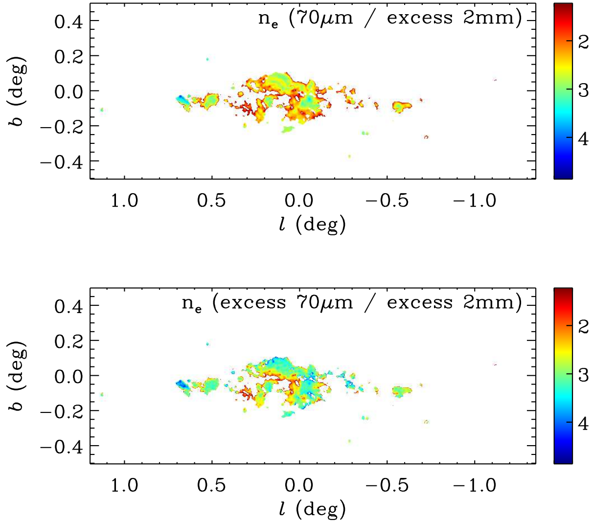
Figure 15. Maps of the logarithm of the electron density, \log(n_e) , implied by the ratio of residual 2 mm emission (mostly free-free) to 70\mu\text{m} emission without (top) and with (bottom) subtraction of the emission of cold dust extrapolated from longer wavelengths. The latter case better isolates dust emission from warm regions where free-free emission is more likely to arise, and results in derived n_e values that are less correlated with the 70\mu\text{m} brightness. The color scale for \log(n_e) is the same as in Figure 14.
