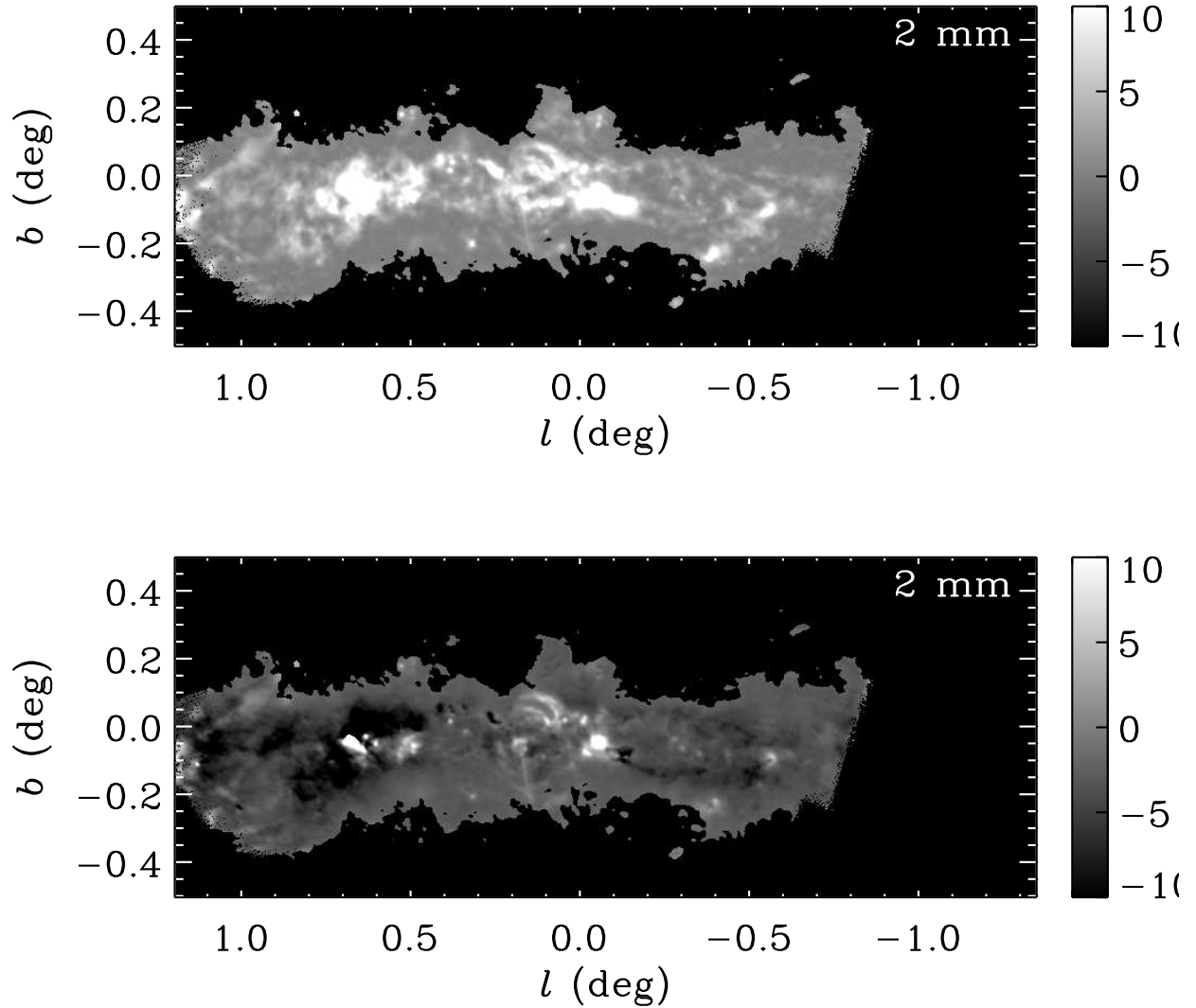
Figure 13. The observed 2 mm intensity (top) displayed on a linear grayscale range of [-10,10] \text{MJy sr}^{-1} , and the difference (bottom) between the observed and extrapolated 2 mm intensities on the same display range ( 37'' resolution). The difference image shows that most of the 2 mm emission is associated with thermal emission from dust. In regions where T_d is low, the emission is sometimes over-subtracted (appearing dark). Regions exhibiting 2 mm emission in excess of the dust emission (bright in the difference image) are H II regions and ionized structures that radiate via free-free emission at radio wavelengths, and non-thermal emission from the central filament of the Galactic center Radio Arc.
