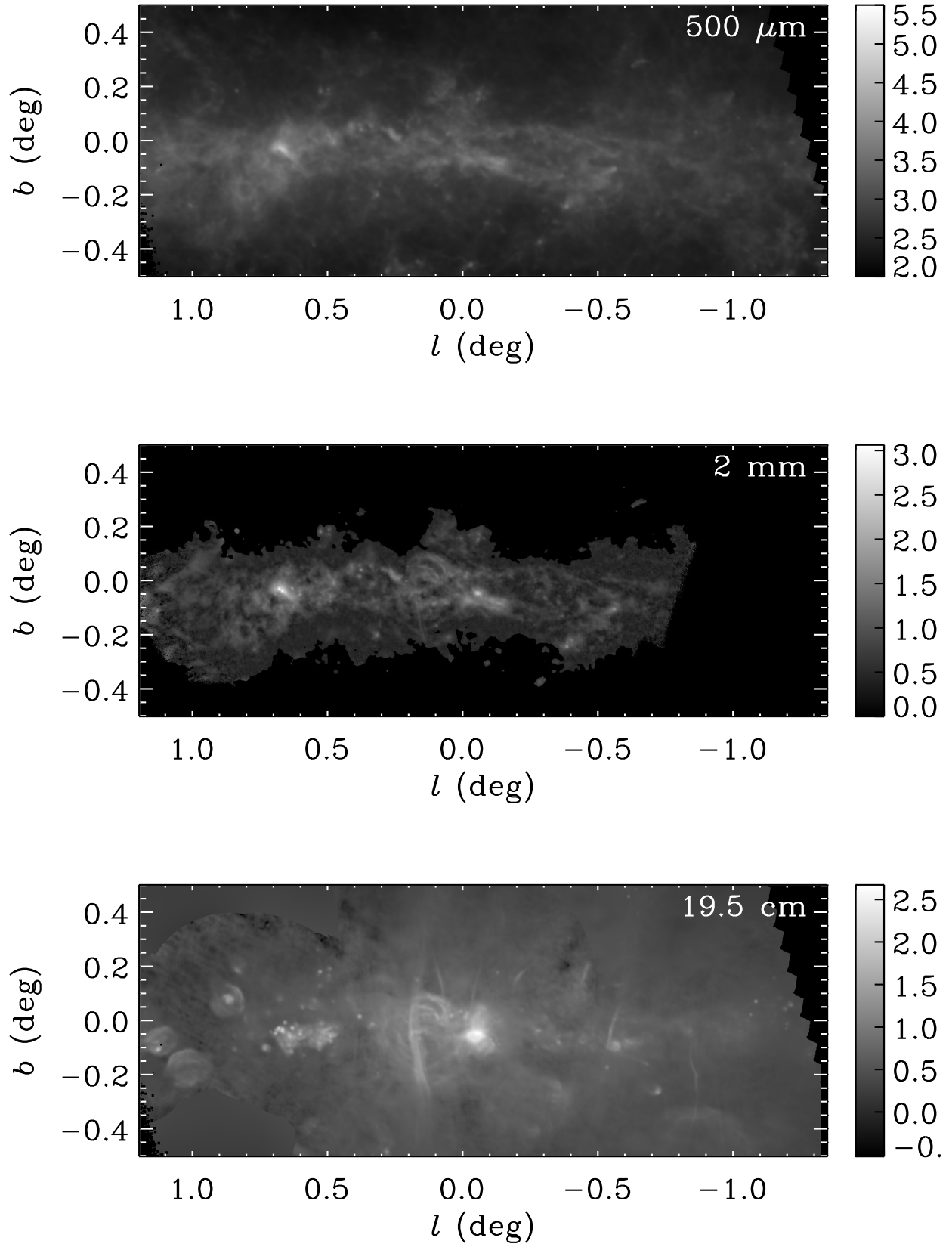
Figure 4. (top to bottom) SPIRE 500\ \mu\text{m} , GISMO 2\ \text{mm} and VLA 19.5\ \text{cm} images of the Galactic center region. These are displayed on a logarithmic scale spanning [100, 3.5 \times 10^5] , [1, 1150] , and [0.3, 470] \text{MJy sr}^{-1} respectively (an offset of +3\ \text{MJy sr}^{-1} is applied to the 2\ \text{mm} image to avoid truncating the negative noise variations of the background). The 19.5\ \text{cm} image exhibits both thermal (free-free) and non-thermal (synchrotron) sources. The 2\ \text{mm} image shows features in common with both longer and shorter wavelength images.
