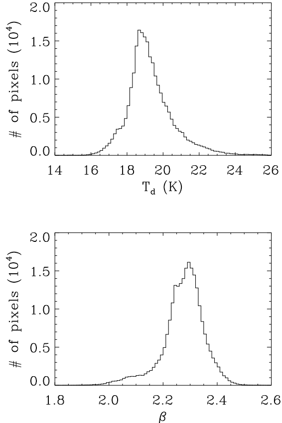
Figure 6. Histograms of the derived T_d (top) and \beta (bottom) for each pixel derived using the model in which both are free parameters (See Figure 5). The mean and median values of \beta are 2.27 and 2.28. Based on this distribution, we used a fixed \beta = 2.25 for subsequent models.
