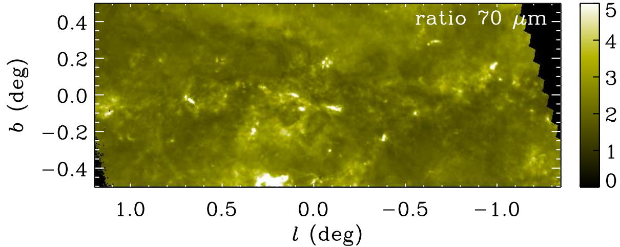
Figure 12. Ratio of observed to extrapolated 70 \mu\text{m} intensities (from Figures 2 and 11). The linear grayscale range is [0,5] . White regions, where the observed 70 \mu\text{m} intensity is significantly greater than the extrapolated intensity, include star-forming regions with warm dust and, prominently, cold molecular clouds and IRDCs.
