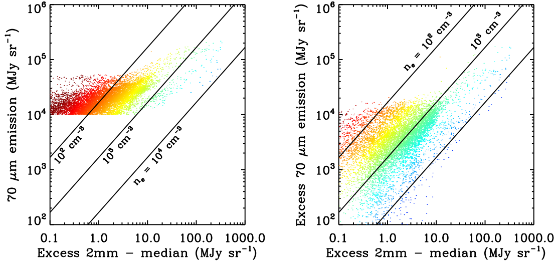
Figure 14. Ratio of residual 2 mm emission (mostly free-free) to 70 \mu m emission without (left) and with (right) subtraction of the emission of cold dust extrapolated from longer wavelengths. The points are shaded as a function of n_e , with several lines of constant density overplotted for guidance.
