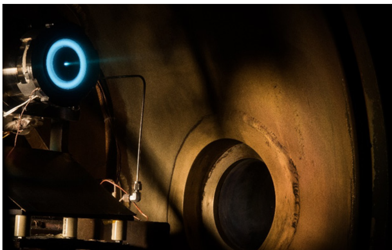
Figure 22.—NASA-H64M-LMW operating in VF-8.
