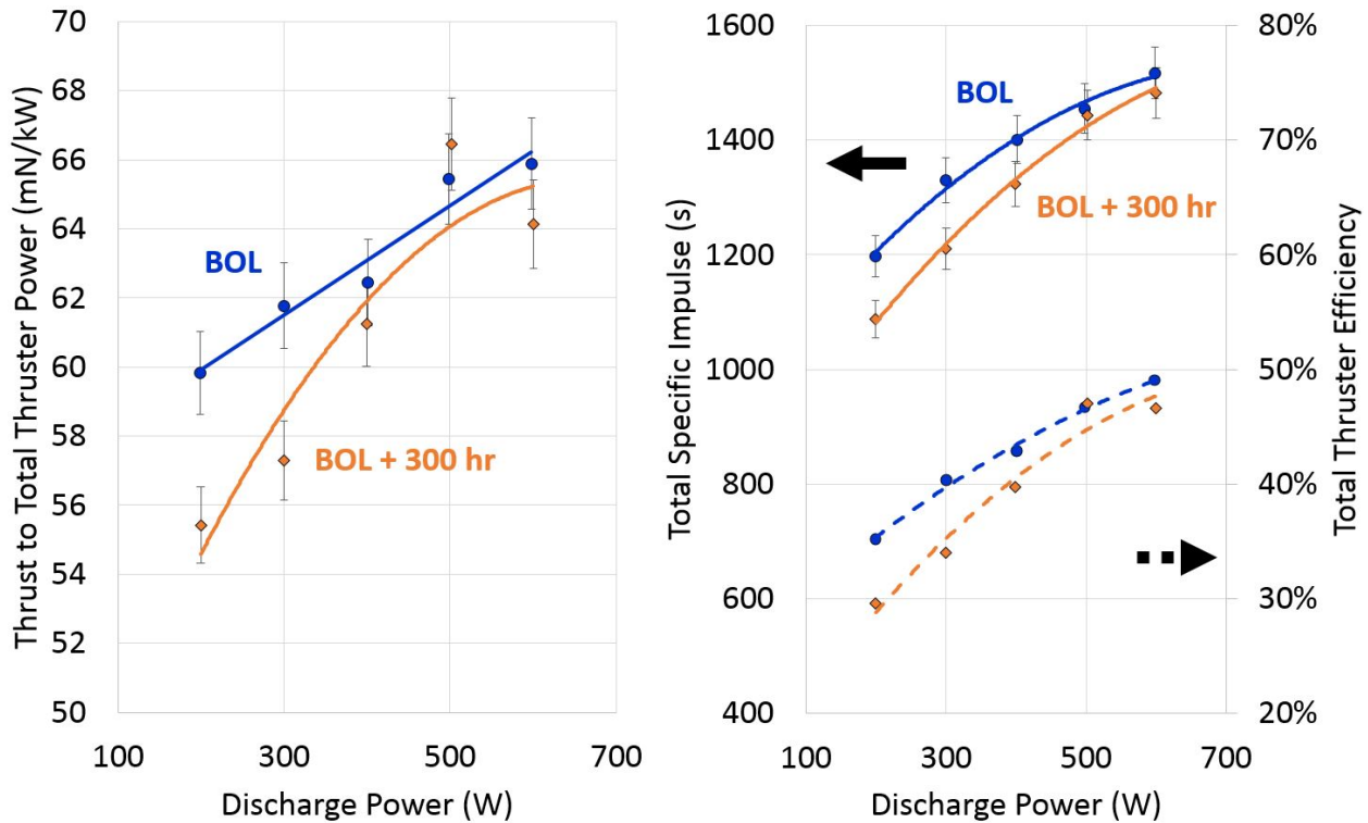
Figure 20.—Comparison of NASA-H64M-LM performance at BOL versus BOL + 300 hr for 300-V discharge voltage, identical magnetic field settings, 7 percent cathode flow fraction, and electrically floating configuration. The total thruster efficiency uncertainty bars (up to a maximum of \pm 5 percent) are not shown for clarity.
