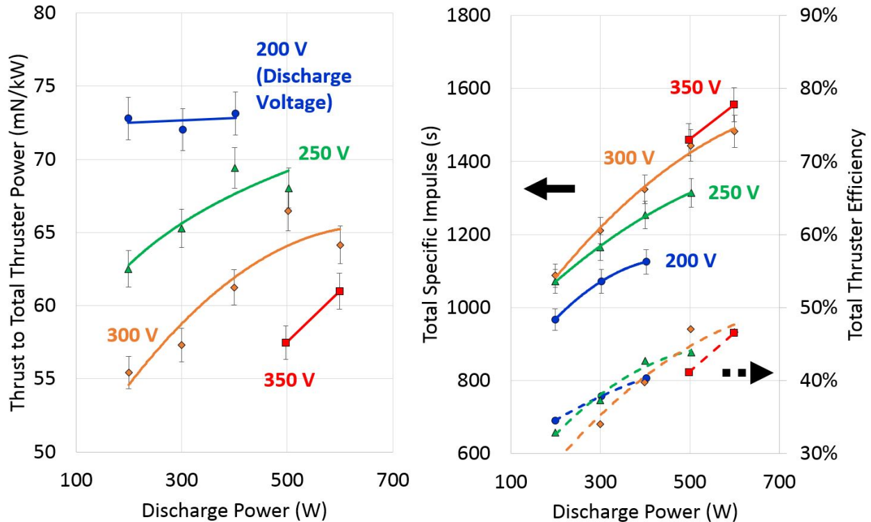
Figure 19.—NASA-H64M-LM performance at BOL + 300 hr with the same magnetic field settings as the results in Figure 18, 7 percent cathode flow fraction, and electrically floating configuration. The total thruster efficiency uncertainty bars (up to a maximum of \pm 5 percent) are not shown for clarity.
