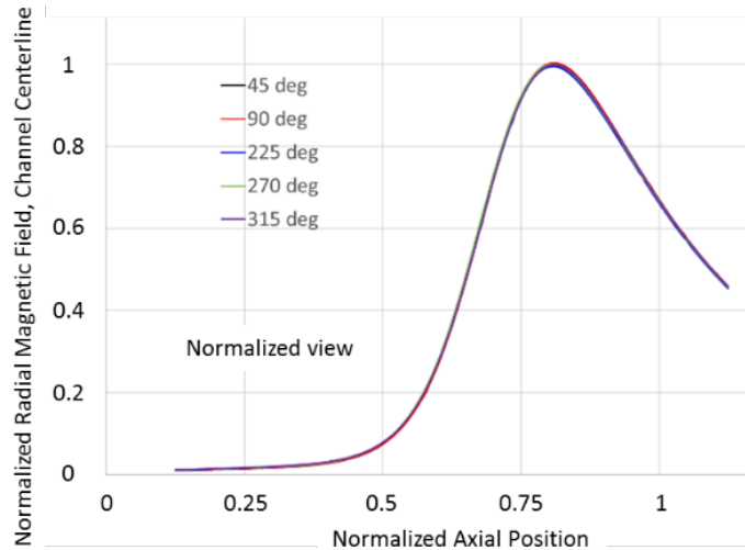
Figure 5.—Channel centerline magnetic mapping results at various azimuthal angles for the NASA-H64M-LM thruster.
