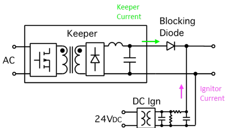
Figure 13.—Schematic of cathode keeper ignitor configured in parallel with the cathode keeper supply output.
