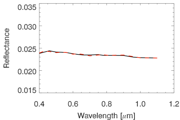
Fig 1: An example of a best-fit model spectrum (red dashed) to an observed OVIRS spectrum (black line) over an area centered at 204.6°E and 8.7°N.
