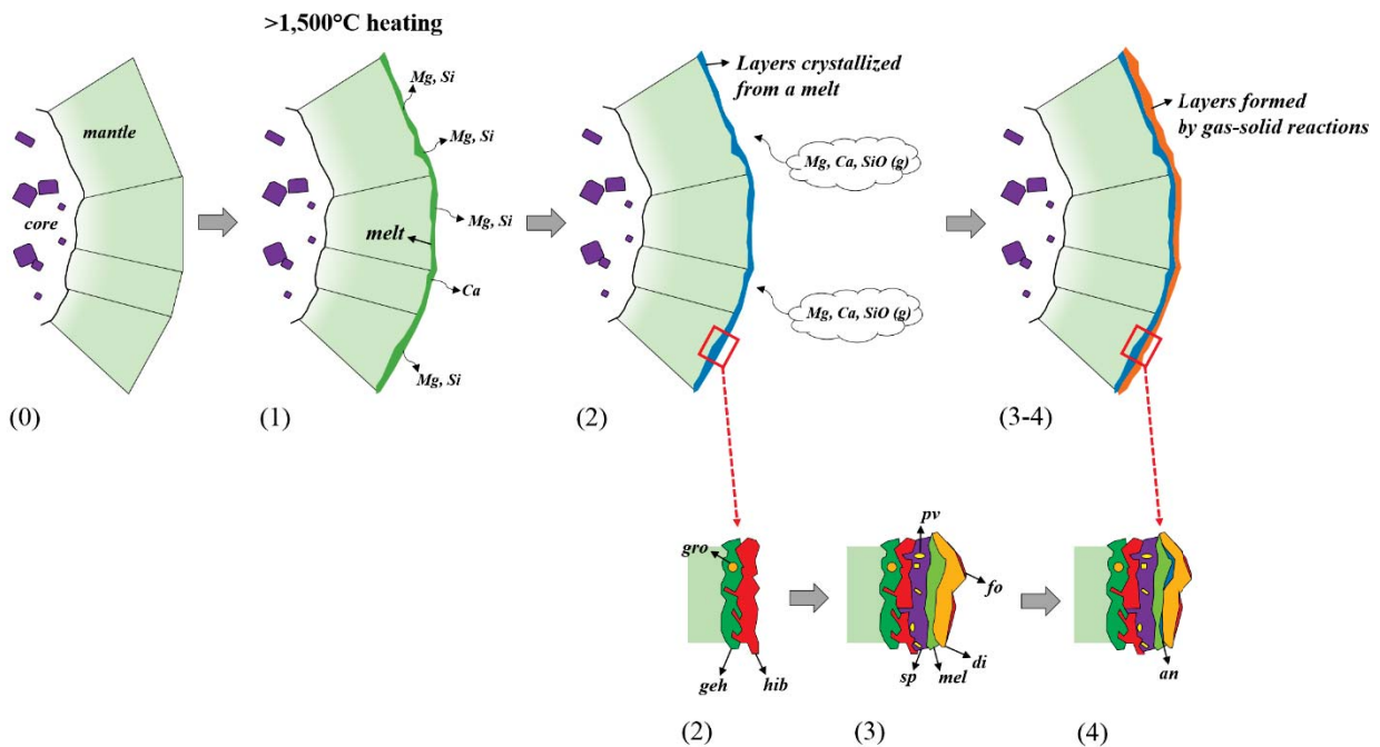
Figure 10. Schematic scenario for the WL rim formation on the Vigarano CAI Big Guy . The formation sequence of the WL rim is described as follows: (0) formation of the host CAI; (1) formation of a Ca,Al-rich melt layer by flash heating and extensive evaporation of Mg, Si, and possibly Ca; (2) crystallization of gehlenite, hibonite, and rare grossite; (3) sequential gas-solid reactions to form spinel, perovskite, melilite, diopside, and forsterite; and (4) parital replacement of melilite and Al-diopside by anorthite.
