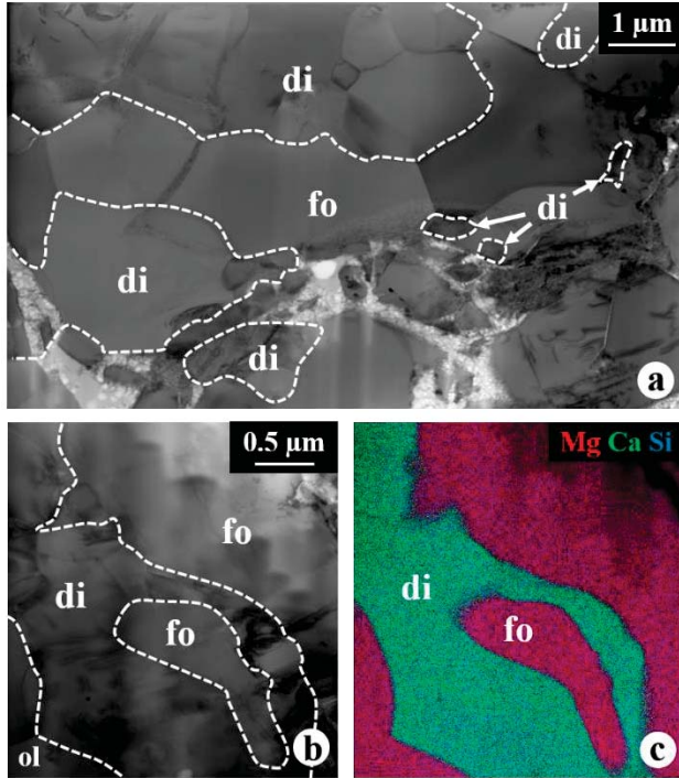
Figure 7. Oxygen isotopic compositions of individual minerals from the Vigarano CAI Big Guy . The data are plotted on an oxygen three-isotope diagram ( \delta^{17}\text{O} vs. \delta^{18}\text{O} ) in (a) and as deviations from the terrestrial fractionation line ( \Delta^{17}\text{O} ) in (b). The terrestrial fractionation (TF) and carbonaceous chondrite anhydrous mineral (CCAM) lines are shown for reference.
