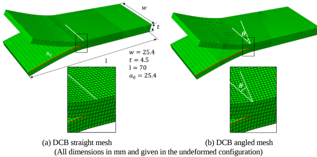
Figure 6. DCB models used. Element size in refined region: el_{size} = 0.5 mm.
