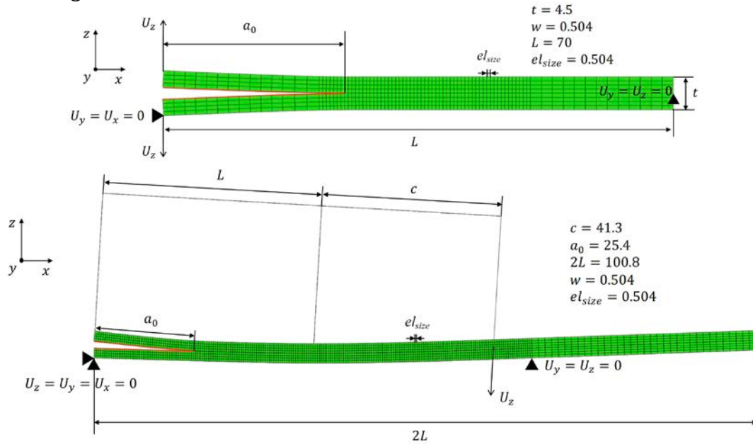
Figure 8 DCB and MMB models. 3D models, with one element along the width.
