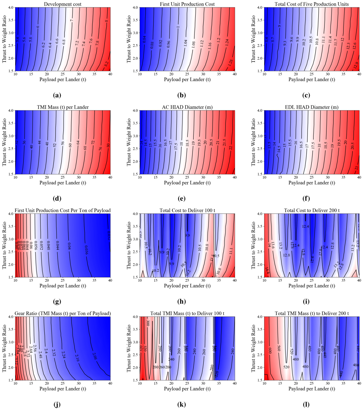
Fig. 14 Payload vs. Thrust to Weight Ratio Trades.
