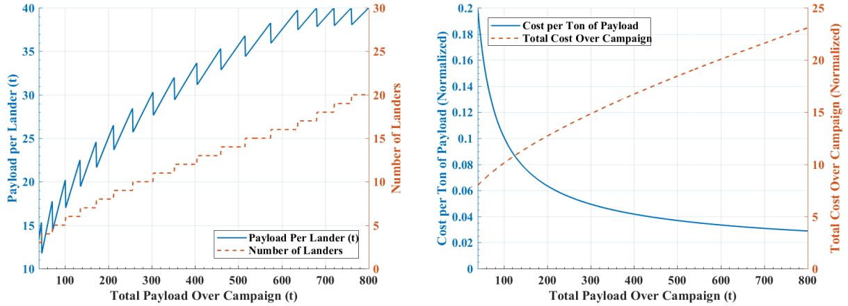
(a) Payload per lander and number of landers to minimize lander hardware costs over a campaign. (b) Total lander hardware cost over campaign and hardware costs per ton of payload delivered.
