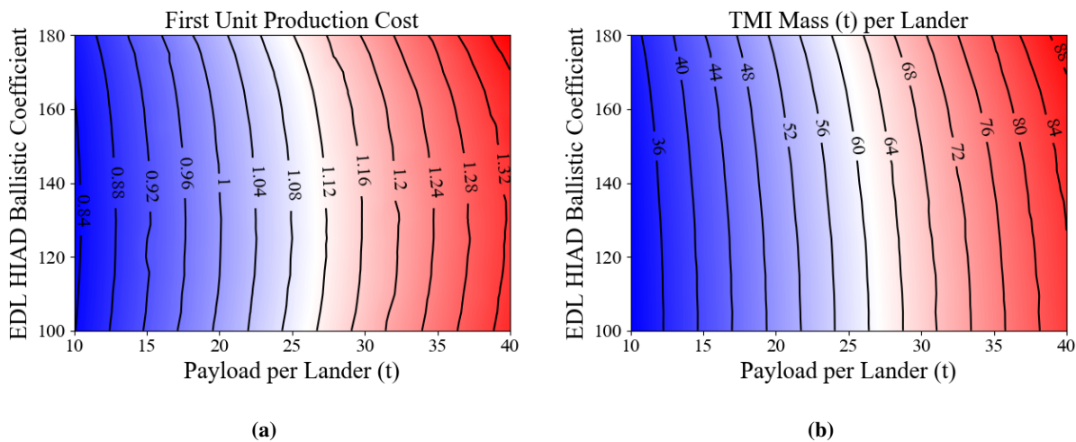
Fig. 8 Lander payload and EDL HIAD ballistic coefficient tradespace entering from 1 Sol orbit.
