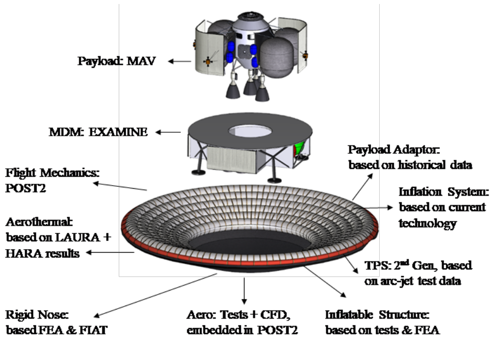
Fig. 1 HIAD entry system models used by SAPE.
