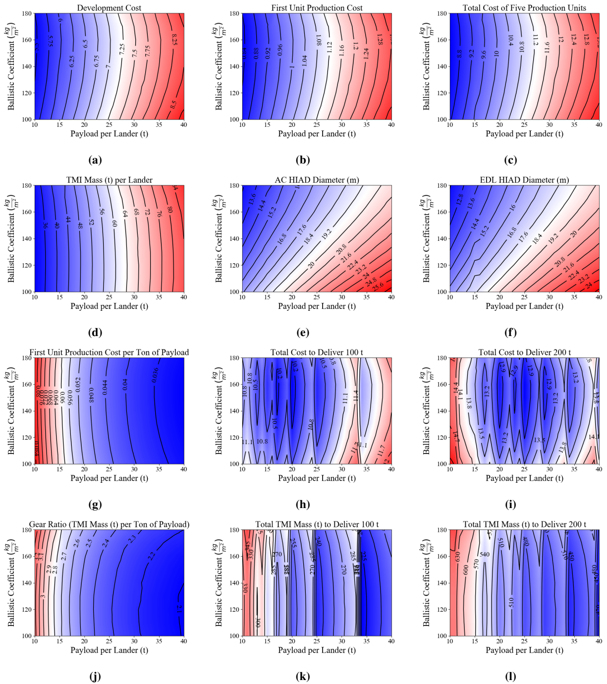
Fig. 4 Payload vs. Ballistic Coefficient Trades.
