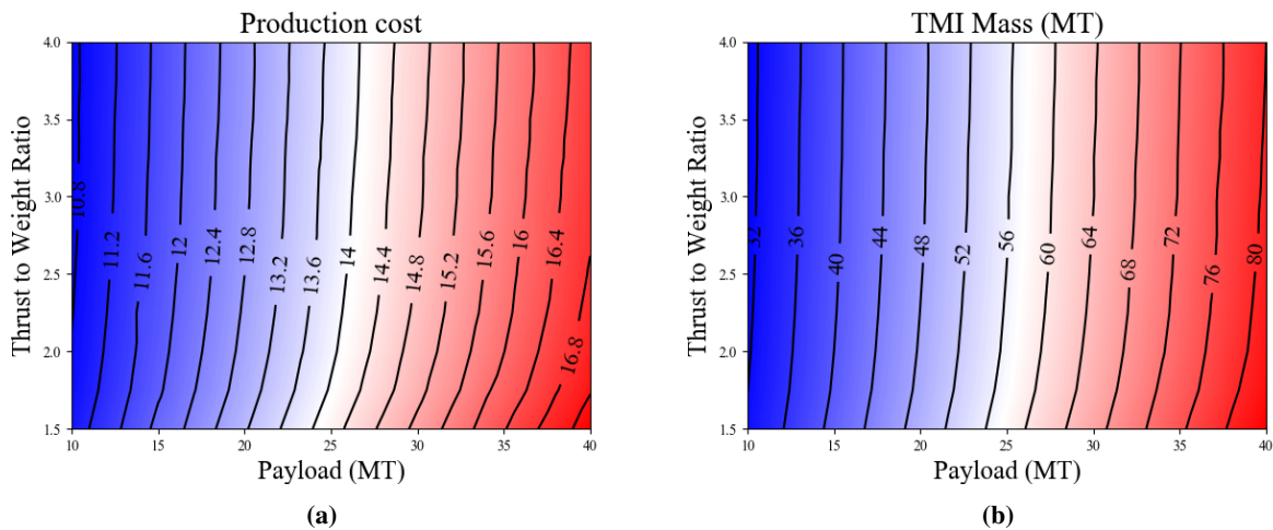
Fig. 10 Lander payload and thrust to weight ratio tradespace entering from 1 Sol orbit.
