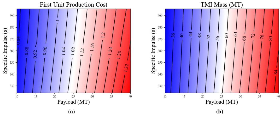
Fig. 9 Lander payload and specific impulse tradespace entering from 1 Sol orbit.
