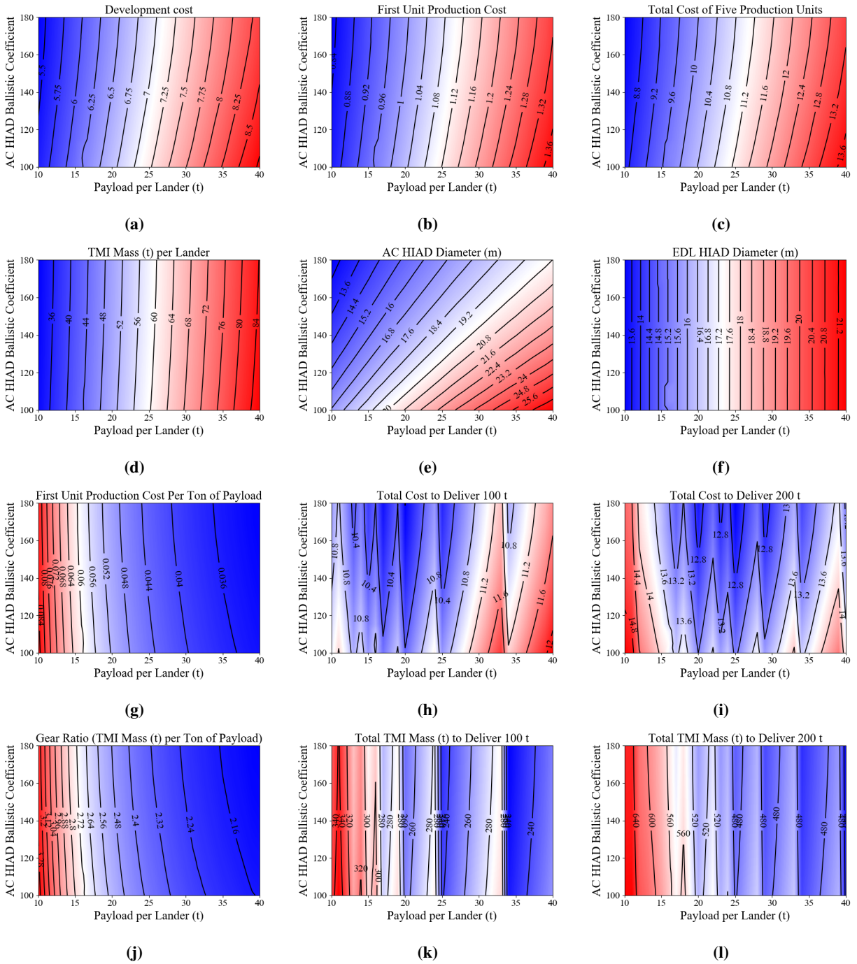
Fig. 11 Payload vs. Aerocapture HIAD Ballistic Coefficient Trades.
