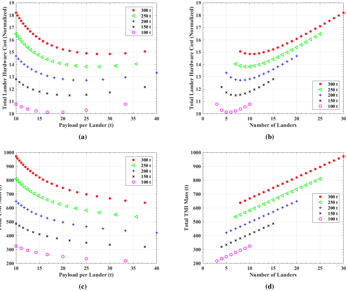
Fig. 5 Effects of lander payload on total cost and TMI mass for several possible multi-mission Mars campaigns.
