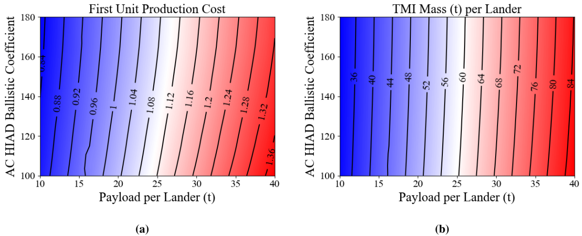
Fig. 7 Lander payload and aerocapture HIAD ballistic coefficient tradespace entering from 1 Sol orbit.
