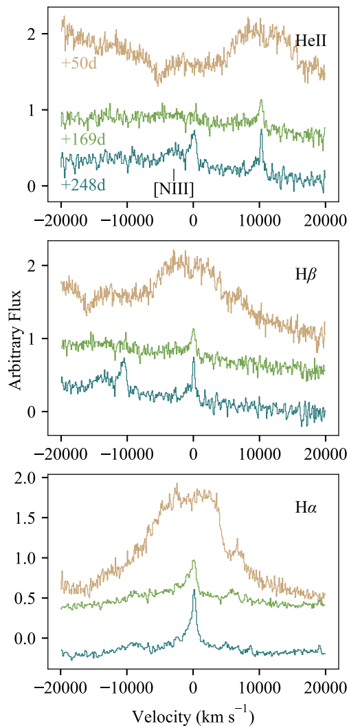
Figure 8. Velocity profiles of He II \lambda 4686 , H\beta and H\alpha of AT2018zr at \Delta t = 50 , 169, and 248 days. Narrow H\alpha , H\beta , and He II \lambda 4686 emission emerged 6 months after maximum light. The narrow line widths are on the order of 1000 \text{ km s}^{-1} , which is only \sim 10\% of the broad Balmer line widths from earlier epochs. We note that on day 50, H\alpha and H\beta have a similar velocity profile that is dented on the red wing, which is likely to arise from the geometry of the line-forming region.
