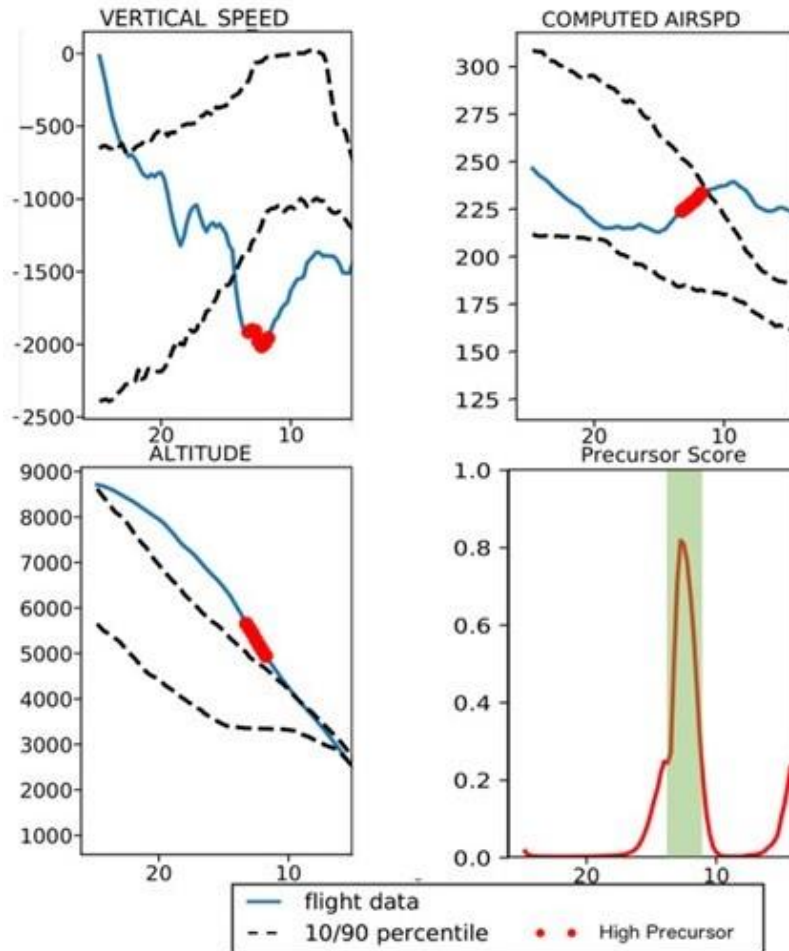
Figure 3.4.1-2. Time series plots for vertical speed, altitude, computed airspeed, and precursor score are depicted for a flight in which a preemptive action (i.e., slowing descent rate) was taken to avoid a high-speed exceedance at 1000 ft.
