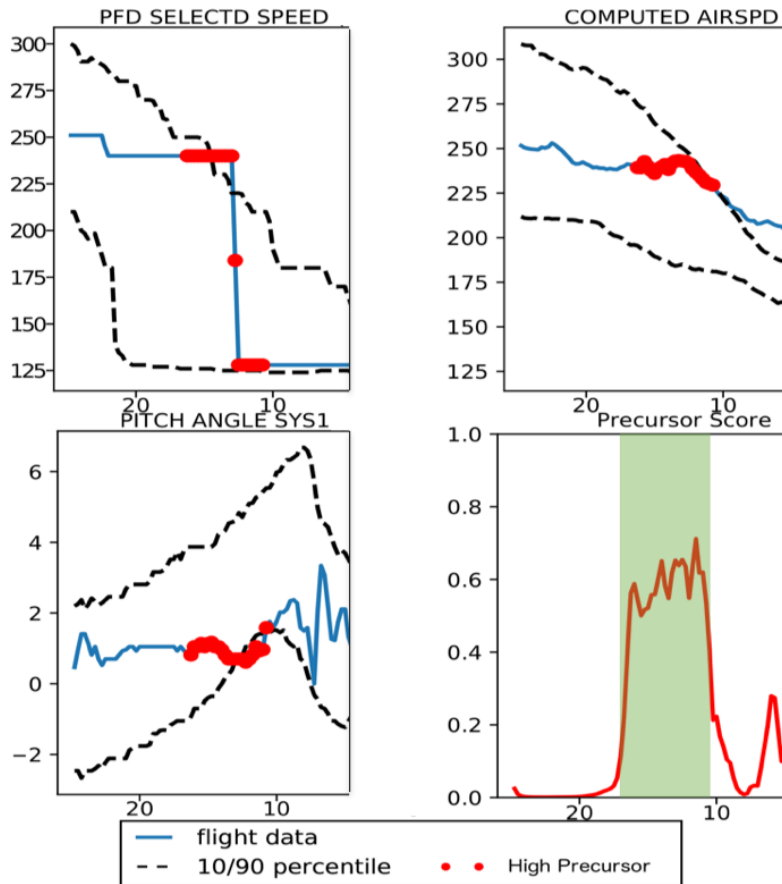
Figure 3.4.1-1. Time series plots for PFD selected speed, pitch angle, computed airspeed, and precursor score are depicted for a flight in which a preemptive action (i.e., resetting speed) was taken to avoid a high-speed exceedance at 1000 ft.
